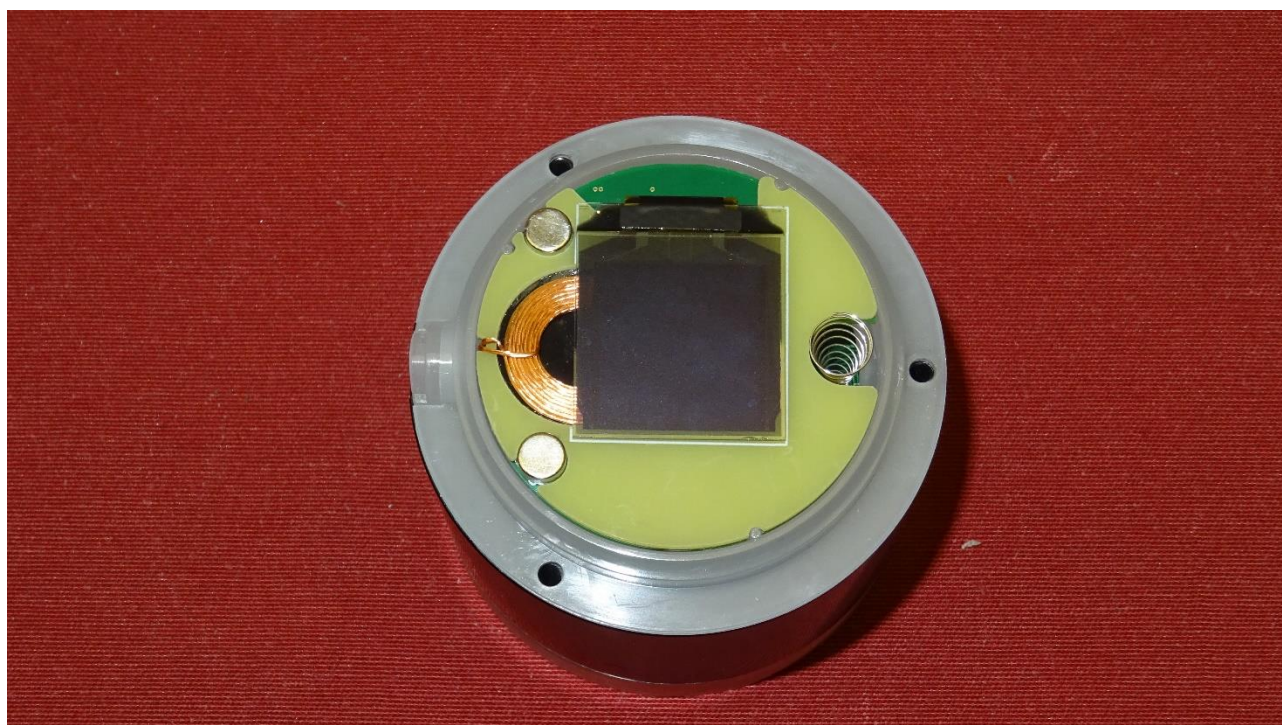
Picture 2: BLE probe – front view of PCB
