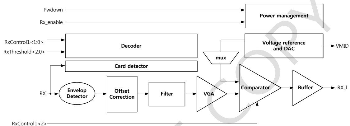
Picture 11-2 Receiver Structure
