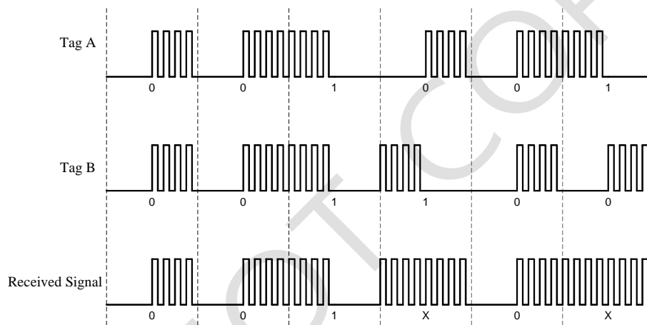
Picture 5-3 Collision Detection
