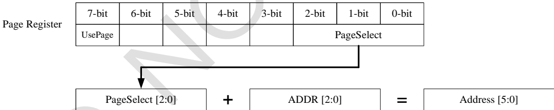
Picture 3-2 Dedicated Address Configuration
