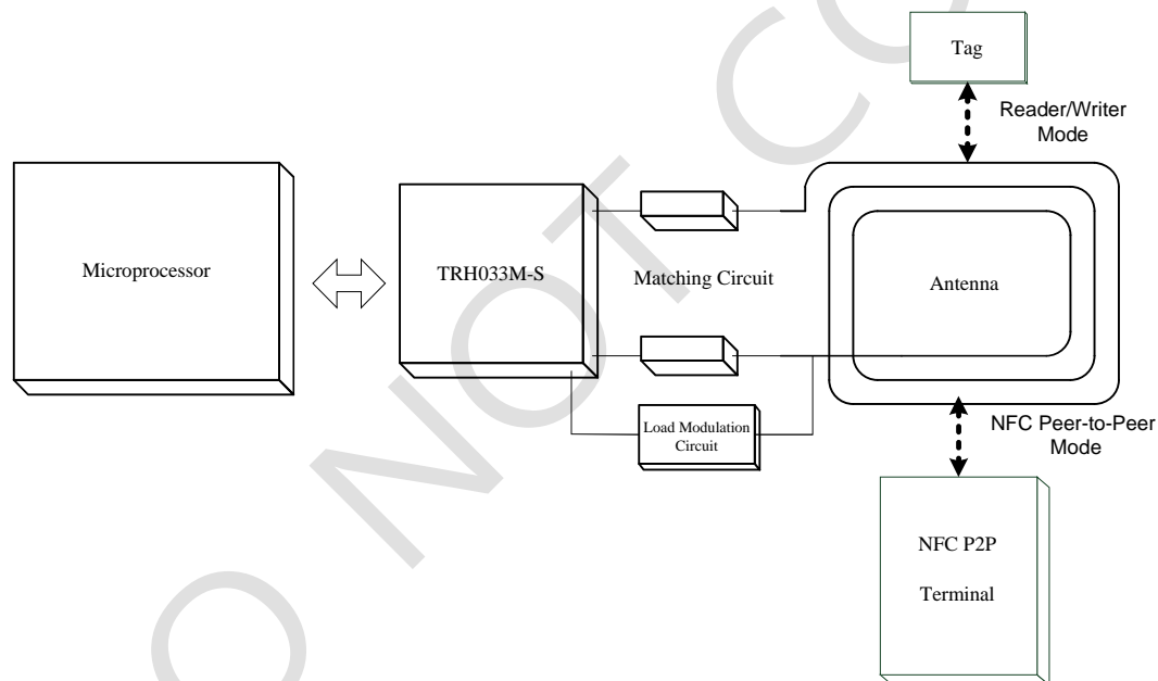
Picture 2-1 RFID Reader
