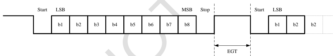
Picture 5-9 Length of EGT
