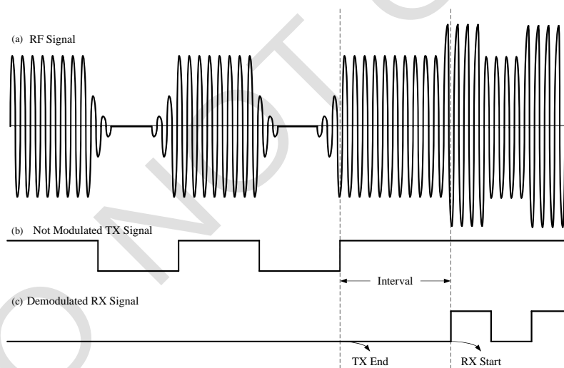
Picture 13-1 Observable signals by using test pin
