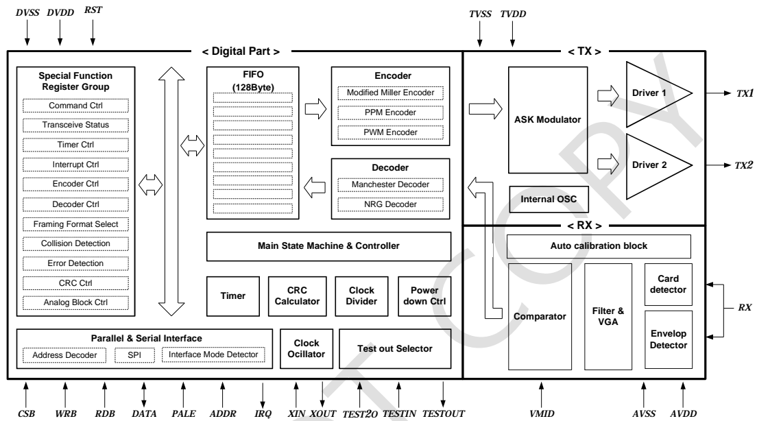
Picture 1-1 TRH033M-S Block Diagram
