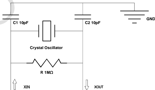
Picture 14-1 External Crystal Oscillator circuit
