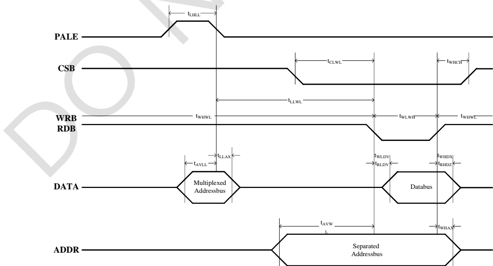
Picture 14-2 Timing for Separated Read/Write Strobe
