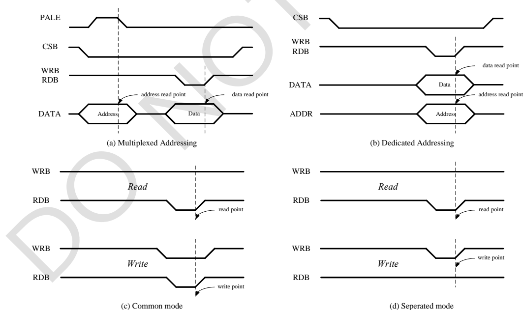
Picture 3-1 Shape of TRH033M-S supported microprocessor interface
