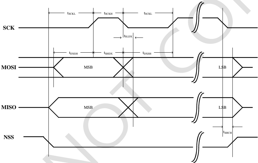
PICTURE 14-3 Timing for SPI compatible interface
