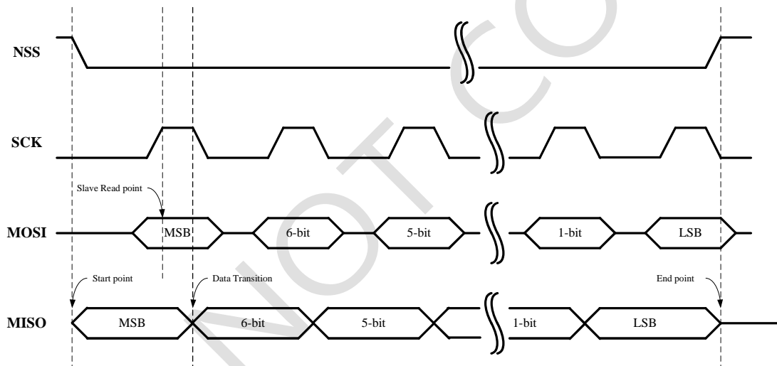
Picture 3-3 SPI Serial interface operation
