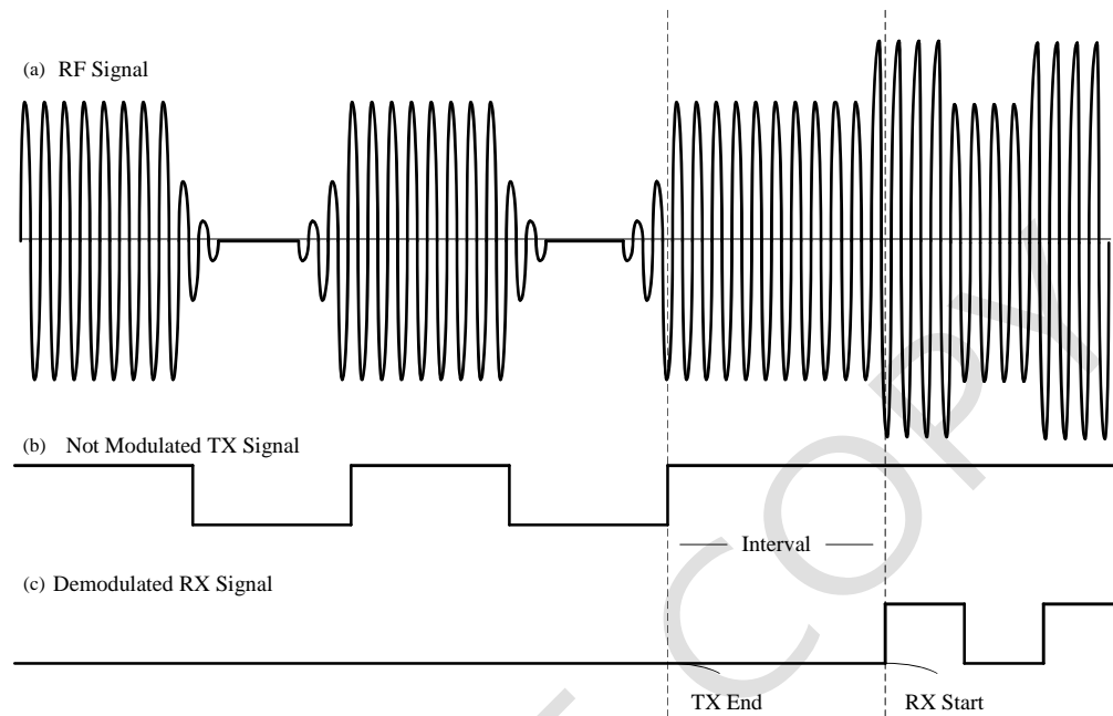
Picture 2-5 Status of Tx/Rx signal
