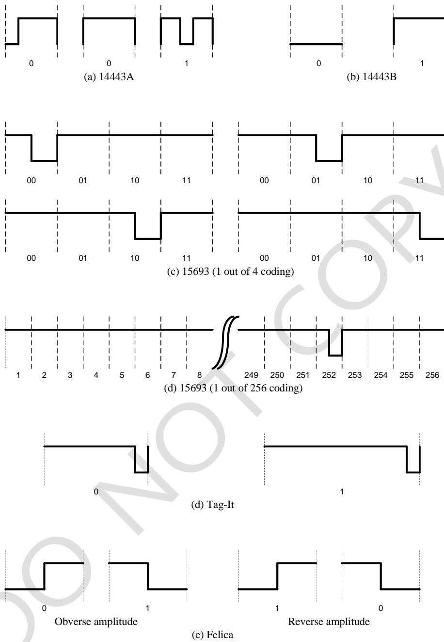
Picture 5-1 Encoding method by protocol
