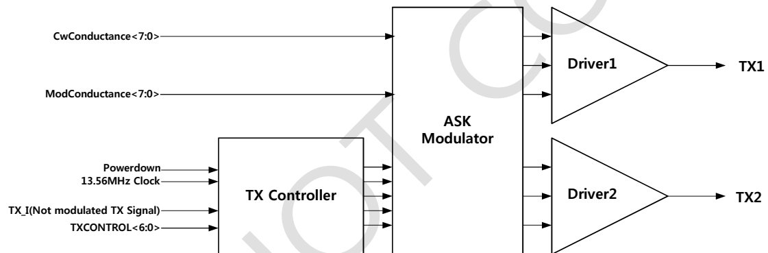
Picture 11-1 Transmitter Structure
