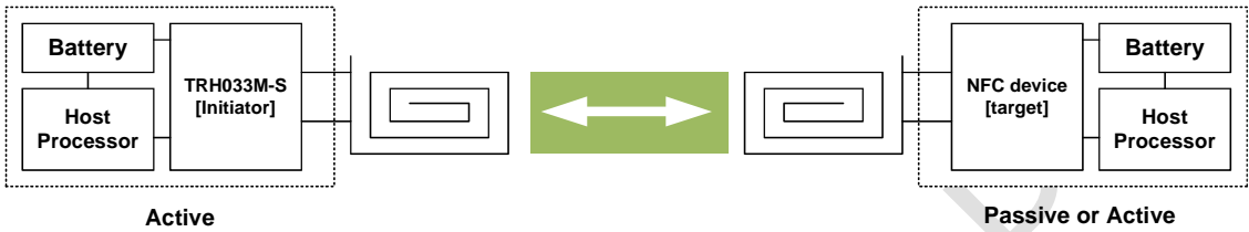
(a) TRH033M-S Active initiator mode
