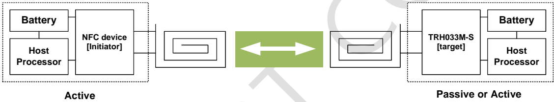
(b) TRH033M-S Active / Passive target mode
