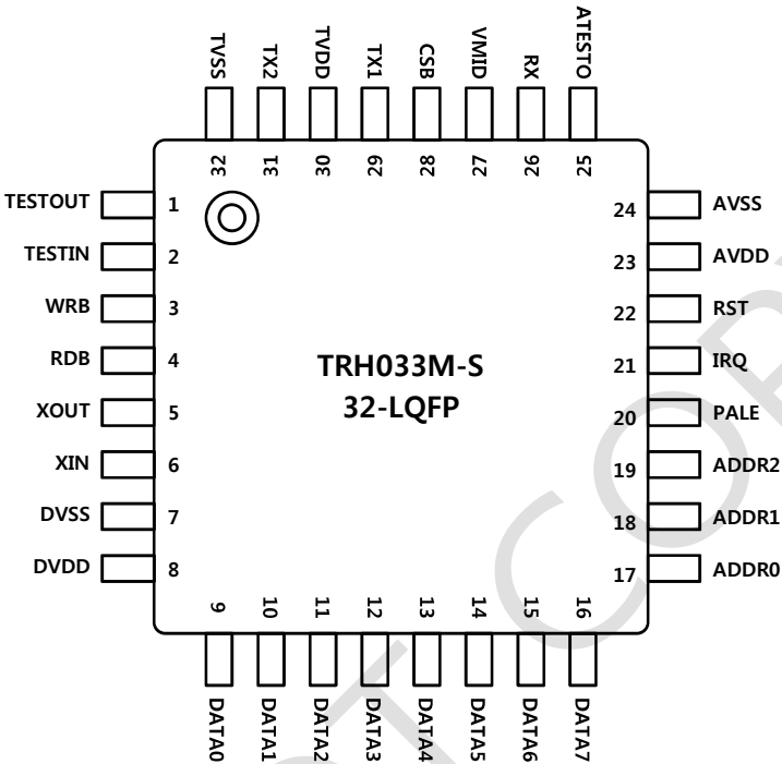
Picture 1-2 TRH033M-S Pin Diagrams
