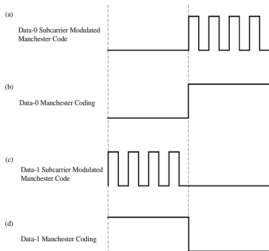
Picture 2-3 Encoding / Decoding
