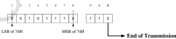
(c) Transmit Data (When TxLastBits = 2)
