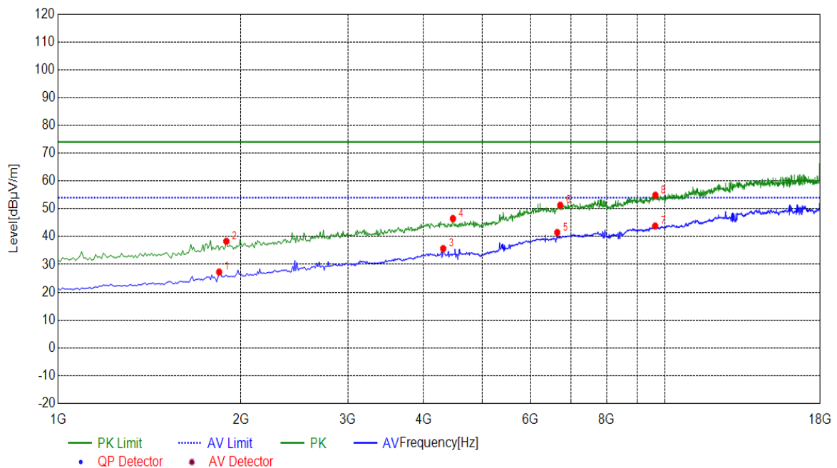
(Plot N: Test Antenna Vertical 1G – 18G)
