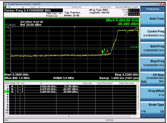
11AC40MIMO-Ant1-5510-PASS
