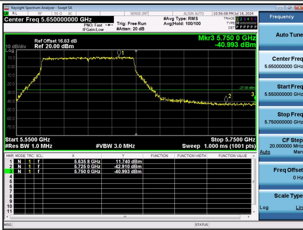
11AC80MIMO-Ant0-5610-PASS
