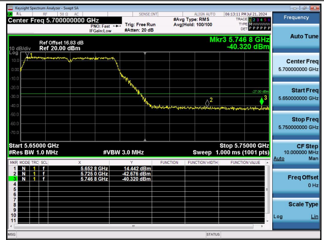
11N40MIMO-Ant1-5670-PASS
