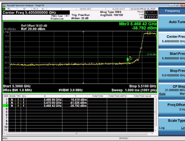
11N20MIMO-Ant0-5500-PASS
