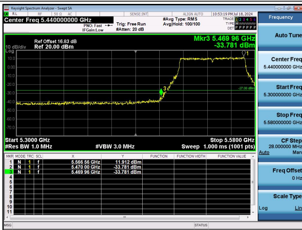
11AC80MIMO-Ant0-5530-PASS
