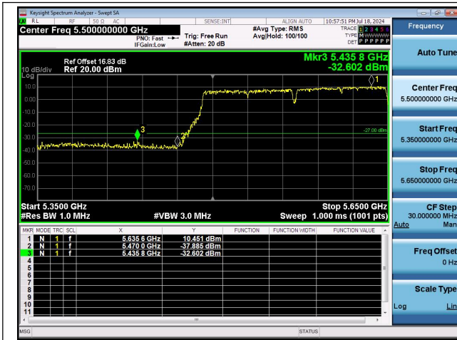
11AC160MIMO-Ant0-5570-PASS
