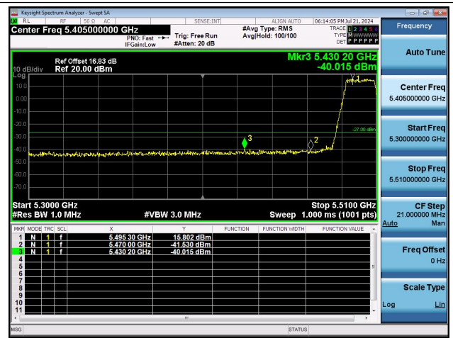
11AC20MIMO-Ant1-5500-PASS
