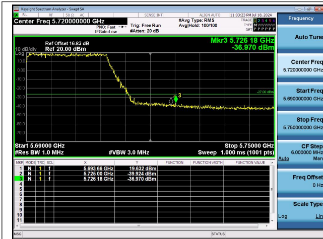
11AX20MIMO-Ant0-5700-PASS
