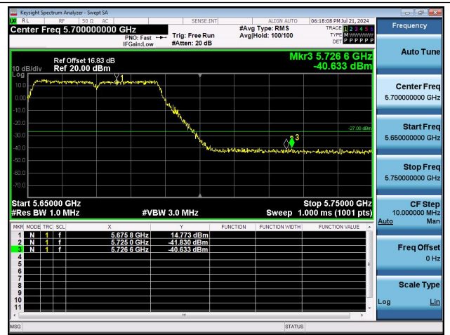
11AC40MIMO-Ant1-5670-PASS
