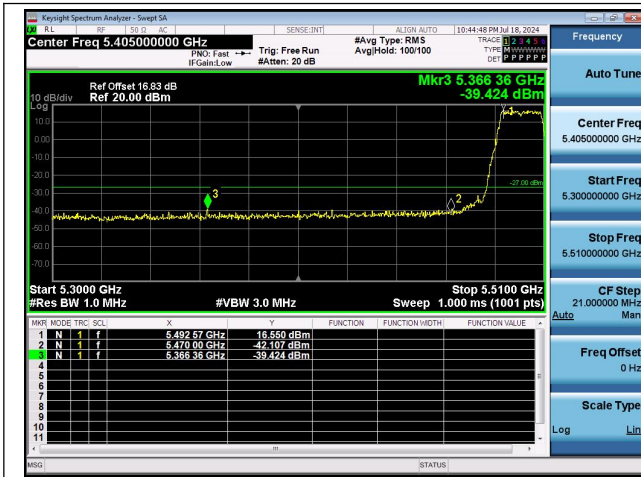
11AC20MIMO-Ant0-5500-PASS
