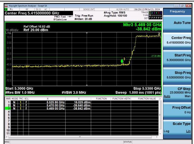
11AX40MIMO-Ant1-5510-PASS
