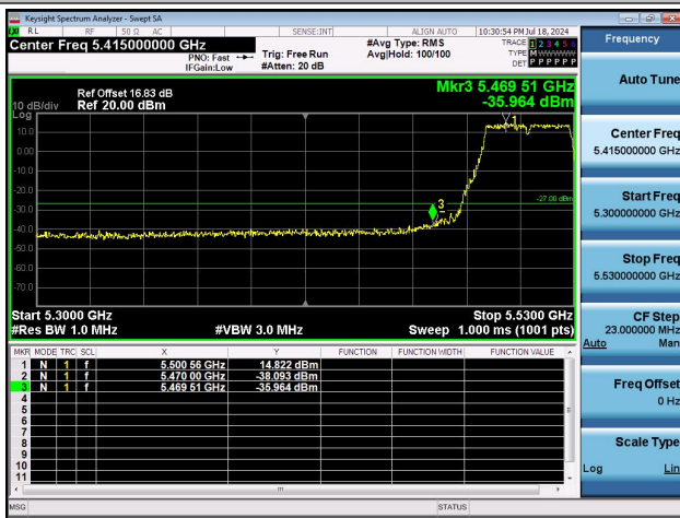
11N40MIMO-Ant0-5510-PASS
