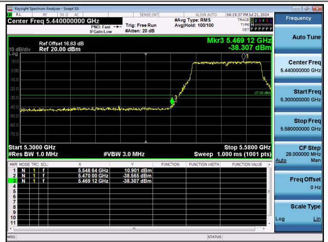
11AC80MIMO-Ant1-5530-PASS
