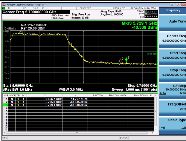
11N40MIMO-Ant0-5670-PASS
