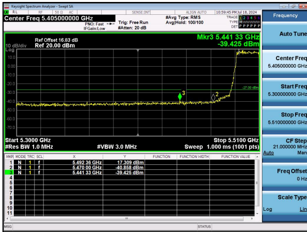
11AX20MIMO-Ant0-5500-PASS
