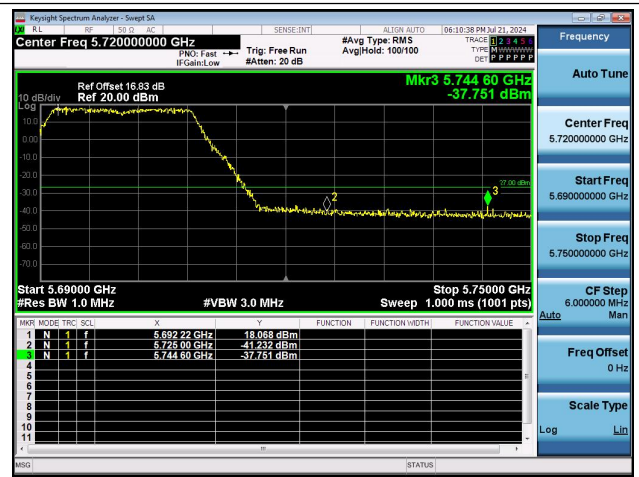
11N20MIMO-Ant1-5700-PASS
