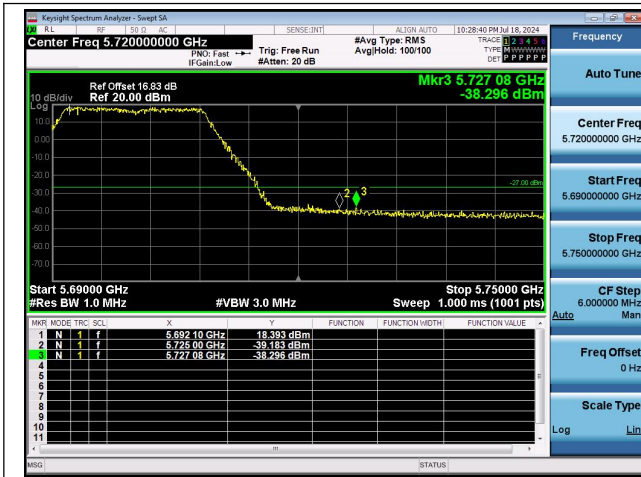
11N20MIMO-Ant0-5700-PASS
