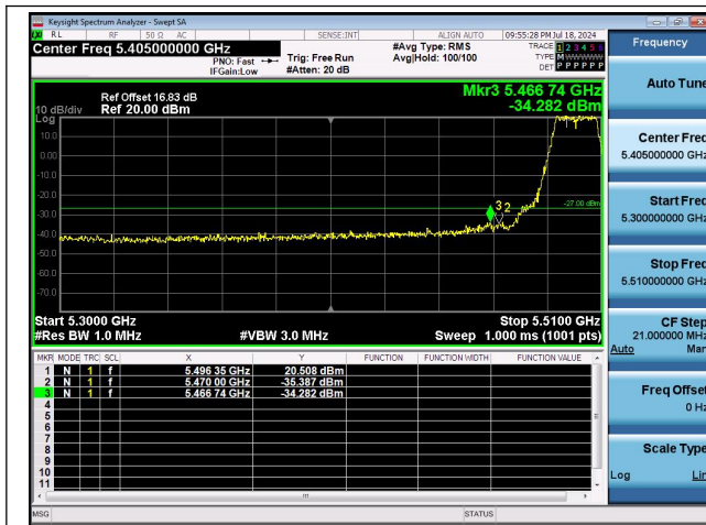
11A-Ant0-5500-PASS
