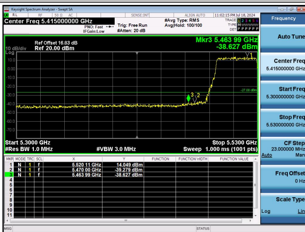
11AX40MIMO-Ant0-5510-PASS
