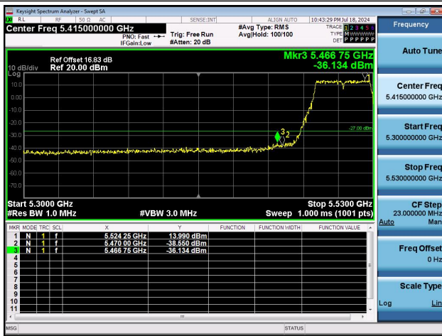
11AC40MIMO-Ant0-5510-PASS
