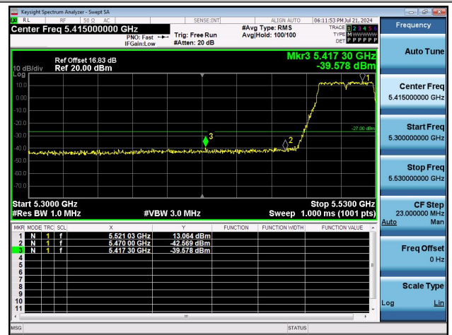
11N40MIMO-Ant1-5510-PASS
