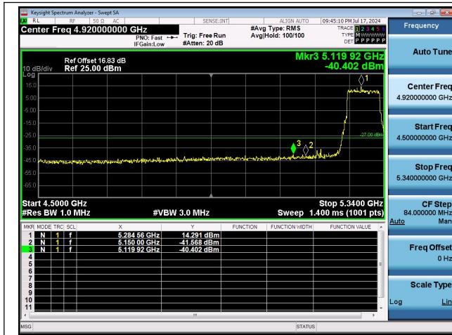
11AX80MIMO-Ant1-5290-PASS
