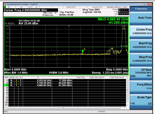
11AC20MIMO-Ant1-5320-PASS
