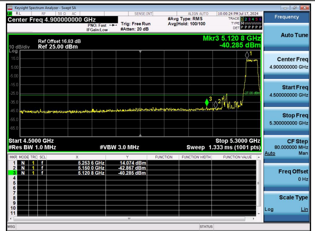
11AC40MIMO-Ant1-5310-PASS
