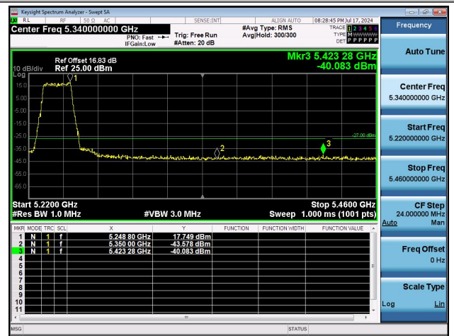
11AX20MIMO-Ant1-5240-PASS
