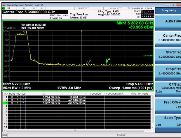
11AX20MIMO-Ant0-5240-PASS
