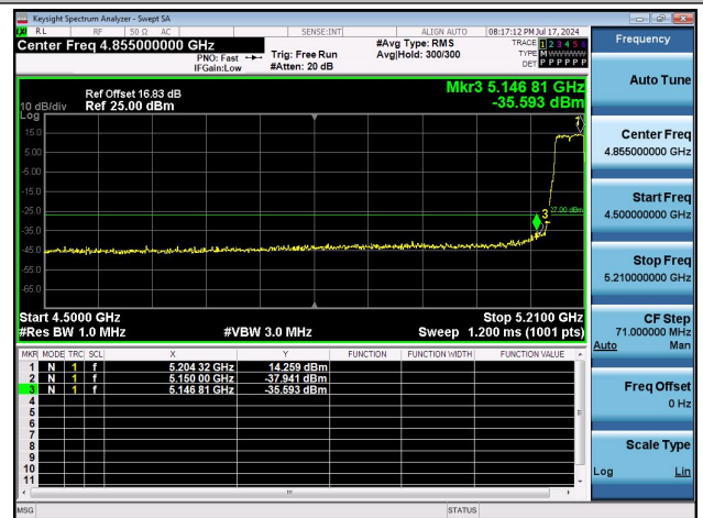
11N40MIMO-Ant1-5190-PASS
