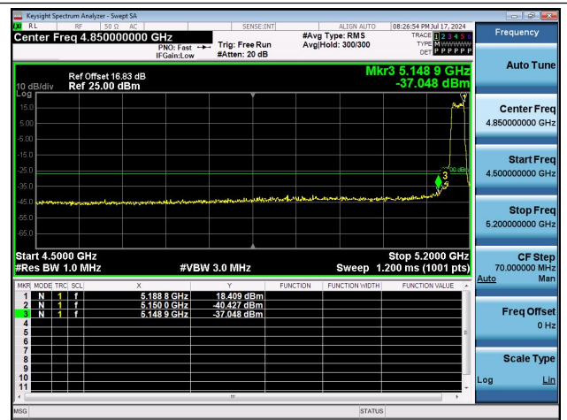
11AX20MIMO-Ant1-5180-PASS
