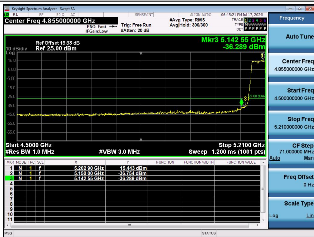
11N40MIMO-Ant0-5190-PASS
