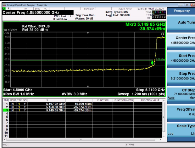
11AX40MIMO-Ant0-5190-PASS
