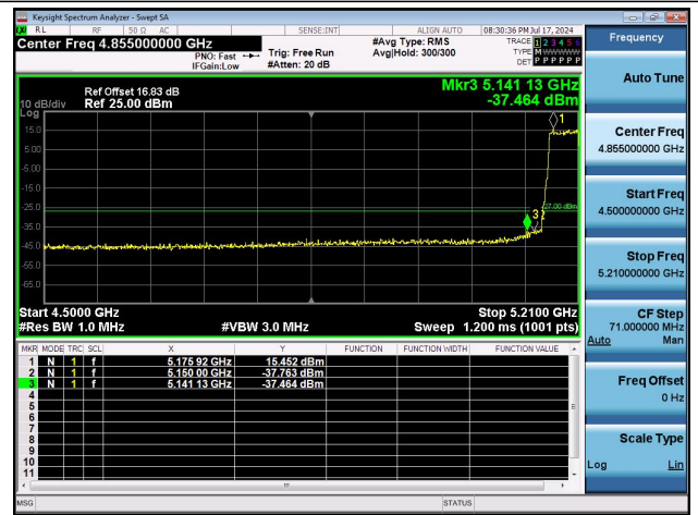
11AX40MIMO-Ant1-5190-PASS
