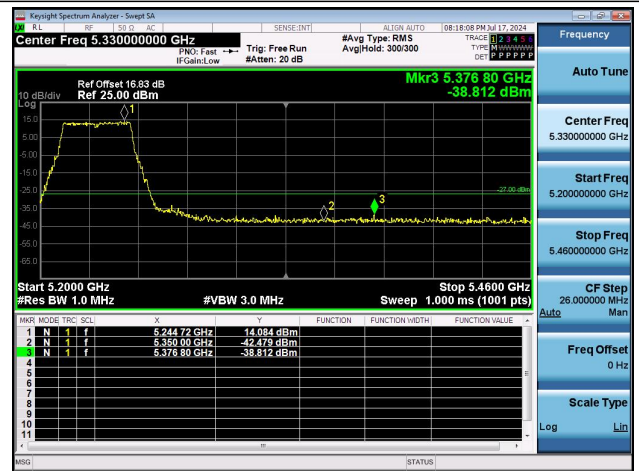
11N40MIMO-Ant1-5230-PASS
