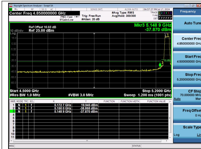
11AX20MIMO-Ant0-5180-PASS
