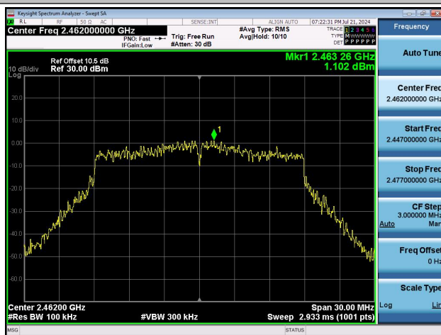
11N20MIMO-Ant0-2462-0~Reference-PASS
