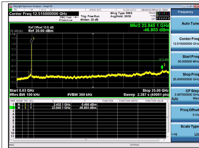
11N40MIMO-Ant0-2437-30~25000-PASS
