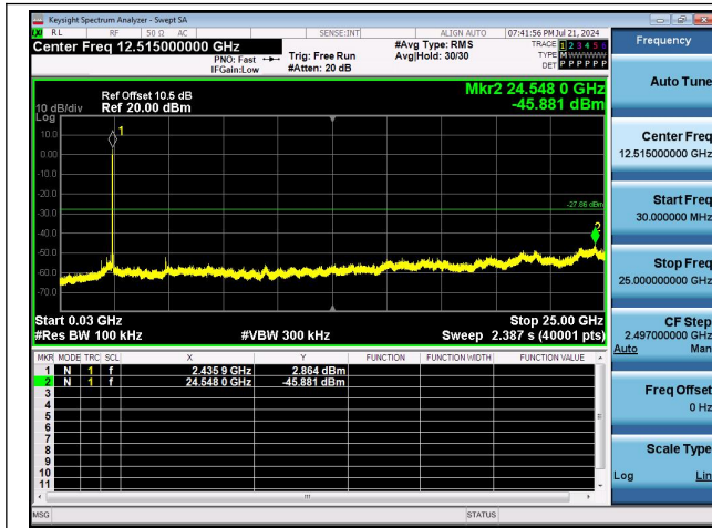
11AX20MIMO-Ant0-2437-30~25000-PASS
