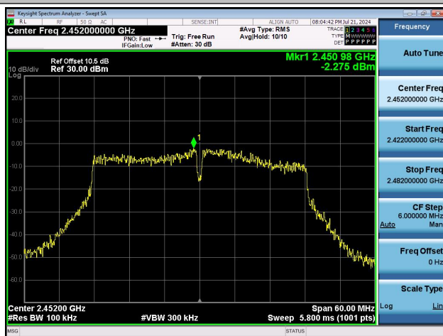
11N40MIMO-Ant0-2452-0~Reference-PASS
