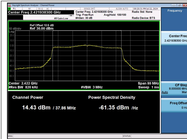
11AX40MIMO-Ant1-2422-PASS
