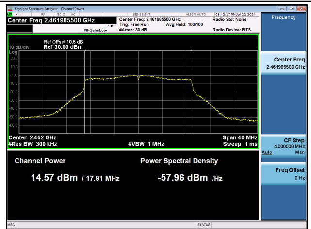
11N20MIMO-Ant1-2462-PASS
