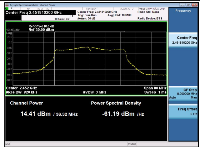
11N40MIMO-Ant0-2452-PASS
