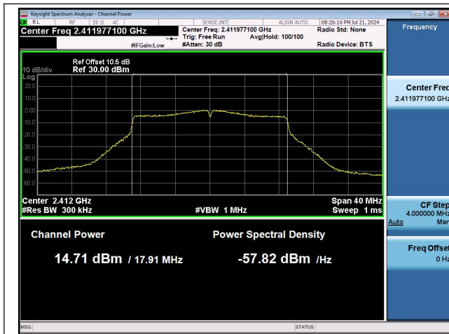
11N20MIMO-Ant0-2412-PASS
