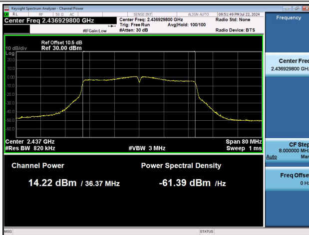
11N40MIMO-Ant1-2437-PASS
