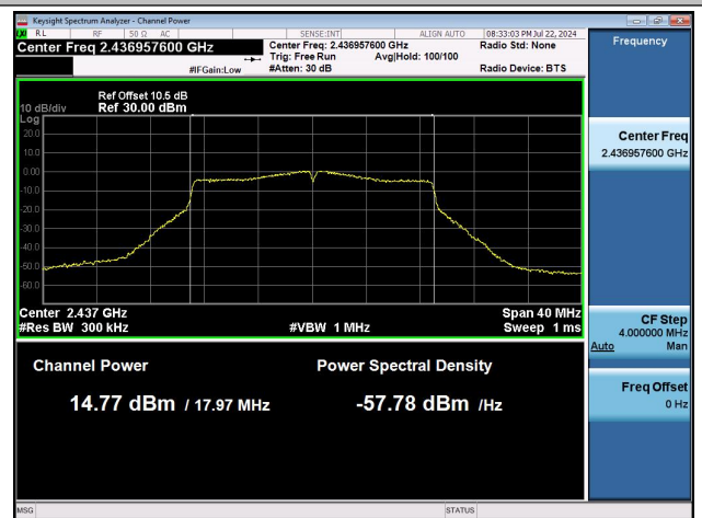
11N20MIMO-Ant1-2437-PASS
