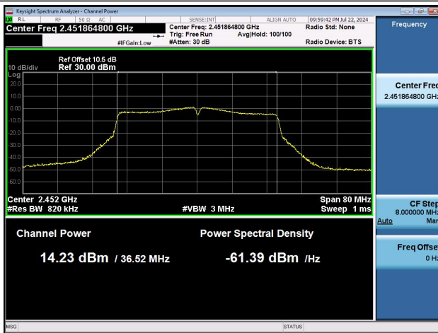
11N40MIMO-Ant1-2452-PASS
