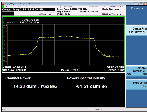
11AX40MIMO-Ant1-2452-PASS
