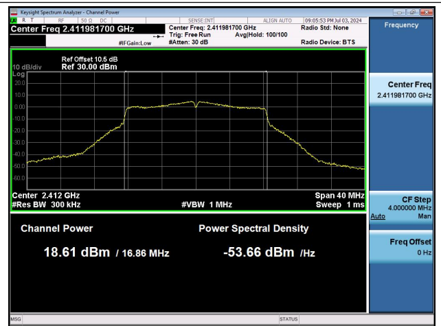
11G-Ant1-2412-PASS
