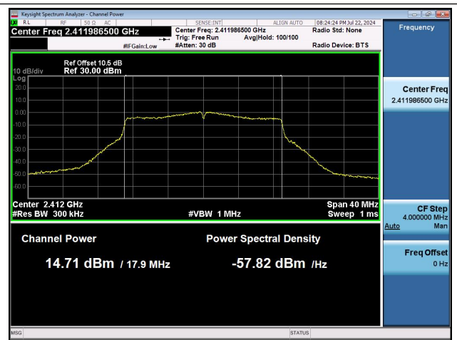
11N20MIMO-Ant1-2412-PASS
