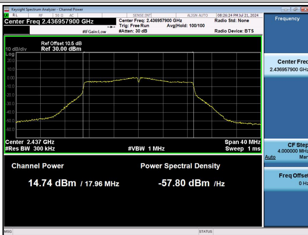
11N20MIMO-Ant0-2437-PASS
