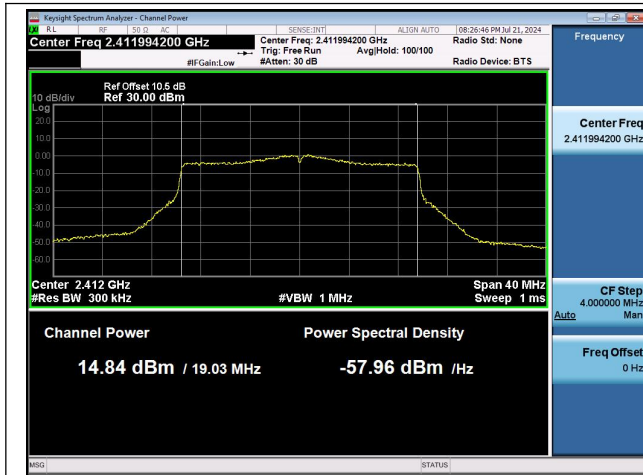
11AX20MIMO-Ant0-2412-PASS
