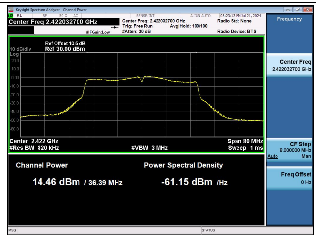
11N40MIMO-Ant0-2422-PASS
