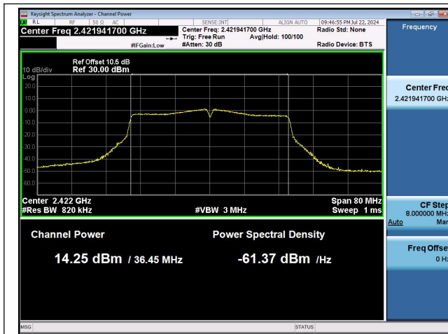
11N40MIMO-Ant1-2422-PASS
