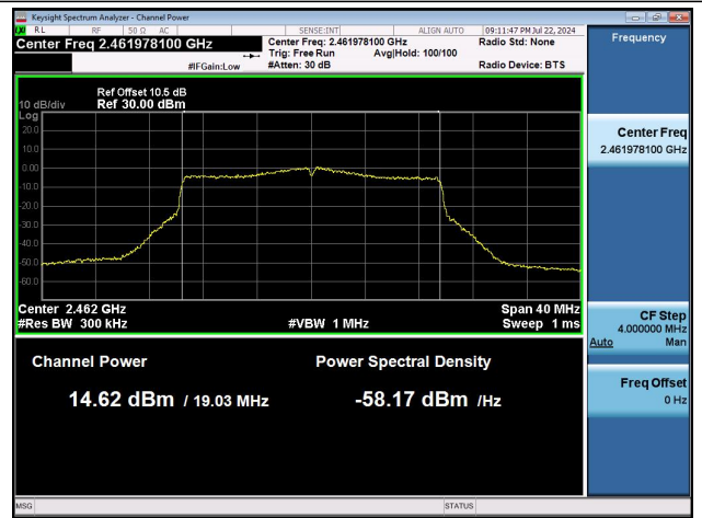
11AX20MIMO-Ant1-2462-PASS
