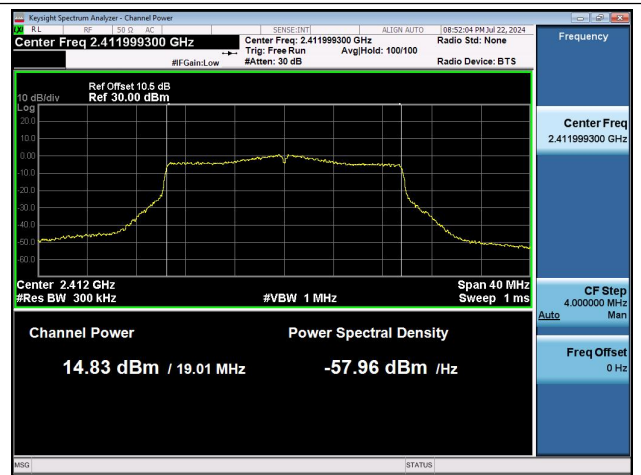
11AX20MIMO-Ant1-2412-PASS
