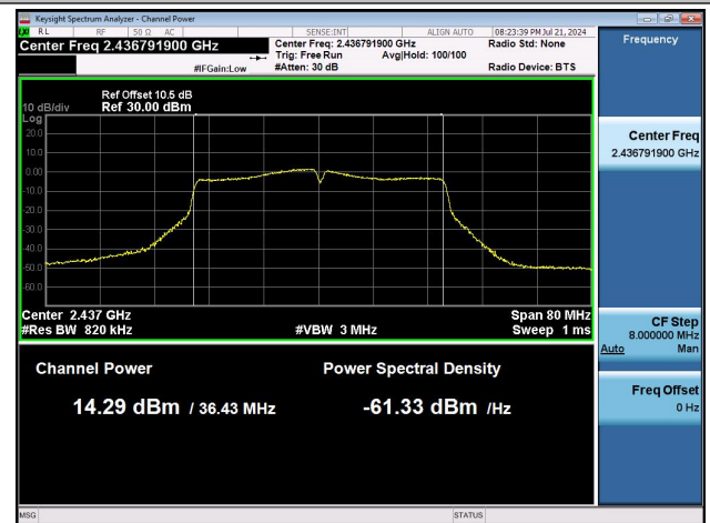
11N40MIMO-Ant0-2437-PASS
