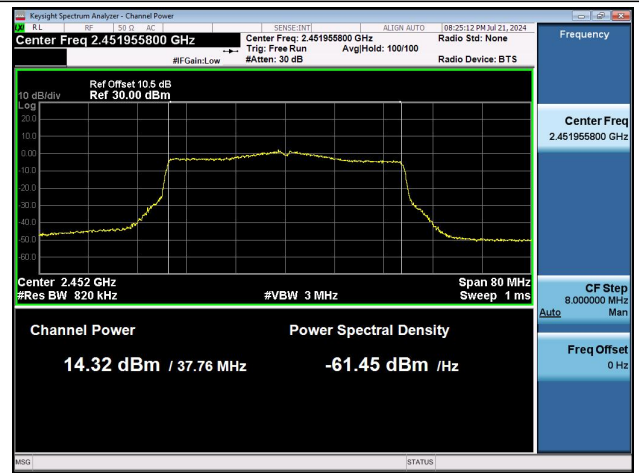
11AX40MIMO-Ant0-2452-PASS
