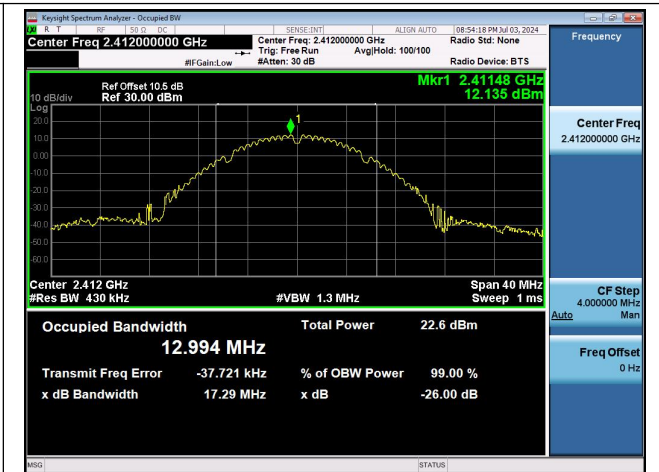
11B-Ant1-2412
