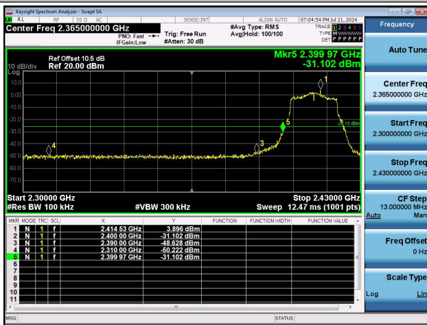
11N20MIMO-Ant0-2412-PASS
