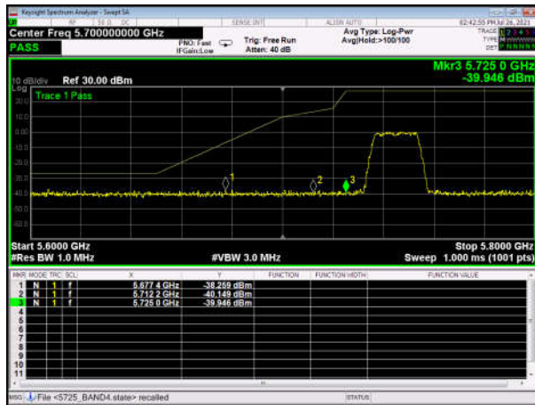
U-NII-3 ,Plot 1,Band Edge-802.11ac(20 MHz),5745MHz,Ant0
