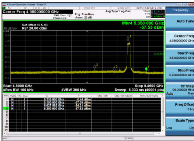
U-NII-1 ,Plot 1,Band Edge-802.11ax(40 MHz),5230MHz,Ant1
