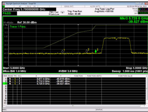
U-NII-3 ,Plot 1,Band Edge-802.11ac(80 MHz),5775MHz,Ant0 Left bandedge
