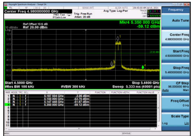
U-NII-1 ,Plot 1,Band Edge-802.11ax(80 MHz),5210MHz,Ant1
