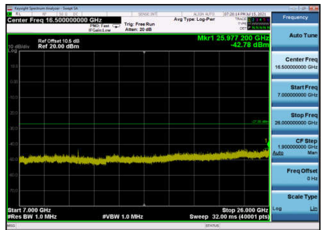
U-NII-3 ,Plot 4,7000MHz~26000MHz-802. 11a(20MHz),5745MHz,Ant0
