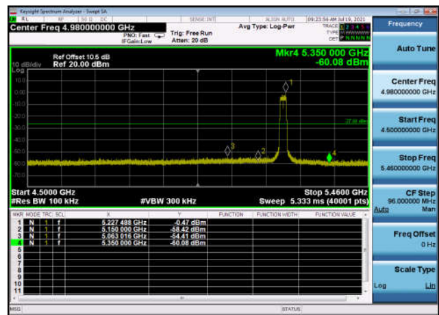
U-NII-1 ,Plot 1,Band Edge-802.11ax(20 MHz),5220MHz,Ant1
