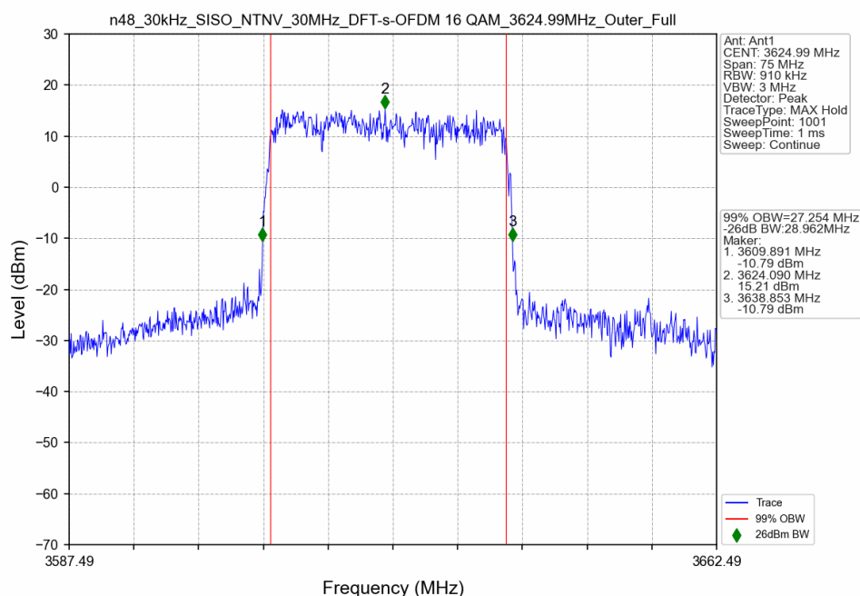
n48_30kHz_SISO_NTNV_30MHz_DFT-s-OFDM 16 QAM_3624.99MHz_Outer_Full
