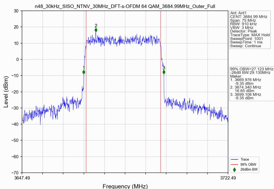
n48_30kHz_SISO_NTNV_30MHz_DFT-s-OFDM 64 QAM_3684.99MHz_Outer_Full
