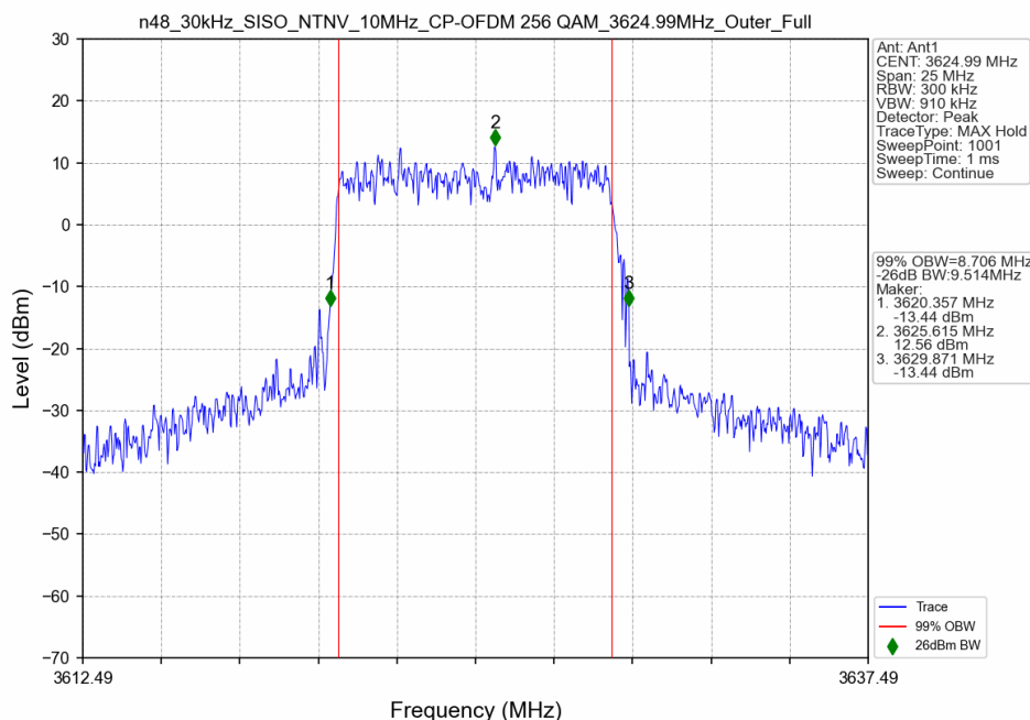
n48_30kHz_SISO_NTNV_10MHz_CP-OFDM 256 QAM_3624.99MHz_Outer_Full
