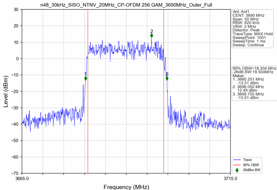
n48_30kHz_SISO_NTNV_20MHz_CP-OFDM 256 QAM_3690MHz_Outer_Full
