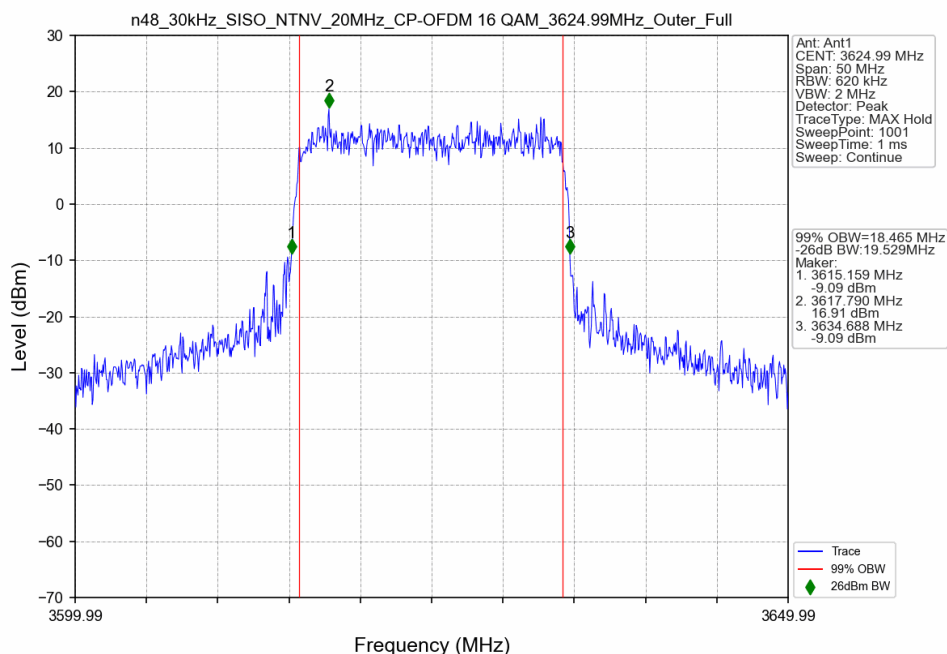
n48_30kHz_SISO_NTNV_20MHz_CP-OFDM 16 QAM_3624.99MHz_Outer_Full
