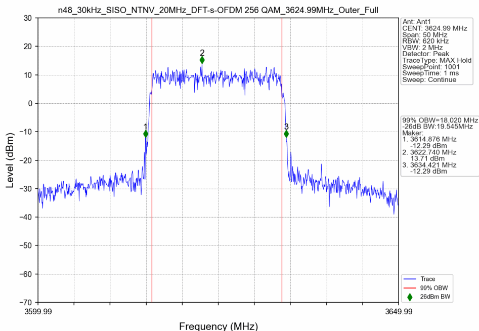
n48_30kHz_SISO_NTNV_20MHz_DFT-s-OFDM 256 QAM_3624.99MHz_Outer_Full
