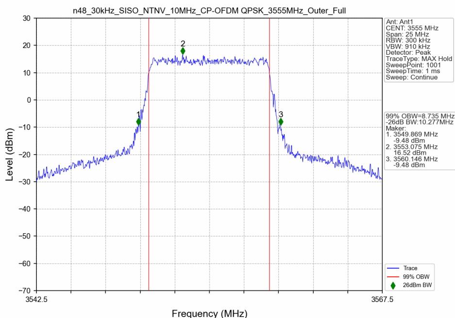
n48_30kHz_SISO_NTNV_10MHz_CP-OFDM QPSK_3555MHz_Outer_Full
