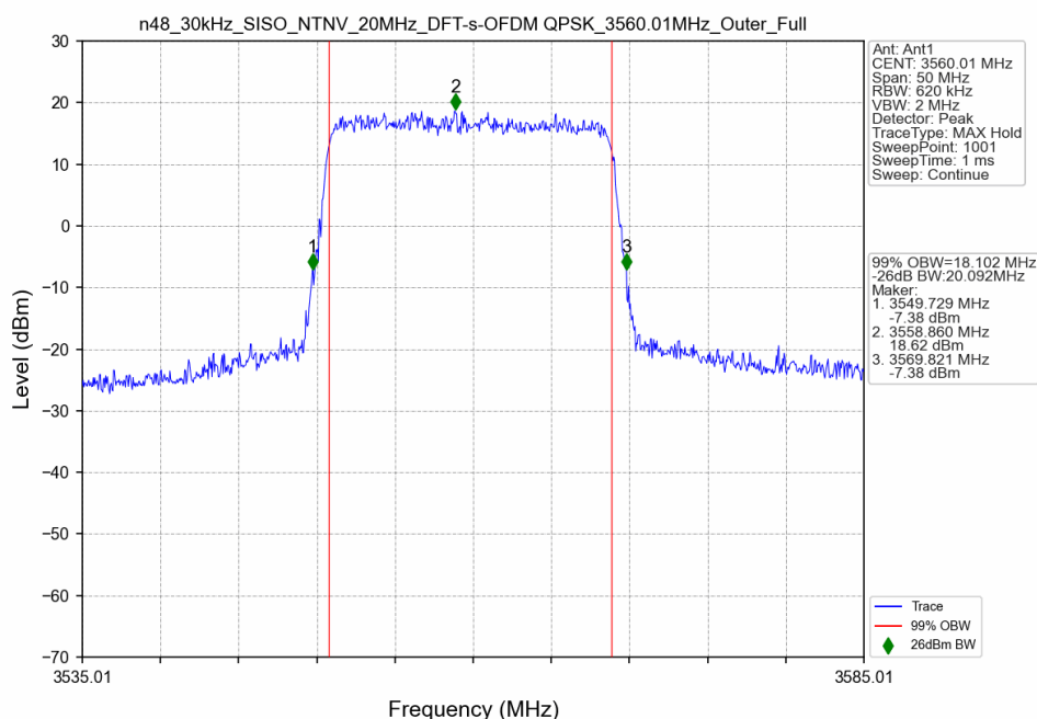
n48_30kHz_SISO_NTNV_20MHz_DFT-s-OFDM QPSK_3560.01MHz_Outer_Full
