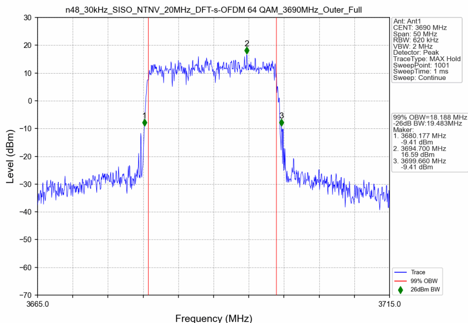
n48_30kHz_SISO_NTNV_20MHz_DFT-s-OFDM 64 QAM_3690MHz_Outer_Full
