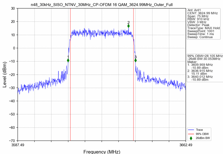
n48_30kHz_SISO_NTNV_30MHz_CP-OFDM 16 QAM_3624.99MHz_Outer_Full
