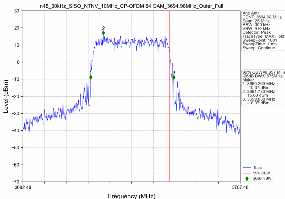
n48_30kHz_SISO_NTNV_10MHz_CP-OFDM 64 QAM_3694.98MHz_Outer_Full
