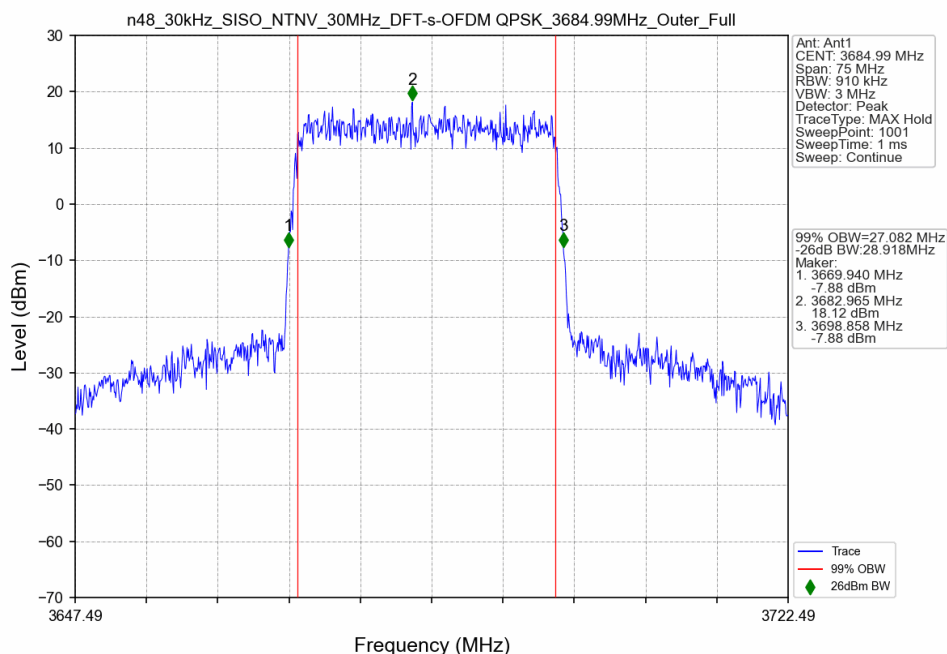
n48_30kHz_SISO_NTNV_30MHz_DFT-s-OFDM QPSK_3684.99MHz_Outer_Full
