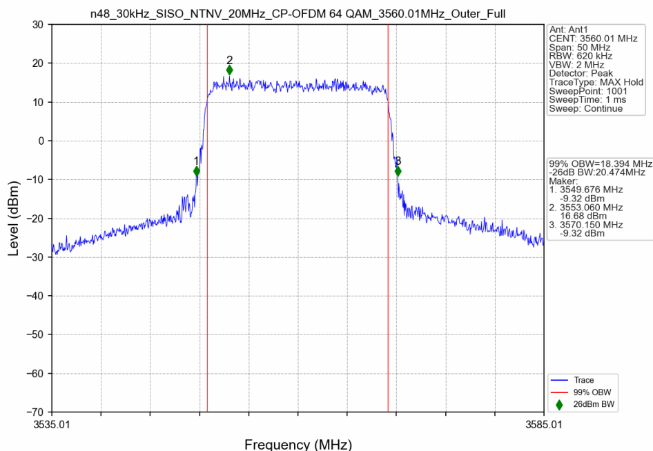
n48_30kHz_SISO_NTNV_20MHz_CP-OFDM 64 QAM_3560.01MHz_Outer_Full
