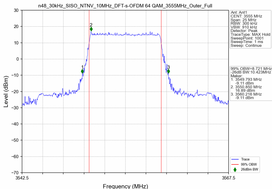
n48_30kHz_SISO_NTNV_10MHz_DFT-s-OFDM 64 QAM_3555MHz_Outer_Full
