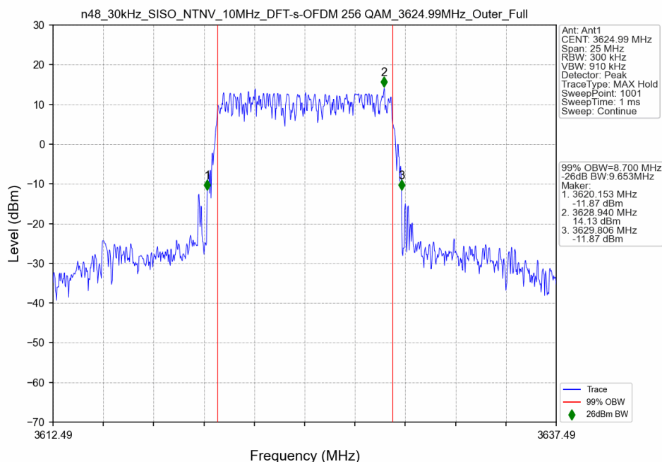
n48_30kHz_SISO_NTNV_10MHz_DFT-s-OFDM 256 QAM_3624.99MHz_Outer_Full
