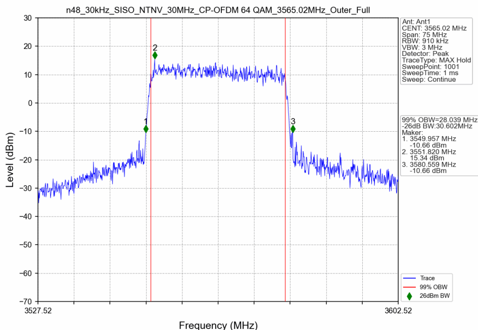
n48_30kHz_SISO_NTNV_30MHz_CP-OFDM 64 QAM_3565.02MHz_Outer_Full
