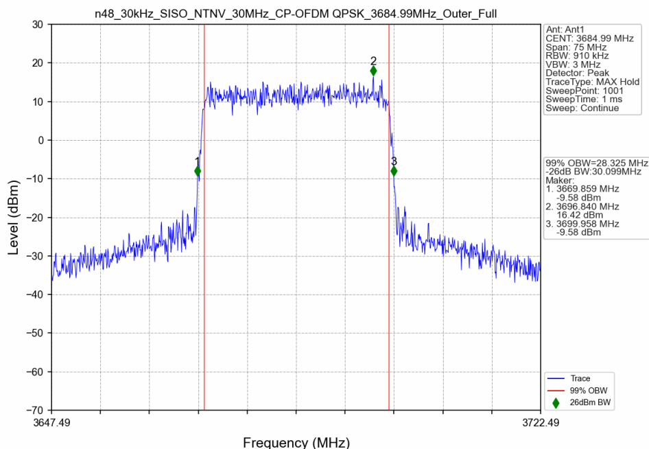
n48_30kHz_SISO_NTNV_30MHz_CP-OFDM QPSK_3684.99MHz_Outer_Full
