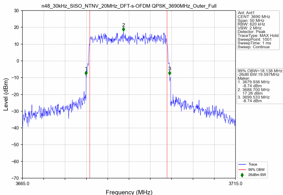
n48_30kHz_SISO_NTNV_20MHz_DFT-s-OFDM QPSK_3690MHz_Outer_Full
