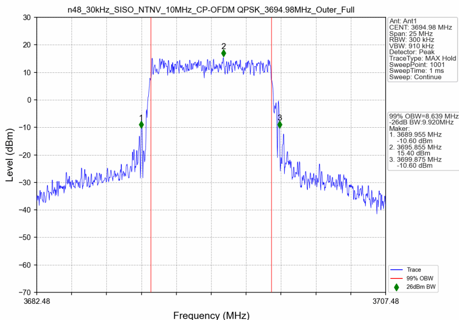
n48_30kHz_SISO_NTNV_10MHz_CP-OFDM QPSK_3694.98MHz_Outer_Full
