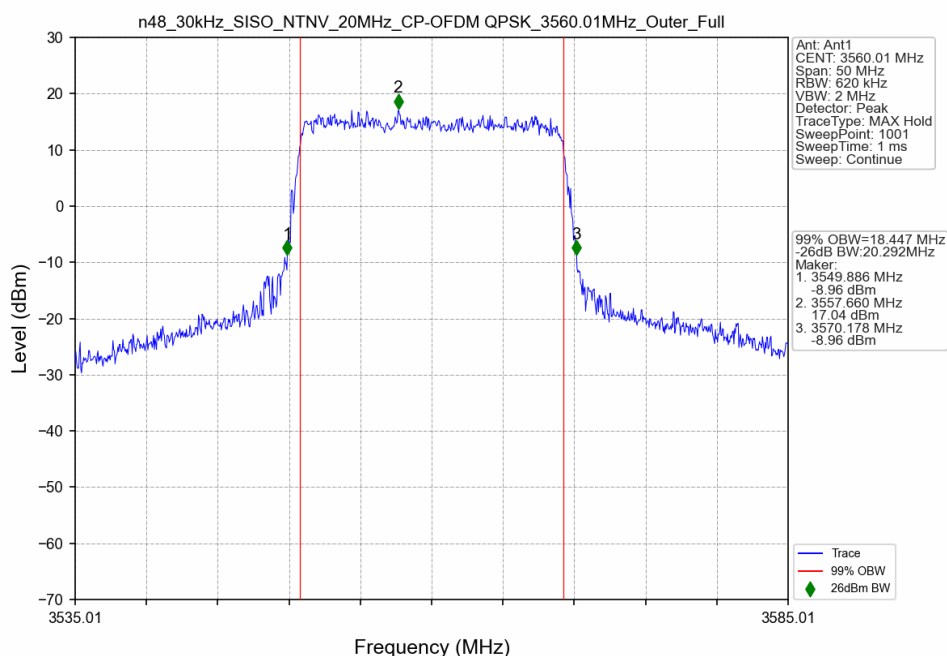
n48_30kHz_SISO_NTNV_20MHz_CP-OFDM QPSK_3560.01MHz_Outer_Full
