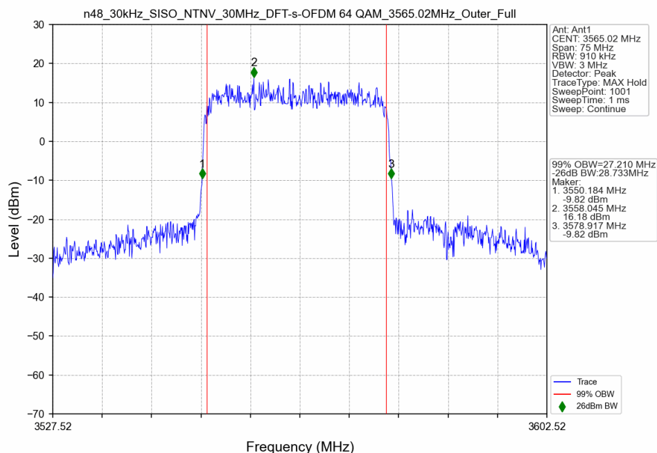
n48_30kHz_SISO_NTNV_30MHz_DFT-s-OFDM 64 QAM_3565.02MHz_Outer_Full
