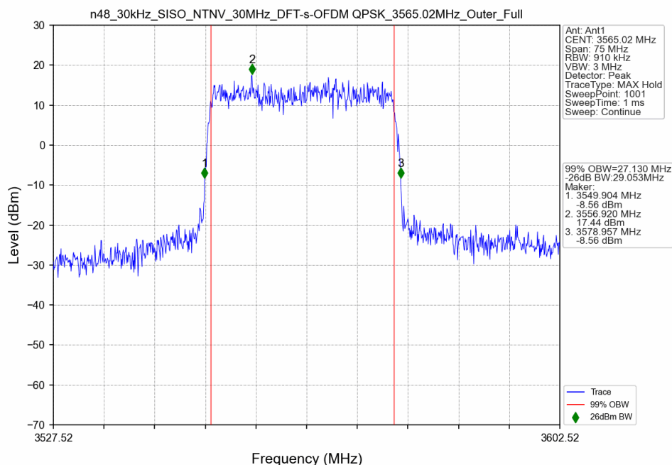
n48_30kHz_SISO_NTNV_30MHz_DFT-s-OFDM QPSK_3565.02MHz_Outer_Full
