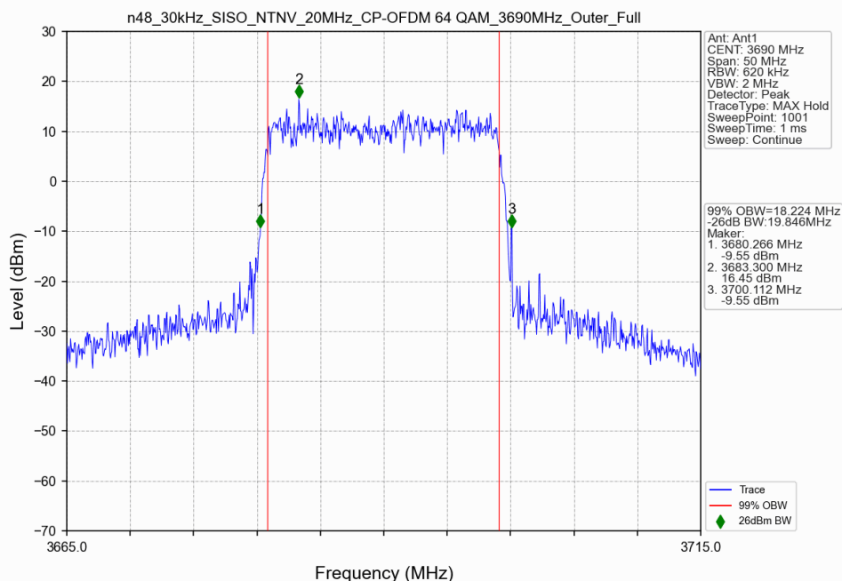
n48_30kHz_SISO_NTNV_20MHz_CP-OFDM 64 QAM_3690MHz_Outer_Full
