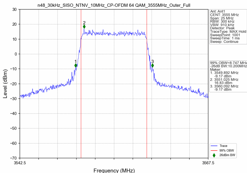
n48_30kHz_SISO_NTNV_10MHz_CP-OFDM 64 QAM_3555MHz_Outer_Full
