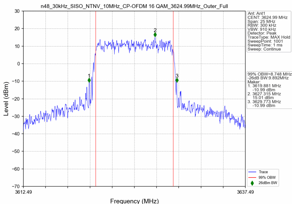
n48_30kHz_SISO_NTNV_10MHz_CP-OFDM 16 QAM_3624.99MHz_Outer_Full
