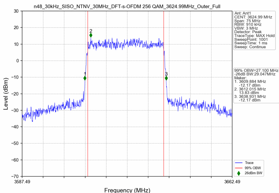
n48_30kHz_SISO_NTNV_30MHz_DFT-s-OFDM 256 QAM_3624.99MHz_Outer_Full
