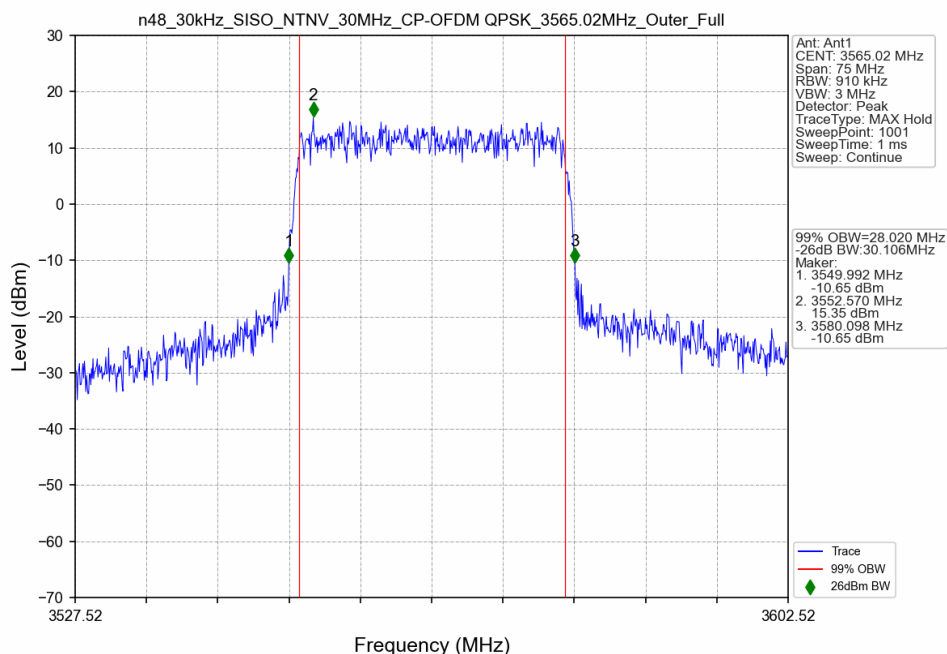
n48_30kHz_SISO_NTNV_30MHz_CP-OFDM QPSK_3565.02MHz_Outer_Full
