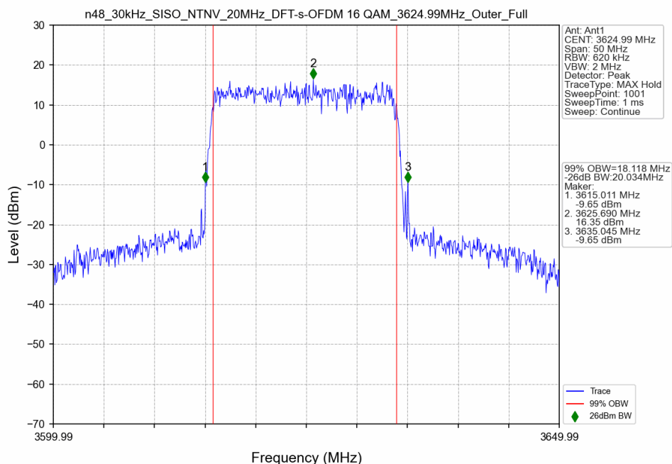
n48_30kHz_SISO_NTNV_20MHz_DFT-s-OFDM 16 QAM_3624.99MHz_Outer_Full
