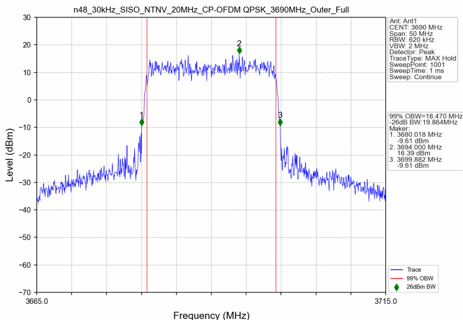
n48_30kHz_SISO_NTNV_20MHz_CP-OFDM QPSK_3690MHz_Outer_Full
