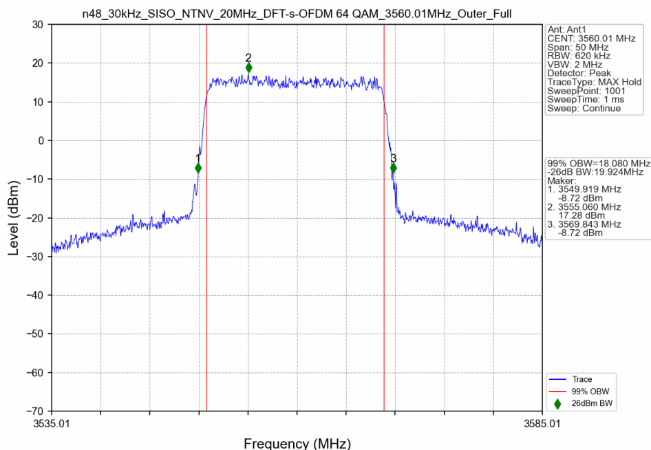
n48_30kHz_SISO_NTNV_20MHz_DFT-s-OFDM 64 QAM_3560.01MHz_Outer_Full
