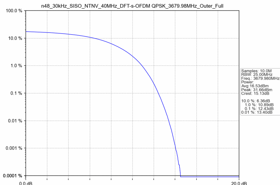
n48_30kHz_SISO_NTNV_40MHz_DFT-s-OFDM QPSK_3679.98MHz_Outer_Full
