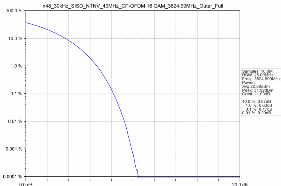
n48_30kHz_SISO_NTNV_40MHz_CP-OFDM 16 QAM_3624.99MHz_Outer_Full
