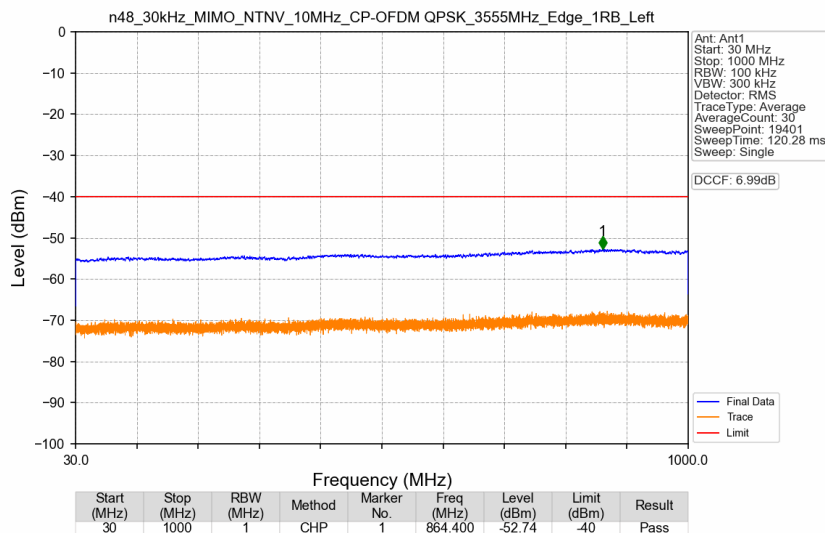
n48_30kHz_MIMO_NTNV_10MHz_CP-OFDM QPSK_3555MHz_Edge_1RB_Left
