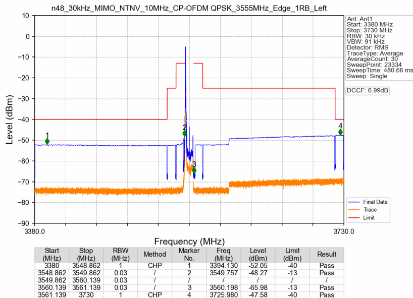
n48_30kHz_MIMO_NTNV_10MHz_CP-OFDM QPSK_3555MHz_Edge_1RB_Left
