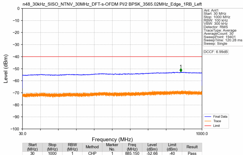
n48_30kHz_SISO_NTNV_30MHz_DFT-s-OFDM PI/2 BPSK_3565.02MHz_Edge_1RB_Left
