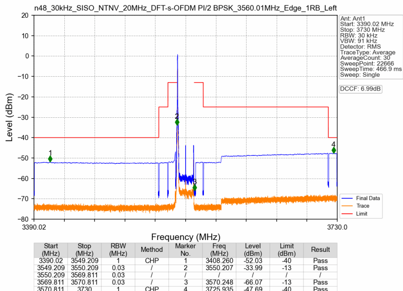
n48_30kHz_SISO_NTNV_20MHz_DFT-s-OFDM PI/2 BPSK_3560.01MHz_Edge_1RB_Left
