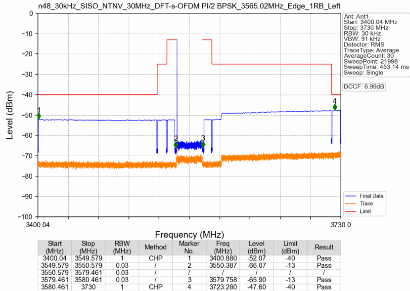
n48_30kHz_SISO_NTNV_30MHz_DFT-s-OFDM PI/2 BPSK_3565.02MHz_Edge_1RB_Left
