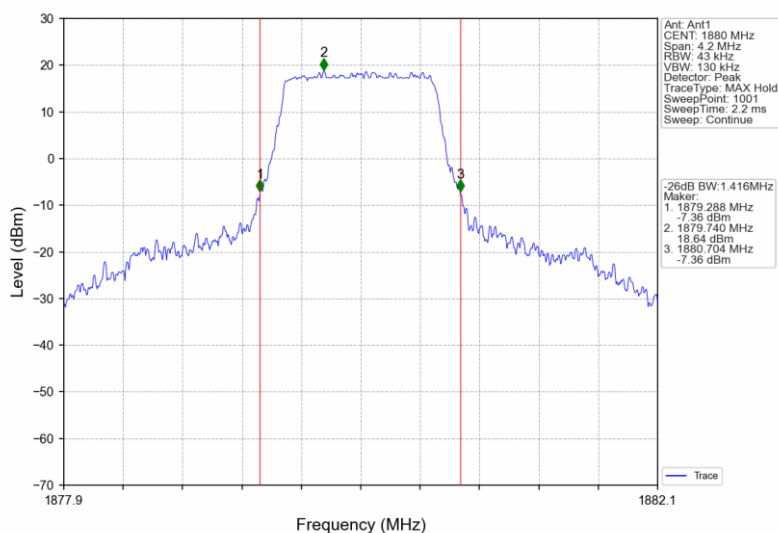
Band2_1.4MHz_QPSK_MCH_1880MHz_RB_6_0_NTNV
