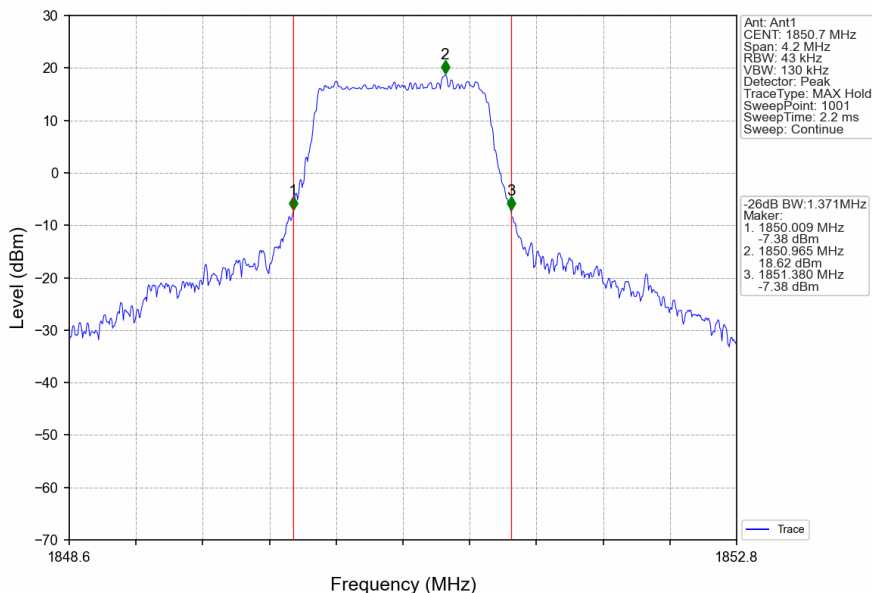
Band2_1.4MHz_16QAM_LCH_1850.7MHz_RB_6_0_NTNV
