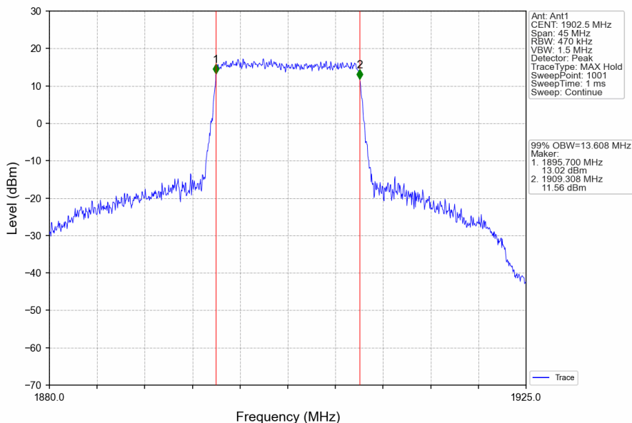
Band2_15MHz_16QAM_HCH_1902.5MHz_RB_75_0_NTNV
