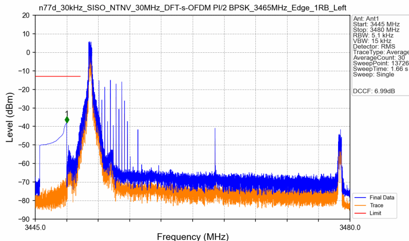
n77d_30kHz_SISO_NTNV_30MHz_DFT-s-OFDM PI/2 BPSK_3465MHz_Edge_1RB_Left
