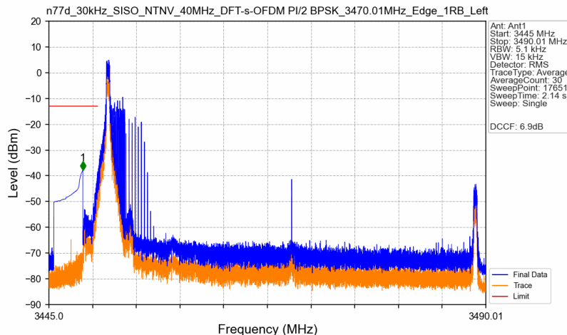
n77d_30kHz_SISO_NTNV_40MHz_DFT-s-OFDM PI/2 BPSK_3470.01MHz_Edge_1RB_Left
