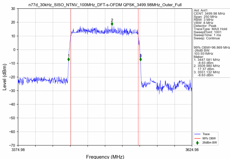
n77d_30kHz_SISO_NTNV_100MHz_DFT-s-OFDM QPSK_3499.98MHz_Outer_Full
