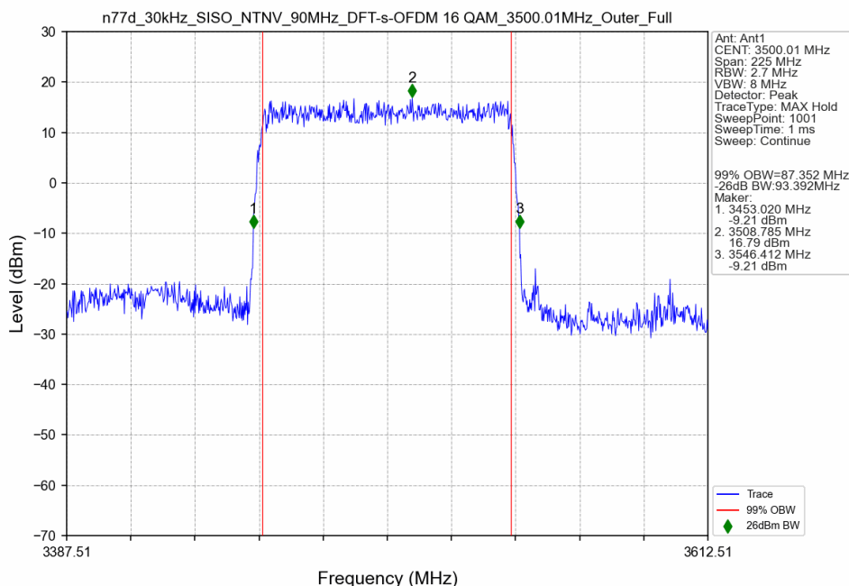
n77d_30kHz_SISO_NTNV_90MHz_DFT-s-OFDM 16 QAM_3500.01MHz_Outer_Full
