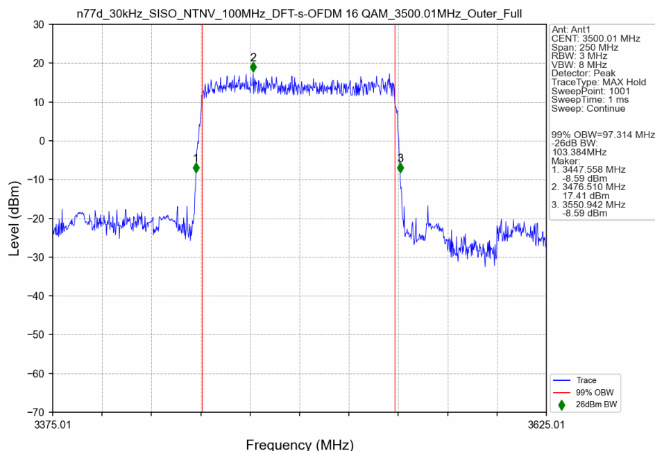
n77d_30kHz_SISO_NTNV_100MHz_DFT-s-OFDM 16 QAM_3500.01MHz_Outer_Full
