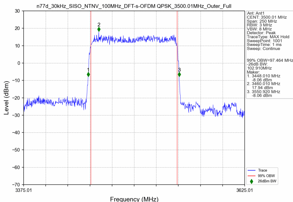
n77d_30kHz_SISO_NTNV_100MHz_DFT-s-OFDM QPSK_3500.01MHz_Outer_Full
