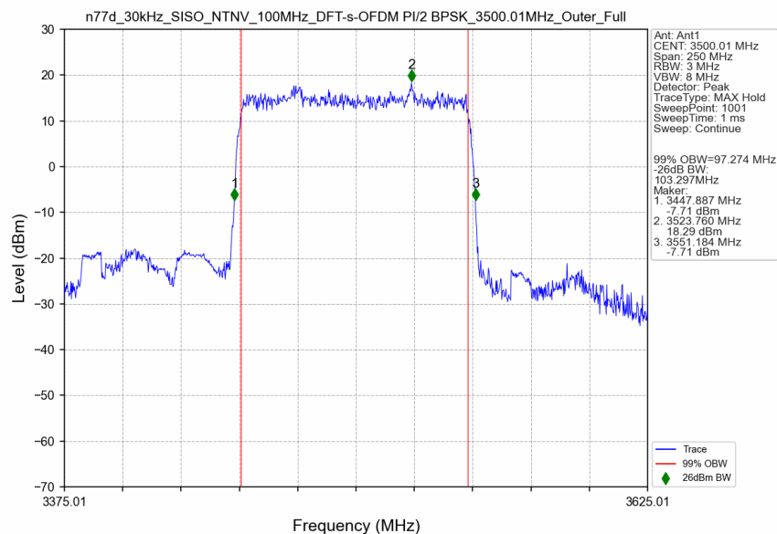
n77d_30kHz_SISO_NTNV_100MHz_DFT-s-OFDM PI/2 BPSK_3500.01MHz_Outer_Full
