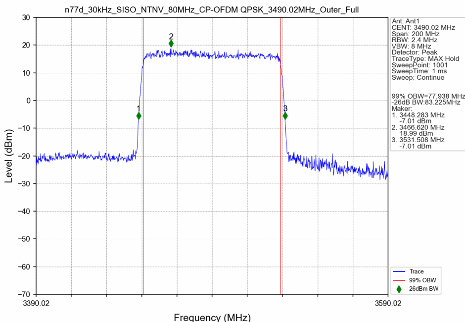
n77d_30kHz_SISO_NTNV_80MHz_CP-OFDM QPSK_3490.02MHz_Outer_Full
