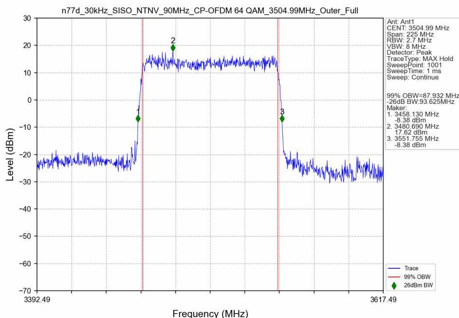
n77d_30kHz_SISO_NTNV_90MHz_CP-OFDM 64 QAM_3504.99MHz_Outer_Full
