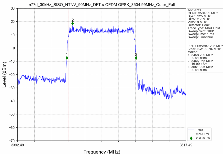
n77d_30kHz_SISO_NTNV_90MHz_DFT-s-OFDM QPSK_3504.99MHz_Outer_Full
