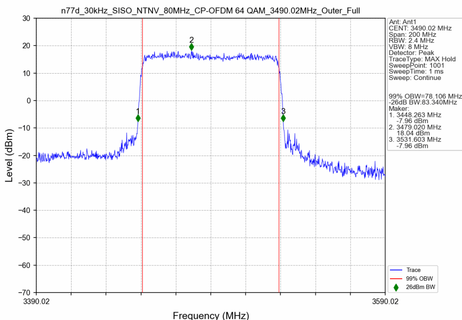
n77d_30kHz_SISO_NTNV_80MHz_CP-OFDM 64 QAM_3490.02MHz_Outer_Full
