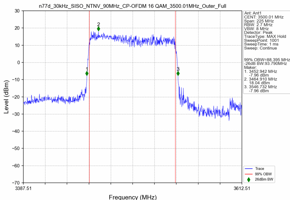
n77d_30kHz_SISO_NTNV_90MHz_CP-OFDM 16 QAM_3500.01MHz_Outer_Full
