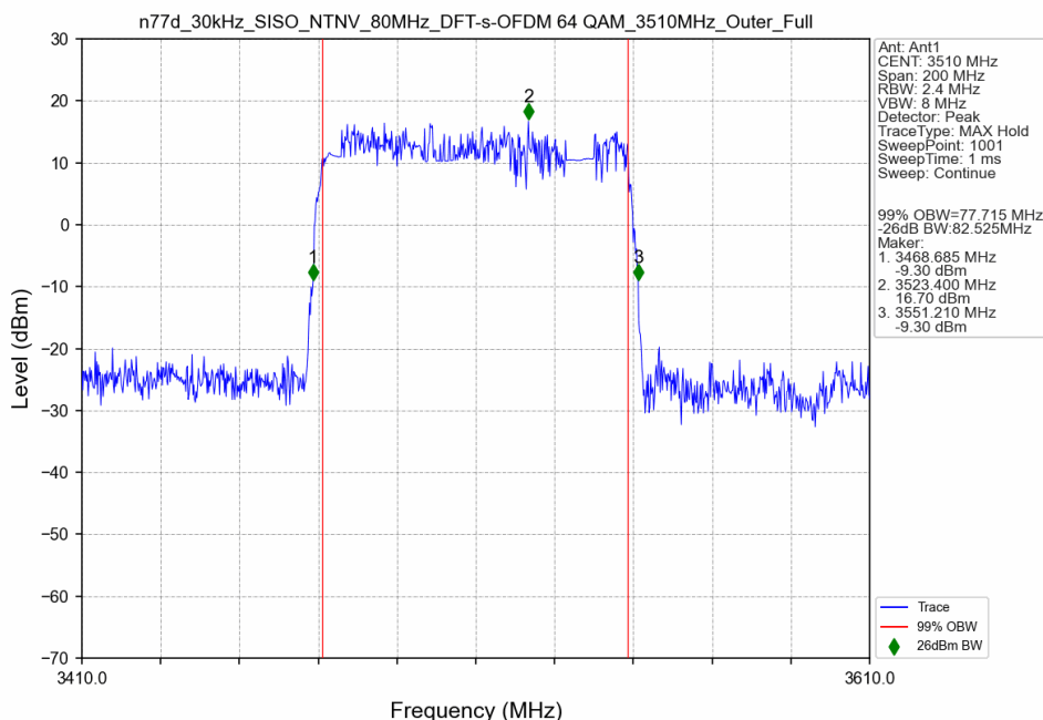
n77d_30kHz_SISO_NTNV_80MHz_DFT-s-OFDM 64 QAM_3510MHz_Outer_Full
