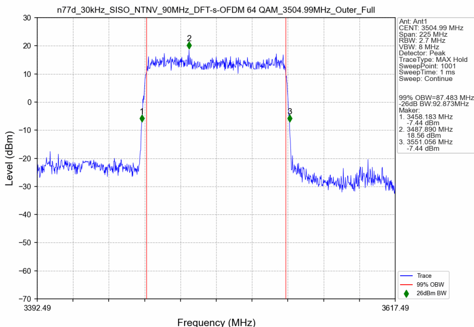
n77d_30kHz_SISO_NTNV_90MHz_DFT-s-OFDM 64 QAM_3504.99MHz_Outer_Full
