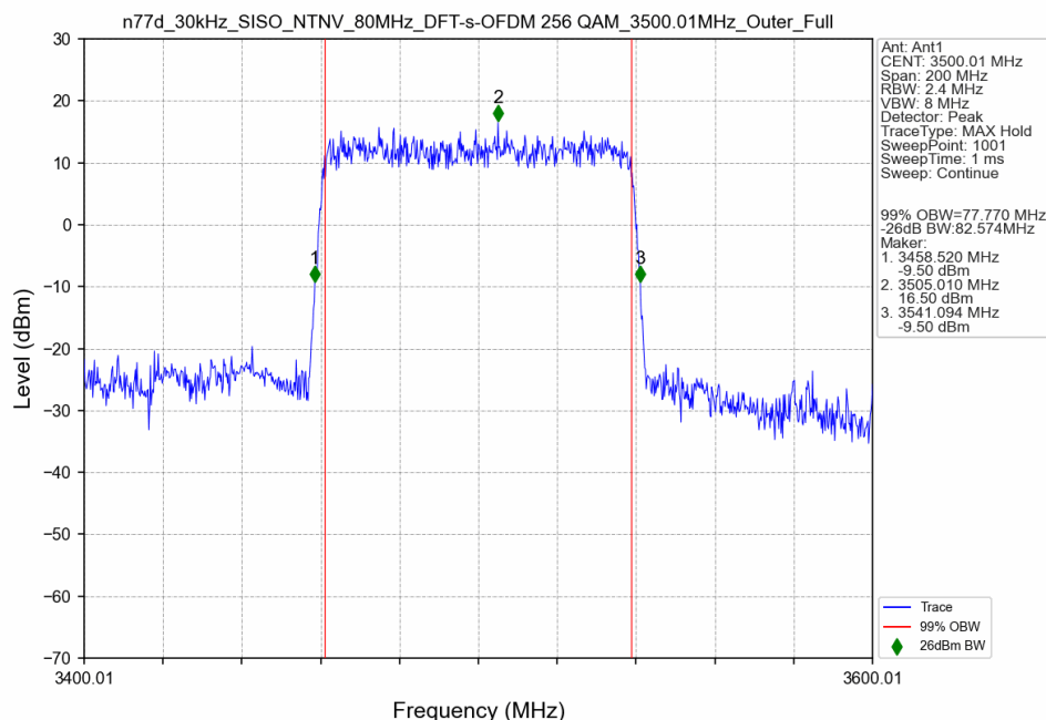
n77d_30kHz_SISO_NTNV_80MHz_DFT-s-OFDM 256 QAM_3500.01MHz_Outer_Full
