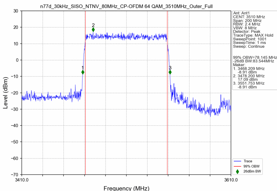
n77d_30kHz_SISO_NTNV_80MHz_CP-OFDM 64 QAM_3510MHz_Outer_Full
