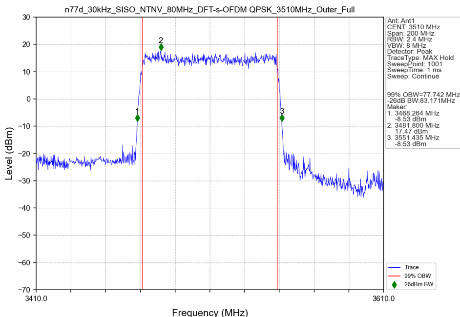
n77d_30kHz_SISO_NTNV_80MHz_DFT-s-OFDM QPSK_3510MHz_Outer_Full
