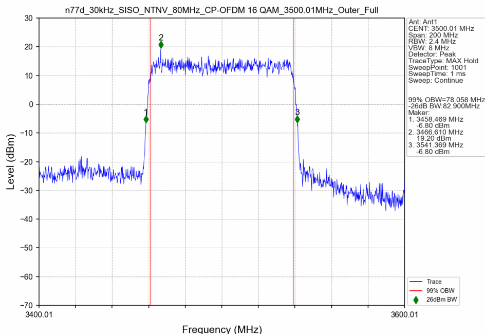
n77d_30kHz_SISO_NTNV_80MHz_CP-OFDM 16 QAM_3500.01MHz_Outer_Full
