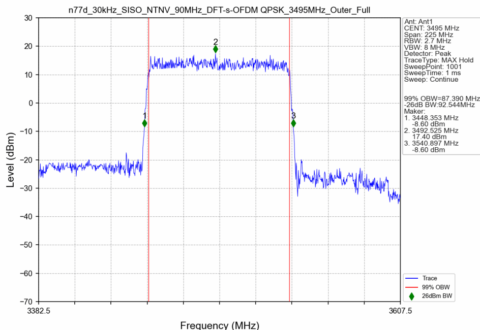
n77d_30kHz_SISO_NTNV_90MHz_DFT-s-OFDM QPSK_3495MHz_Outer_Full
