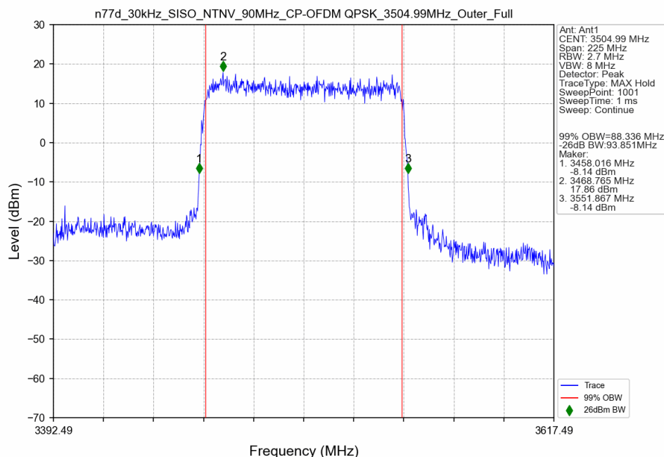
n77d_30kHz_SISO_NTNV_90MHz_CP-OFDM QPSK_3504.99MHz_Outer_Full
