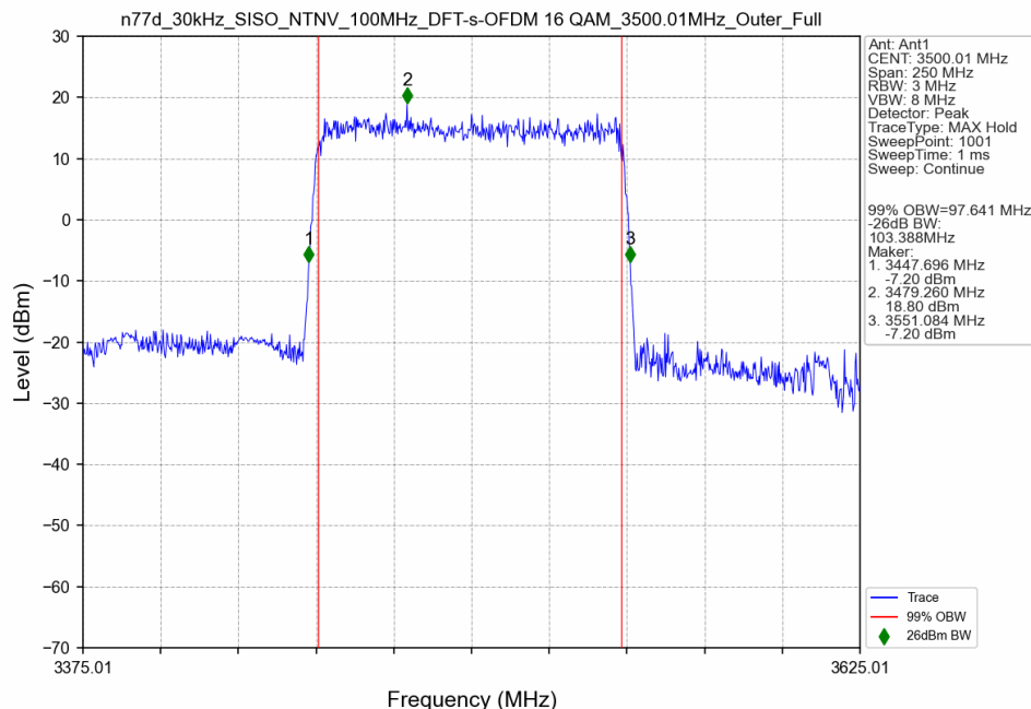
n77d_30kHz_SISO_NTNV_100MHz_DFT-s-OFDM 16 QAM_3500.01MHz_Outer_Full
