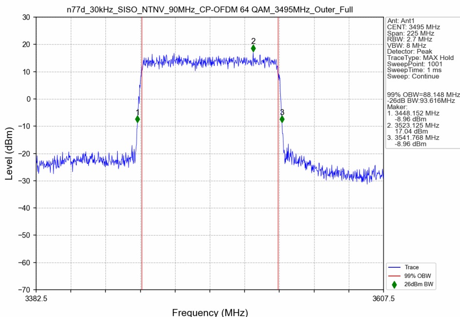
n77d_30kHz_SISO_NTNV_90MHz_CP-OFDM 64 QAM_3495MHz_Outer_Full
