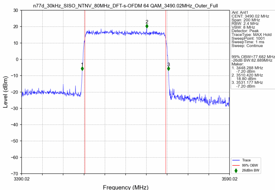
n77d_30kHz_SISO_NTNV_80MHz_DFT-s-OFDM 64 QAM_3490.02MHz_Outer_Full
