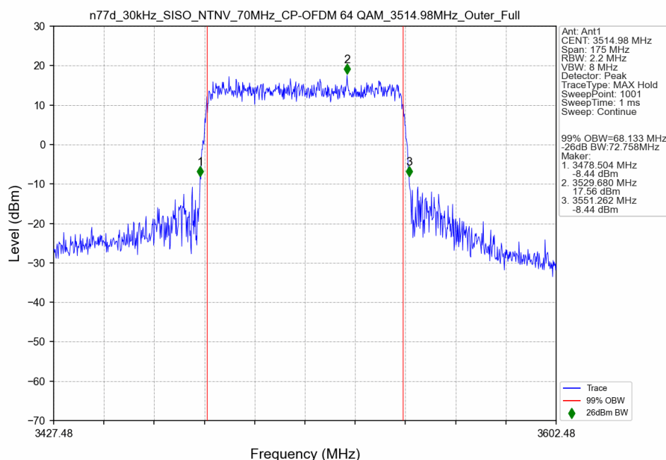
n77d_30kHz_SISO_NTNV_70MHz_CP-OFDM 64 QAM_3514.98MHz_Outer_Full
