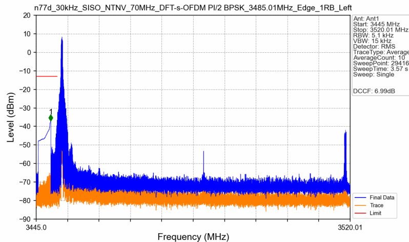
n77d_30kHz_SISO_NTNV_70MHz_DFT-s-OFDM PI/2 BPSK_3485.01MHz_Edge_1RB_Left
