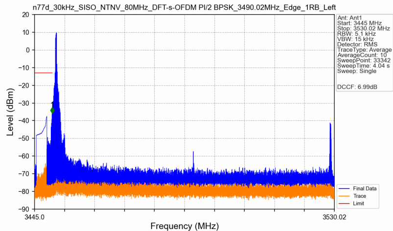
n77d_30kHz_SISO_NTNV_80MHz_DFT-s-OFDM PI/2 BPSK_3490.02MHz_Edge_1RB_Left
