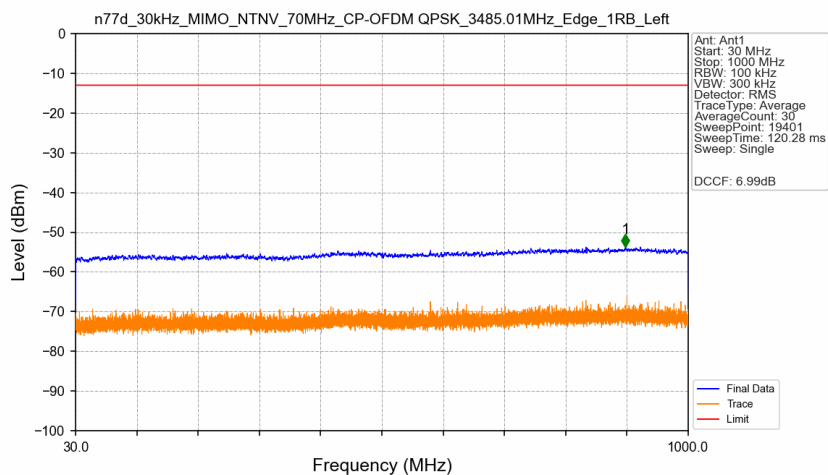
n77d_30kHz_MIMO_NTNV_70MHz_CP-OFDM QPSK_3485.01MHz_Edge_1RB_Left
