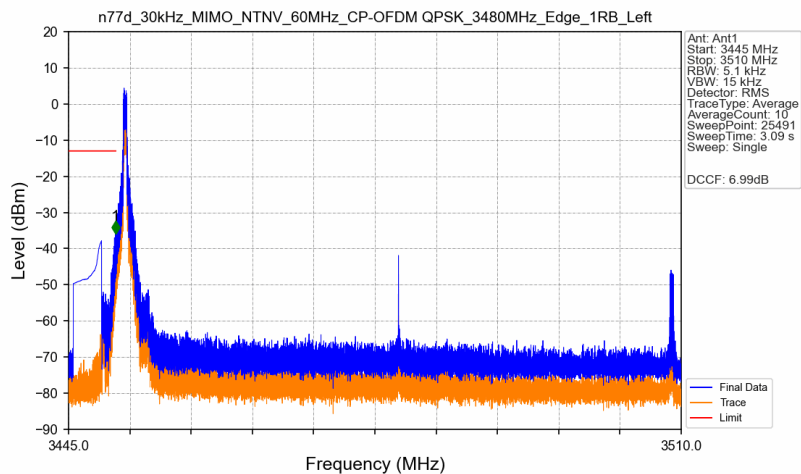
n77d_30kHz_MIMO_NTNV_60MHz_CP-OFDM QPSK_3480MHz_Edge_1RB_Left
