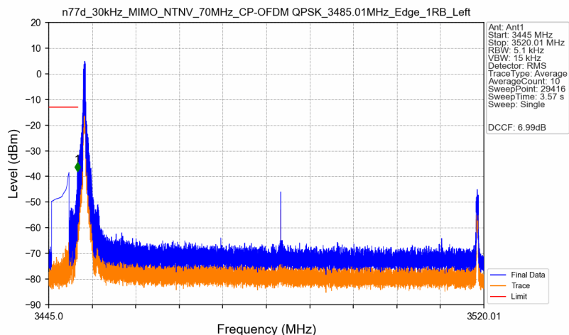
n77d_30kHz_MIMO_NTNV_70MHz_CP-OFDM QPSK_3485.01MHz_Edge_1RB_Left
