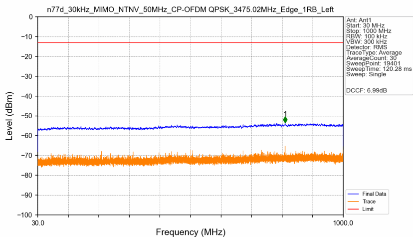
n77d_30kHz_MIMO_NTNV_50MHz_CP-OFDM QPSK_3475.02MHz_Edge_1RB_Left
