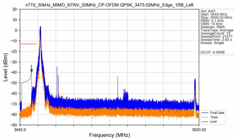
n77d_30kHz_MIMO_NTNV_50MHz_CP-OFDM QPSK_3475.02MHz_Edge_1RB_Left
