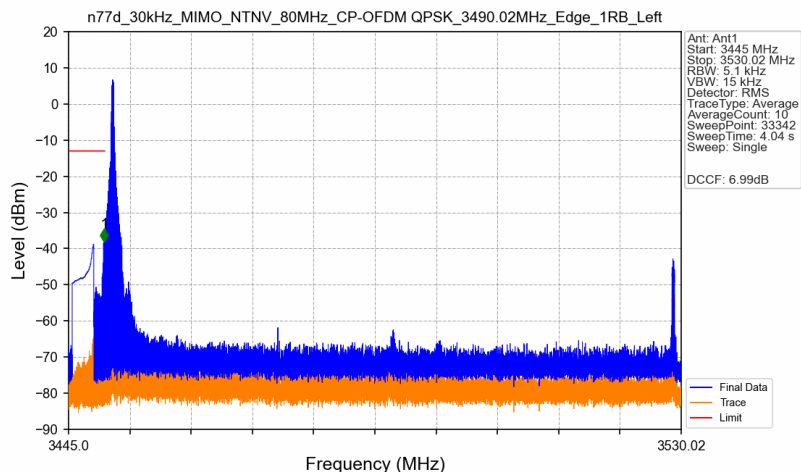
n77d_30kHz_MIMO_NTNV_80MHz_CP-OFDM QPSK_3490.02MHz_Edge_1RB_Left
