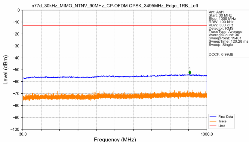
n77d_30kHz_MIMO_NTNV_90MHz_CP-OFDM QPSK_3495MHz_Edge_1RB_Left
