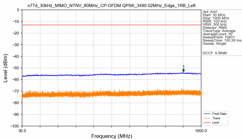
n77d_30kHz_MIMO_NTNV_80MHz_CP-OFDM QPSK_3490.02MHz_Edge_1RB_Left
