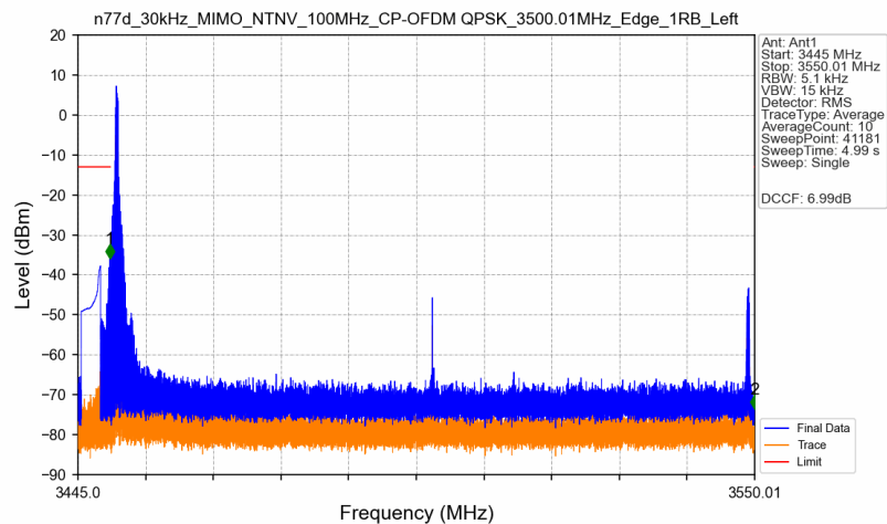
n77d_30kHz_MIMO_NTNV_100MHz_CP-OFDM QPSK_3500.01MHz_Edge_1RB_Left
