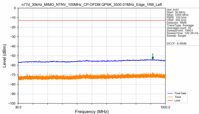
n77d_30kHz_MIMO_NTNV_100MHz_CP-OFDM QPSK_3500.01MHz_Edge_1RB_Left
