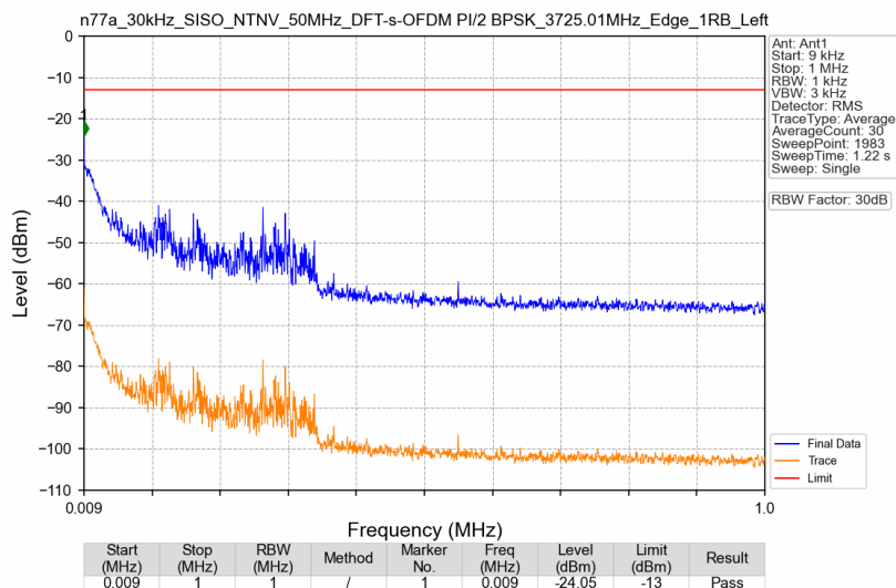
n77a_30kHz_SISO_NTNV_50MHz_DFT-s-OFDM PI/2 BPSK_3725.01MHz_Edge_1RB_Left
