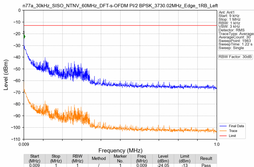
n77a_30kHz_SISO_NTNV_60MHz_DFT-s-OFDM PI/2 BPSK_3730.02MHz_Edge_1RB_Left
