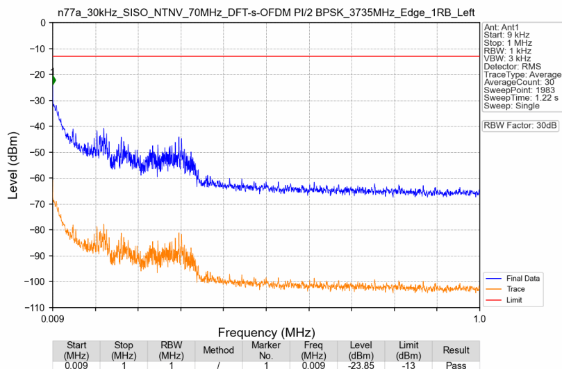
n77a_30kHz_SISO_NTNV_70MHz_DFT-s-OFDM PI/2 BPSK_3735MHz_Edge_1RB_Left
