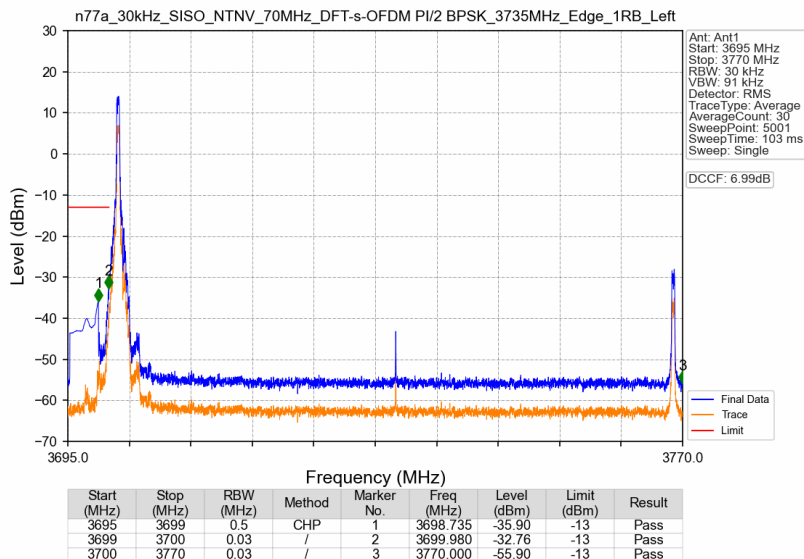
n77a_30kHz_SISO_NTNV_70MHz_DFT-s-OFDM PI/2 BPSK_3735MHz_Edge_1RB_Left
