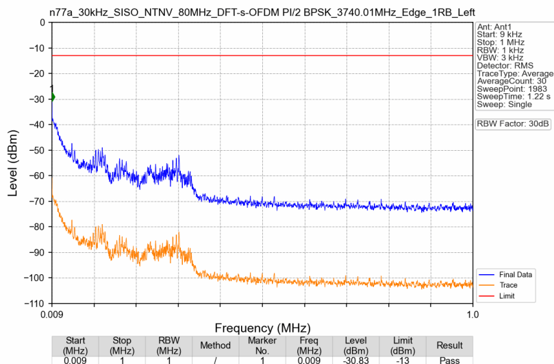
n77a_30kHz_SISO_NTNV_80MHz_DFT-s-OFDM PI/2 BPSK_3740.01MHz_Edge_1RB_Left
