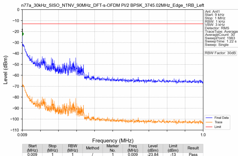
n77a_30kHz_SISO_NTNV_90MHz_DFT-s-OFDM PI/2 BPSK_3745.02MHz_Edge_1RB_Left
