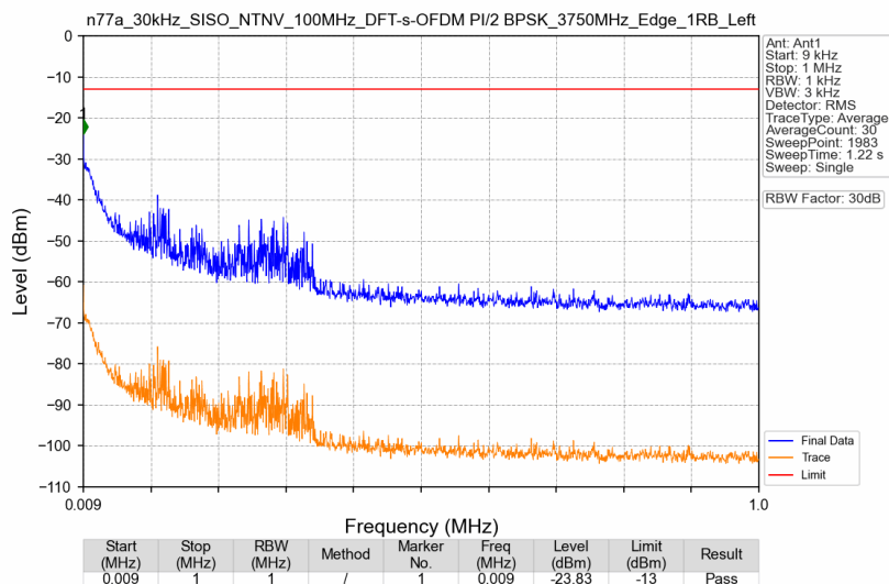
n77a_30kHz_SISO_NTNV_100MHz_DFT-s-OFDM PI/2 BPSK_3750MHz_Edge_1RB_Left
