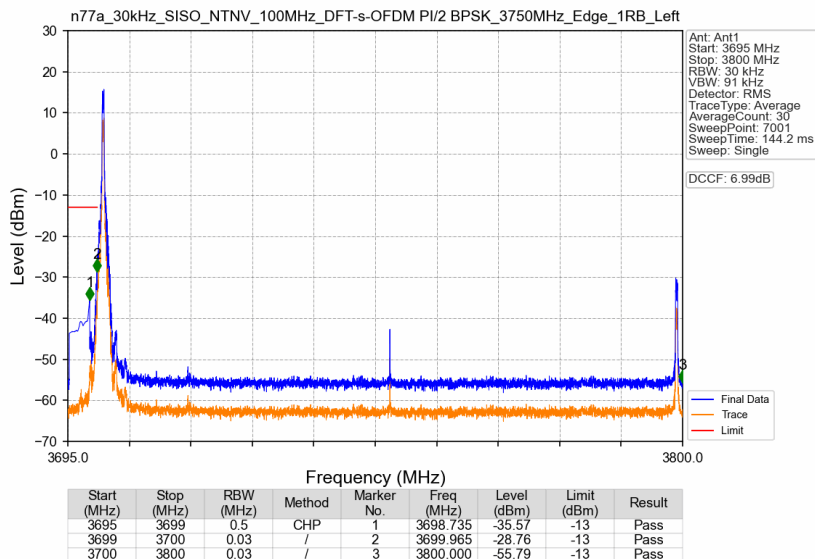
n77a_30kHz_SISO_NTNV_100MHz_DFT-s-OFDM PI/2 BPSK_3750MHz_Edge_1RB_Left
