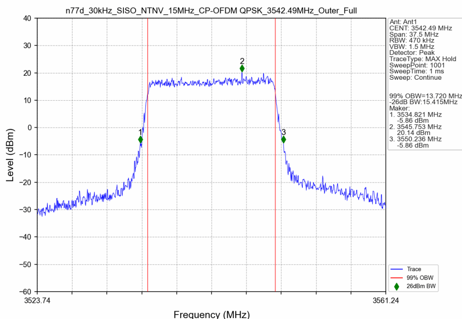
n77d_30kHz_SISO_NTNV_15MHz_CP-OFDM QPSK_3542.49MHz_Outer_Full
