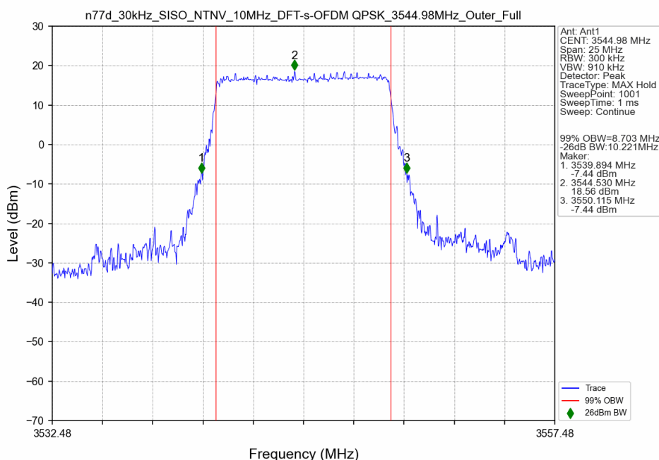
n77d_30kHz_SISO_NTNV_10MHz_DFT-s-OFDM QPSK_3544.98MHz_Outer_Full
