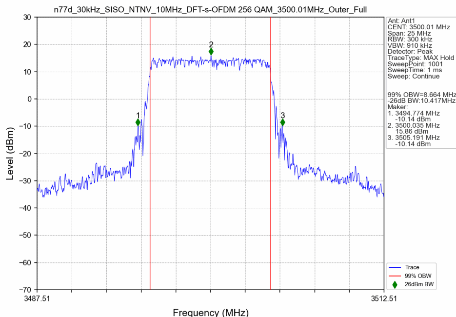
n77d_30kHz_SISO_NTNV_10MHz_DFT-s-OFDM 256 QAM_3500.01MHz_Outer_Full
