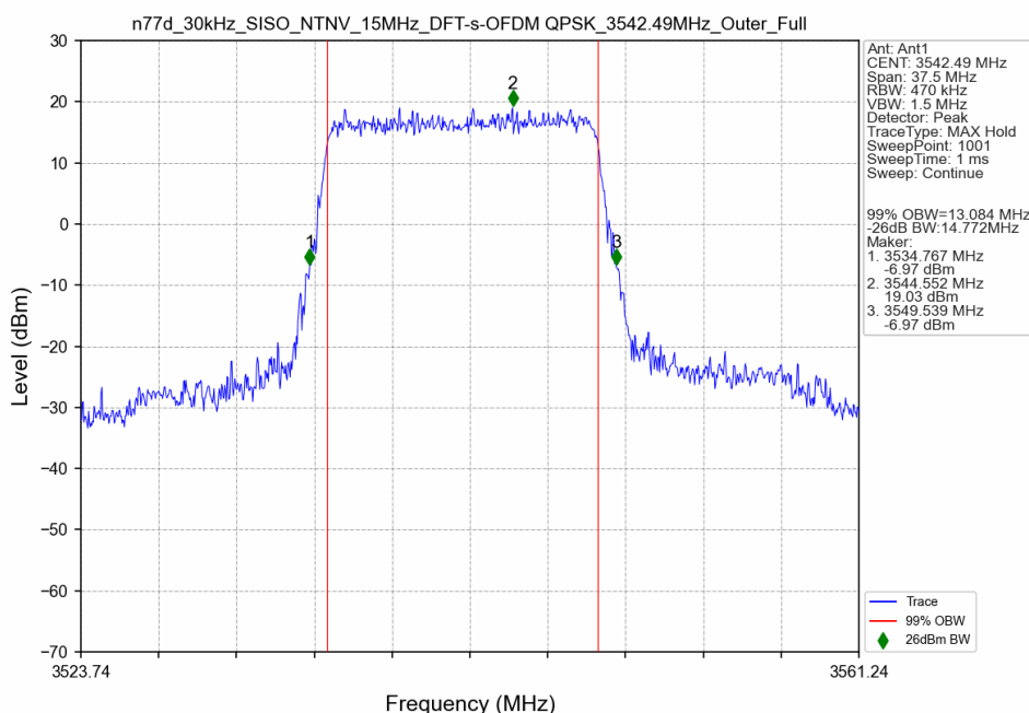
n77d_30kHz_SISO_NTNV_15MHz_DFT-s-OFDM QPSK_3542.49MHz_Outer_Full
