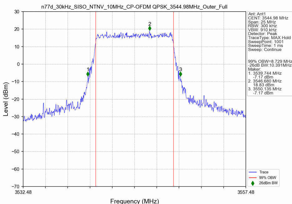
n77d_30kHz_SISO_NTNV_10MHz_CP-OFDM QPSK_3544.98MHz_Outer_Full
