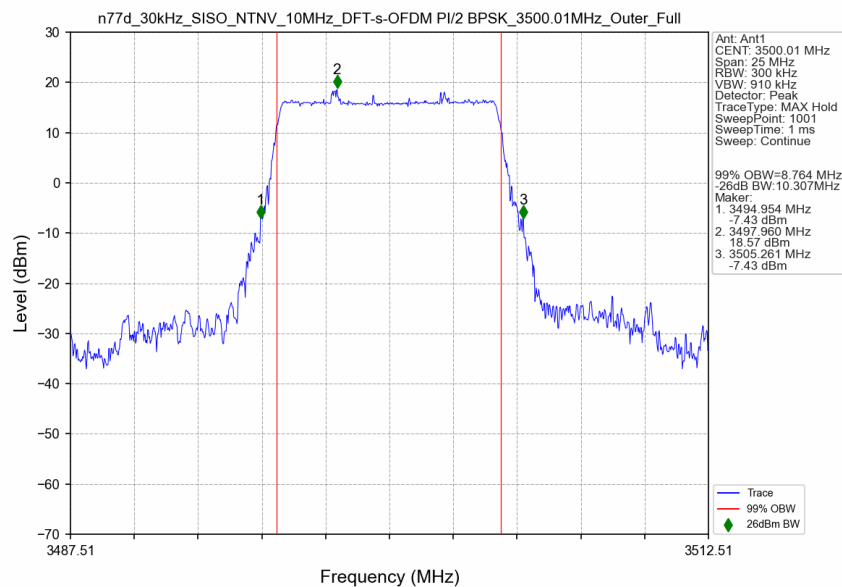
n77d_30kHz_SISO_NTNV_10MHz_DFT-s-OFDM PI/2 BPSK_3500.01MHz_Outer_Full
