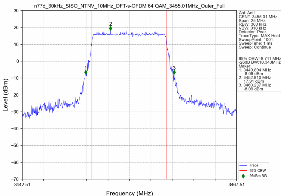
n77d_30kHz_SISO_NTNV_10MHz_DFT-s-OFDM 64 QAM_3455.01MHz_Outer_Full
