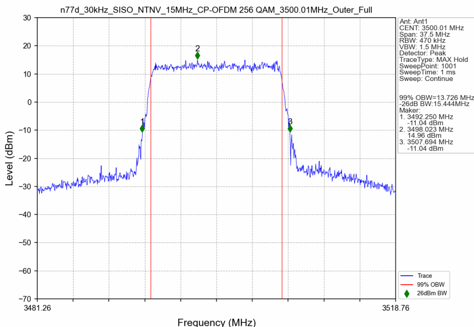
n77d_30kHz_SISO_NTNV_15MHz_CP-OFDM 256 QAM_3500.01MHz_Outer_Full
