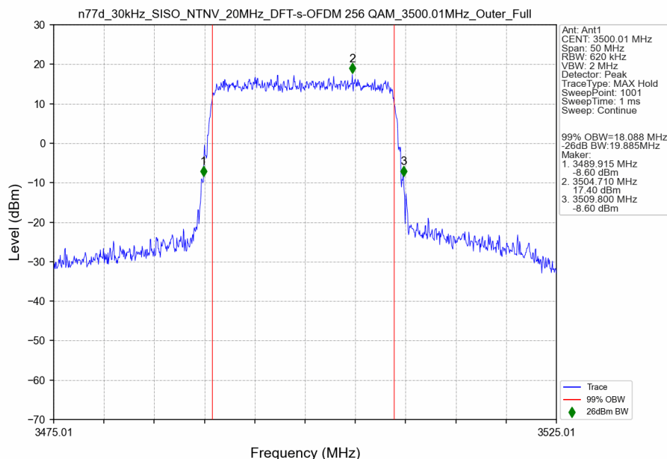
n77d_30kHz_SISO_NTNV_20MHz_DFT-s-OFDM 256 QAM_3500.01MHz_Outer_Full
