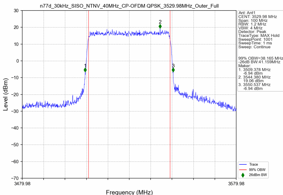
n77d_30kHz_SISO_NTNV_40MHz_CP-OFDM QPSK_3529.98MHz_Outer_Full
