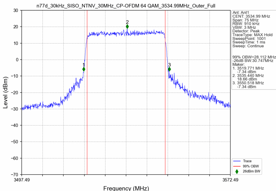
n77d_30kHz_SISO_NTNV_30MHz_CP-OFDM 64 QAM_3534.99MHz_Outer_Full
