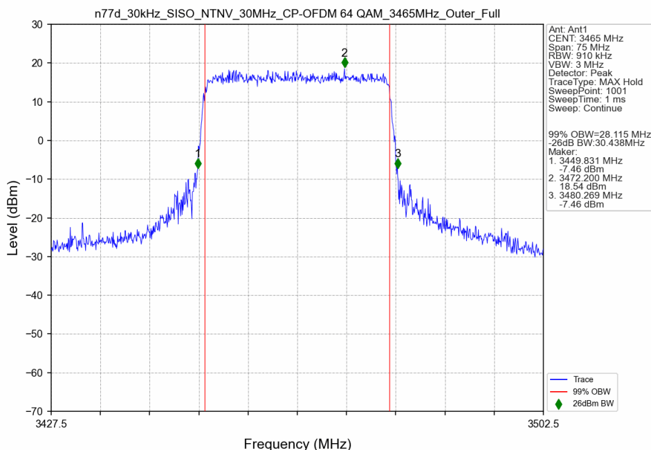
n77d_30kHz_SISO_NTNV_30MHz_CP-OFDM 64 QAM_3465MHz_Outer_Full
