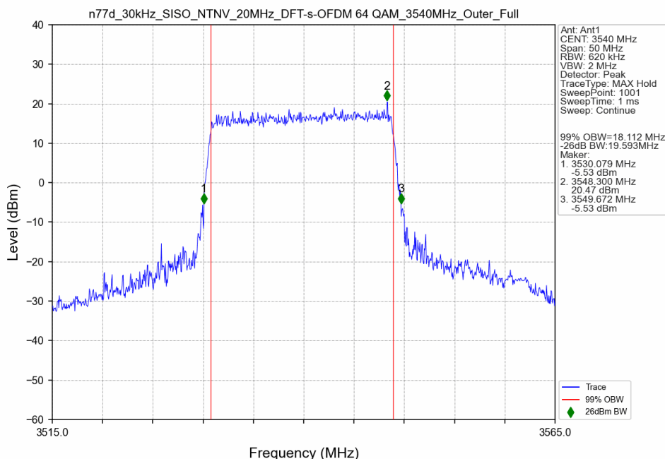
n77d_30kHz_SISO_NTNV_20MHz_DFT-s-OFDM 64 QAM_3540MHz_Outer_Full
