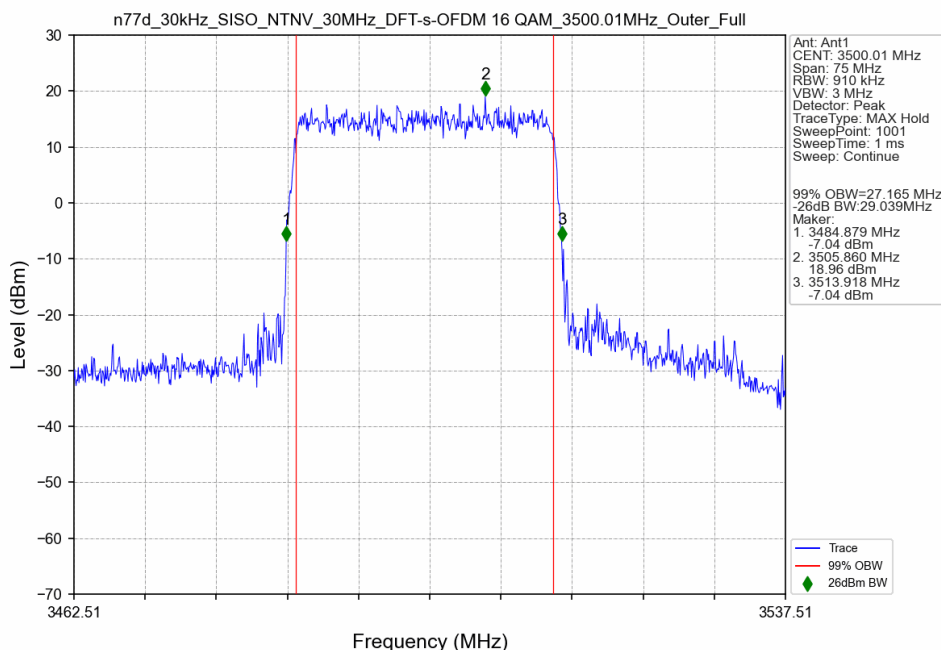
n77d_30kHz_SISO_NTNV_30MHz_DFT-s-OFDM 16 QAM_3500.01MHz_Outer_Full
