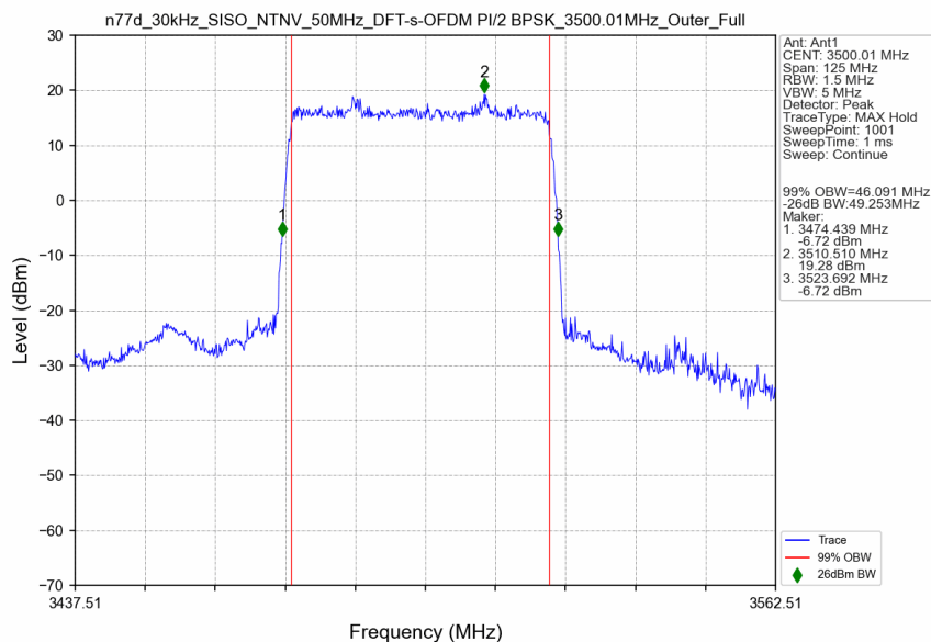
n77d_30kHz_SISO_NTNV_50MHz_DFT-s-OFDM PI/2 BPSK_3500.01MHz_Outer_Full
