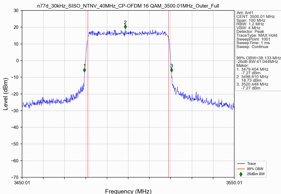
n77d_30kHz_SISO_NTNV_40MHz_CP-OFDM 16 QAM_3500.01MHz_Outer_Full
