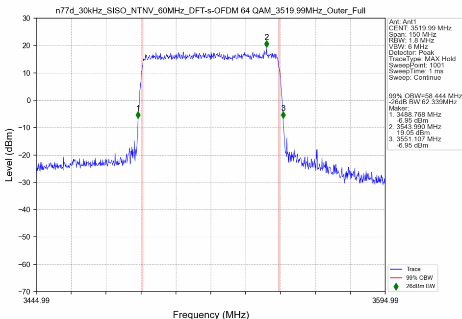
n77d_30kHz_SISO_NTNV_60MHz_DFT-s-OFDM 64 QAM_3519.99MHz_Outer_Full
