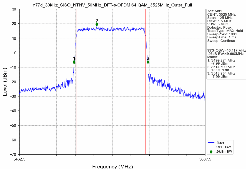
n77d_30kHz_SISO_NTNV_50MHz_DFT-s-OFDM 64 QAM_3525MHz_Outer_Full
