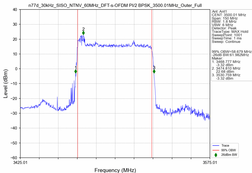
n77d_30kHz_SISO_NTNV_60MHz_DFT-s-OFDM PI/2 BPSK_3500.01MHz_Outer_Full
