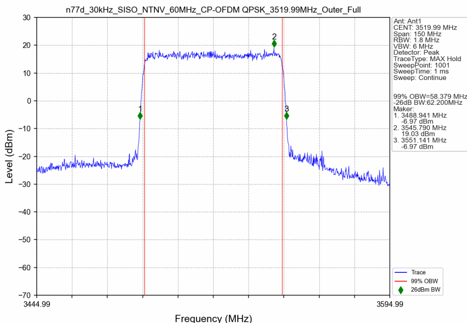
n77d_30kHz_SISO_NTNV_60MHz_CP-OFDM QPSK_3519.99MHz_Outer_Full
