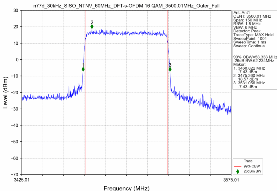
n77d_30kHz_SISO_NTNV_60MHz_DFT-s-OFDM 16 QAM_3500.01MHz_Outer_Full
