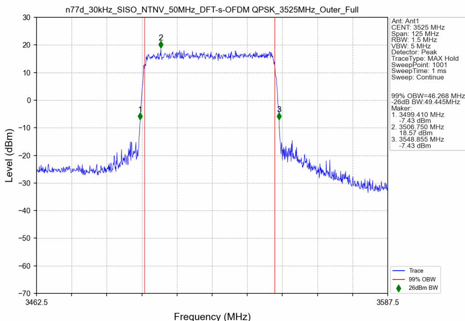
n77d_30kHz_SISO_NTNV_50MHz_DFT-s-OFDM QPSK_3525MHz_Outer_Full
