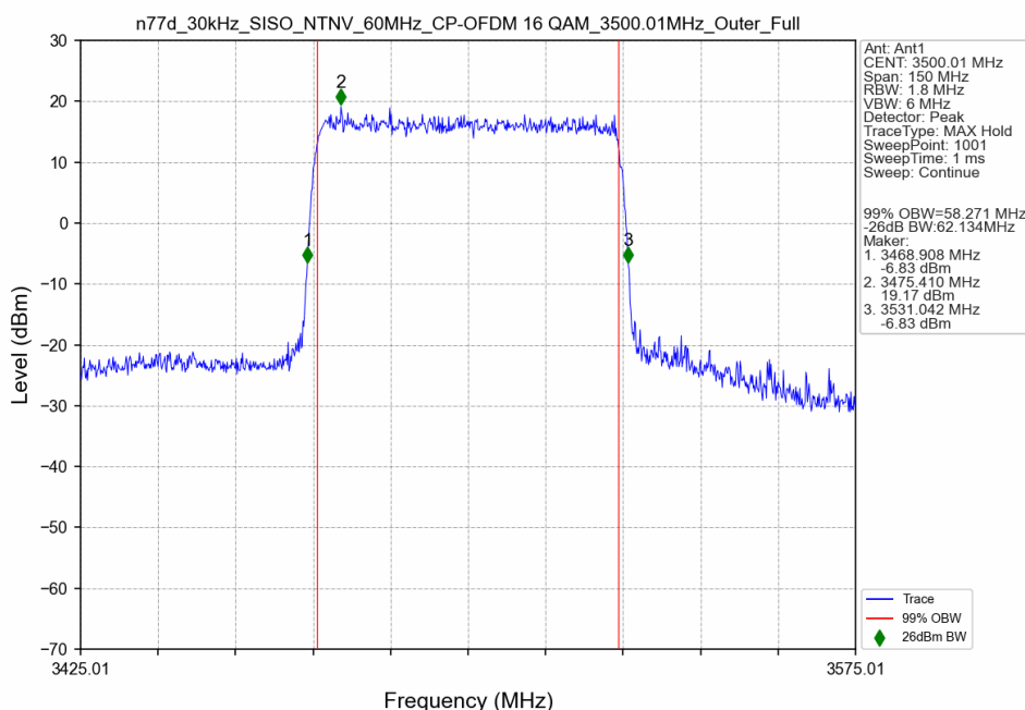
n77d_30kHz_SISO_NTNV_60MHz_CP-OFDM 16 QAM_3500.01MHz_Outer_Full
