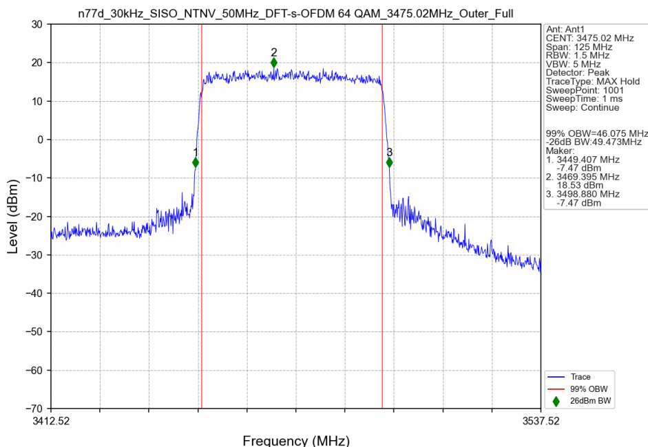
n77d_30kHz_SISO_NTNV_50MHz_DFT-s-OFDM 64 QAM_3475.02MHz_Outer_Full
