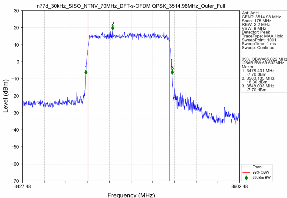
n77d_30kHz_SISO_NTNV_70MHz_DFT-s-OFDM QPSK_3514.98MHz_Outer_Full
