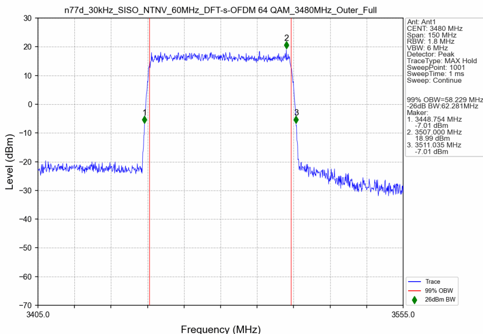
n77d_30kHz_SISO_NTNV_60MHz_DFT-s-OFDM 64 QAM_3480MHz_Outer_Full
