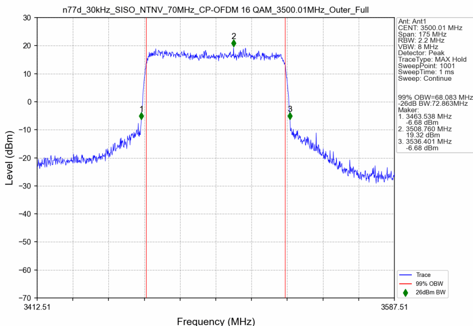
n77d_30kHz_SISO_NTNV_70MHz_CP-OFDM 16 QAM_3500.01MHz_Outer_Full
