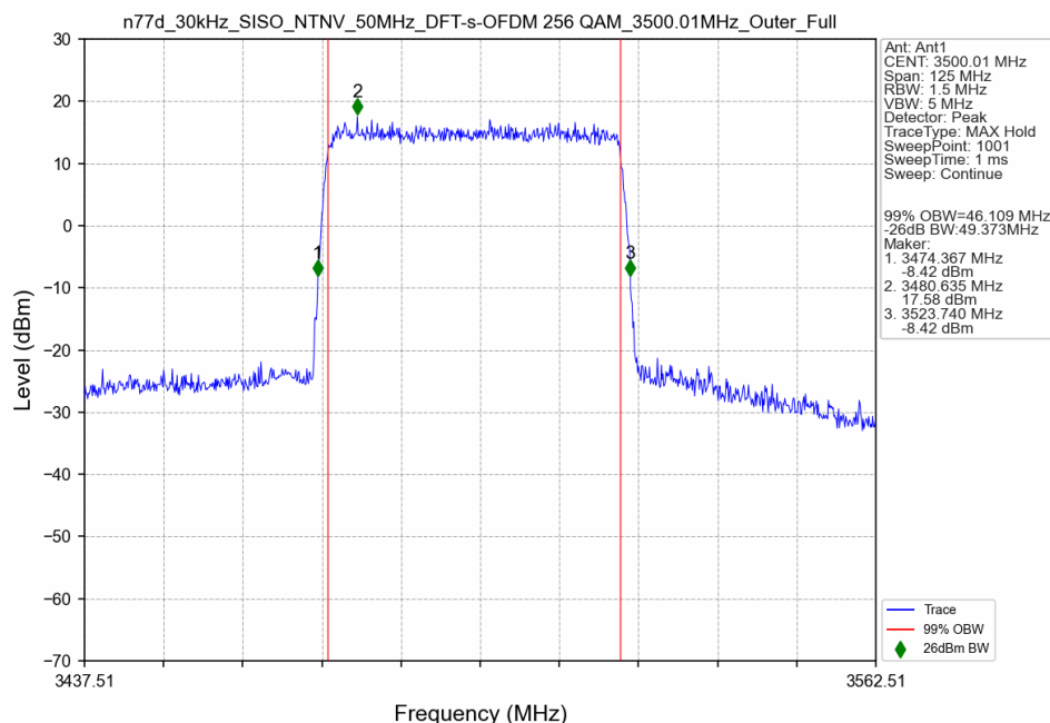
n77d_30kHz_SISO_NTNV_50MHz_DFT-s-OFDM 256 QAM_3500.01MHz_Outer_Full
