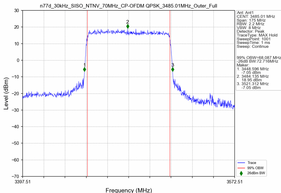
n77d_30kHz_SISO_NTNV_70MHz_CP-OFDM QPSK_3485.01MHz_Outer_Full
