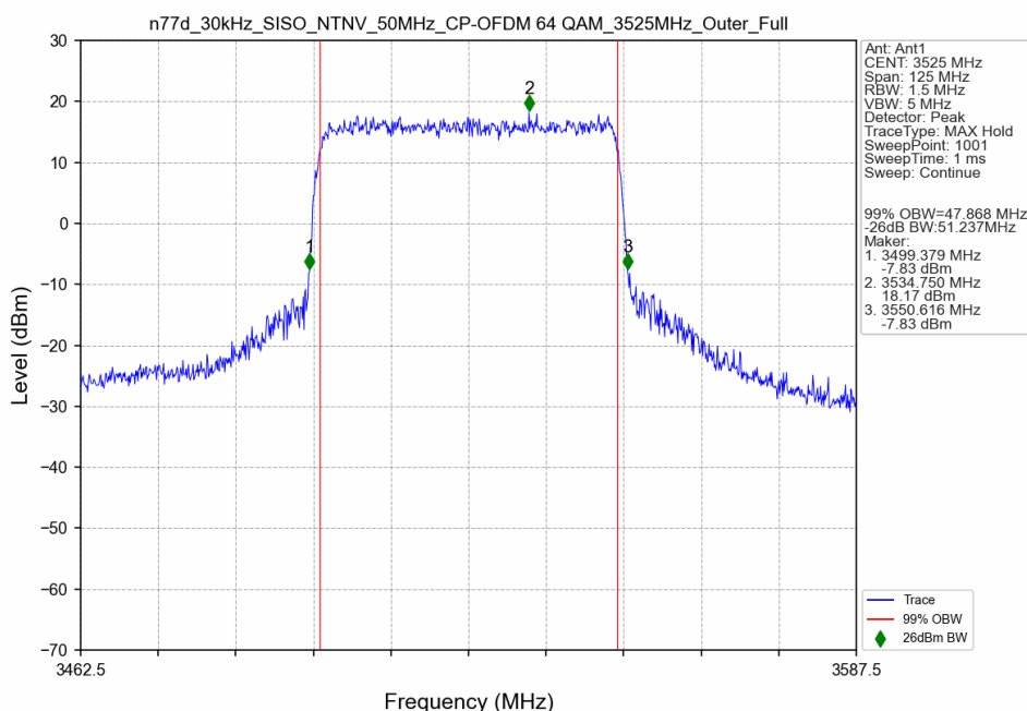
n77d_30kHz_SISO_NTNV_50MHz_CP-OFDM 64 QAM_3525MHz_Outer_Full
