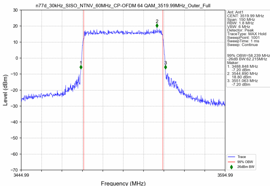
n77d_30kHz_SISO_NTNV_60MHz_CP-OFDM 64 QAM_3519.99MHz_Outer_Full
