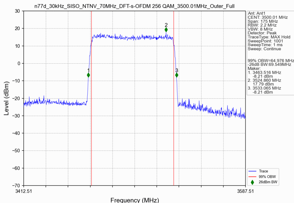
n77d_30kHz_SISO_NTNV_70MHz_DFT-s-OFDM 256 QAM_3500.01MHz_Outer_Full
