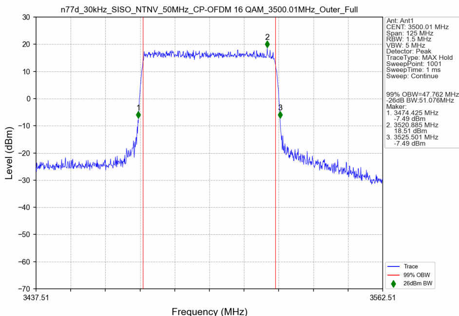
n77d_30kHz_SISO_NTNV_50MHz_CP-OFDM 16 QAM_3500.01MHz_Outer_Full
