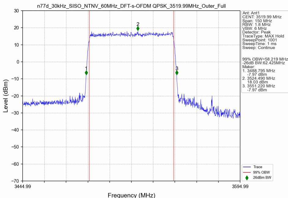
n77d_30kHz_SISO_NTNV_60MHz_DFT-s-OFDM QPSK_3519.99MHz_Outer_Full
