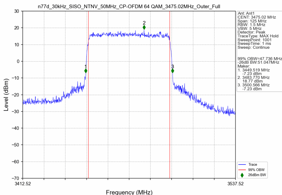
n77d_30kHz_SISO_NTNV_50MHz_CP-OFDM 64 QAM_3475.02MHz_Outer_Full
