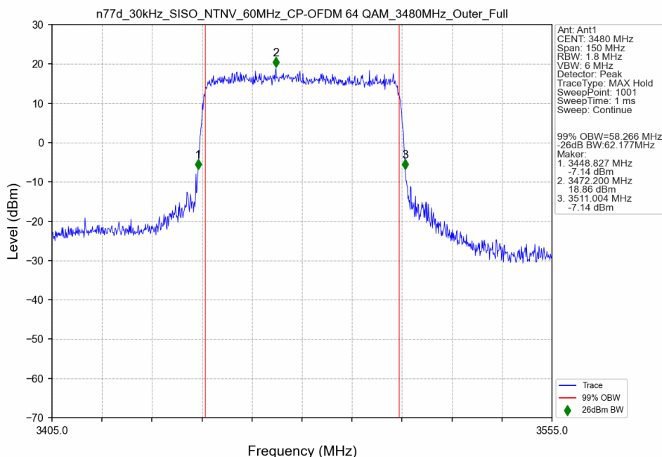
n77d_30kHz_SISO_NTNV_60MHz_CP-OFDM 64 QAM_3480MHz_Outer_Full
