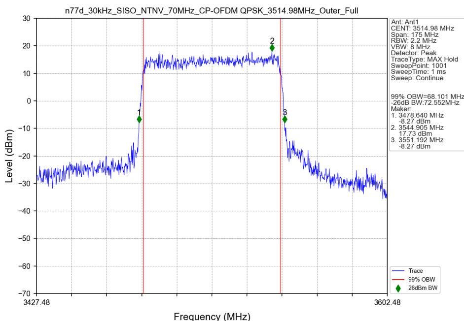
n77d_30kHz_SISO_NTNV_70MHz_CP-OFDM QPSK_3514.98MHz_Outer_Full
