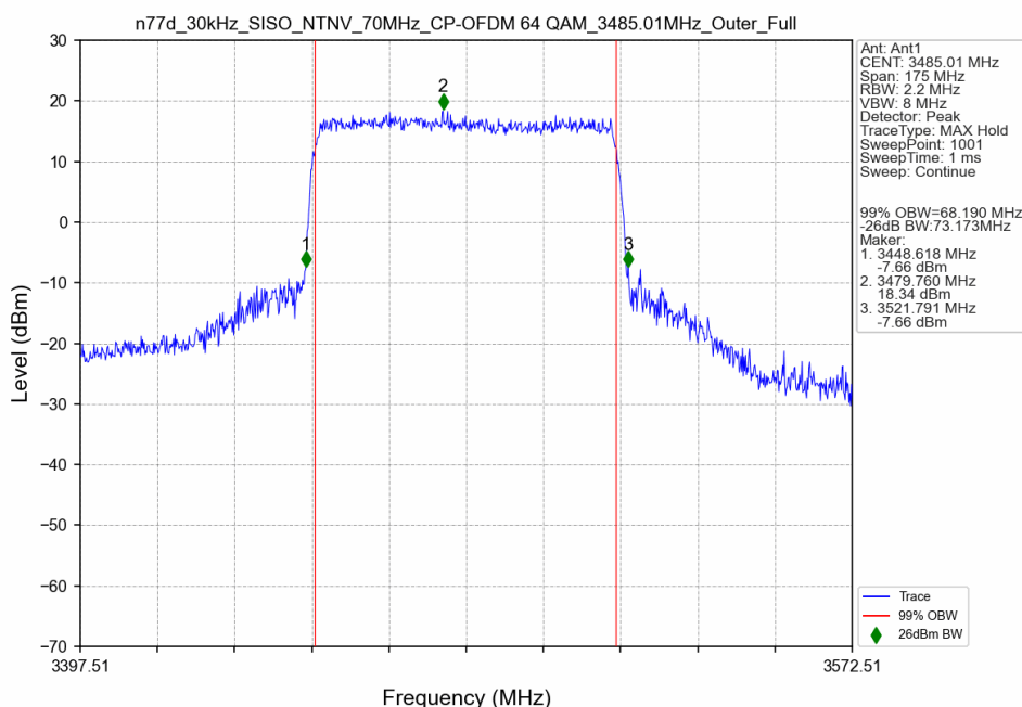
n77d_30kHz_SISO_NTNV_70MHz_CP-OFDM 64 QAM_3485.01MHz_Outer_Full
