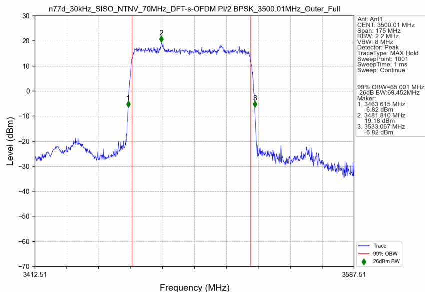
n77d_30kHz_SISO_NTNV_70MHz_DFT-s-OFDM PI/2 BPSK_3500.01MHz_Outer_Full
