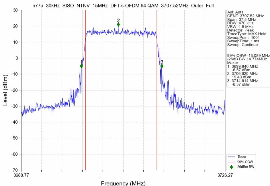
n77a_30kHz_SISO_NTNV_15MHz_DFT-s-OFDM 64 QAM_3707.52MHz_Outer_Full
