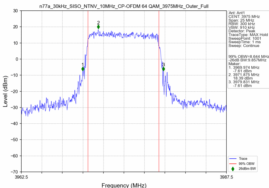
n77a_30kHz_SISO_NTNV_10MHz_CP-OFDM 64 QAM_3975MHz_Outer_Full
