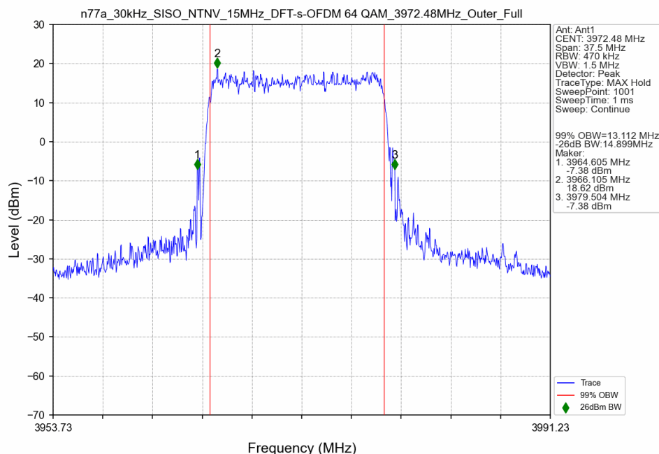
n77a_30kHz_SISO_NTNV_15MHz_DFT-s-OFDM 64 QAM_3972.48MHz_Outer_Full
