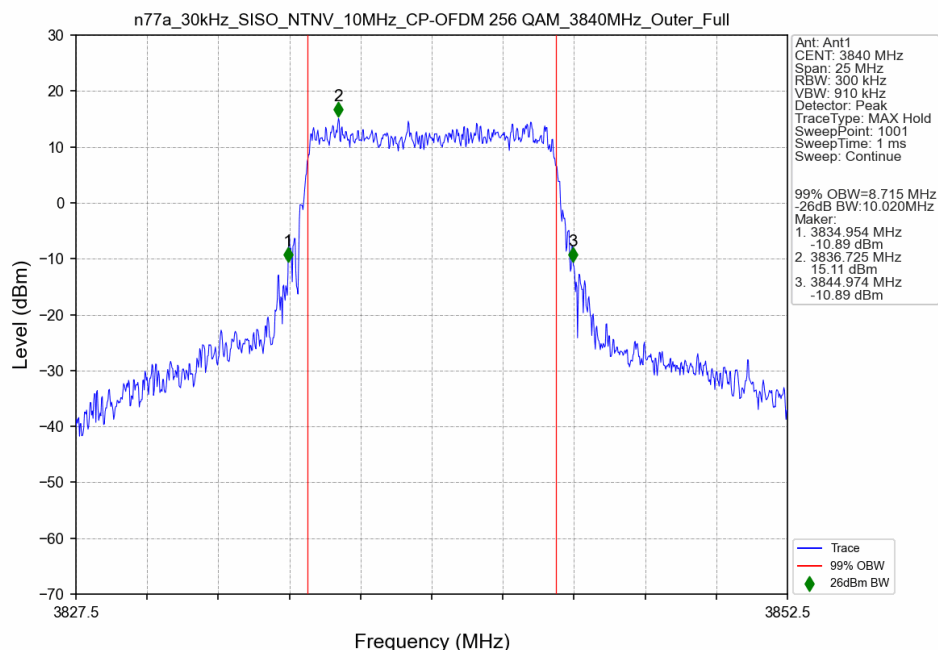
n77a_30kHz_SISO_NTNV_10MHz_CP-OFDM 256 QAM_3840MHz_Outer_Full
