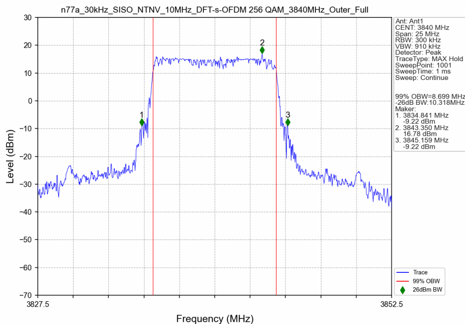
n77a_30kHz_SISO_NTNV_10MHz_DFT-s-OFDM 256 QAM_3840MHz_Outer_Full
