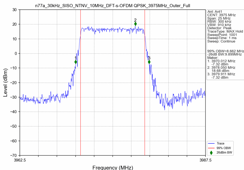
n77a_30kHz_SISO_NTNV_10MHz_DFT-s-OFDM QPSK_3975MHz_Outer_Full
