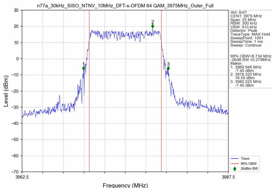
n77a_30kHz_SISO_NTNV_10MHz_DFT-s-OFDM 64 QAM_3975MHz_Outer_Full
