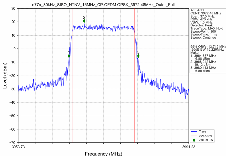
n77a_30kHz_SISO_NTNV_15MHz_CP-OFDM QPSK_3972.48MHz_Outer_Full
