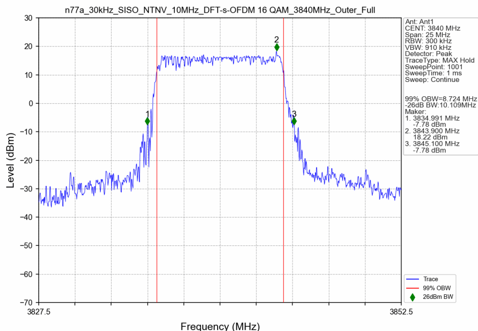
n77a_30kHz_SISO_NTNV_10MHz_DFT-s-OFDM 16 QAM_3840MHz_Outer_Full
