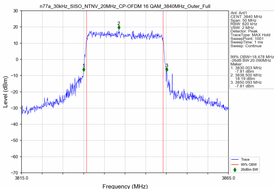
n77a_30kHz_SISO_NTNV_20MHz_CP-OFDM 16 QAM_3840MHz_Outer_Full
