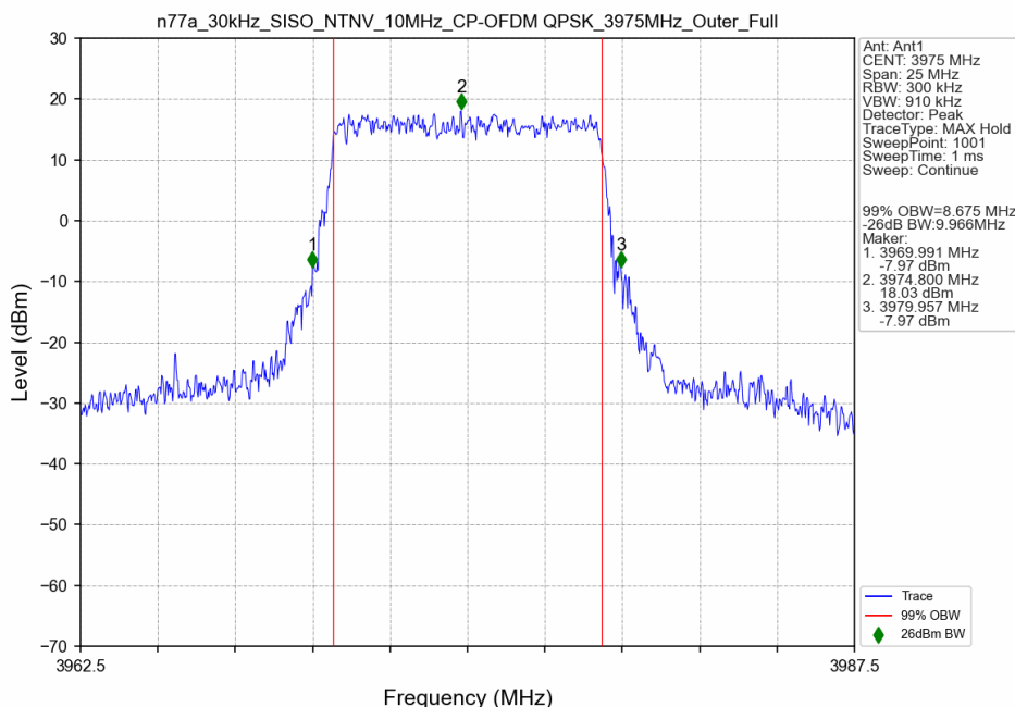
n77a_30kHz_SISO_NTNV_10MHz_CP-OFDM QPSK_3975MHz_Outer_Full
