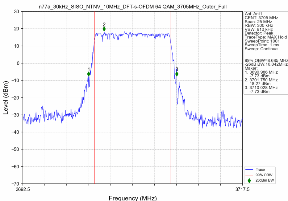
n77a_30kHz_SISO_NTNV_10MHz_DFT-s-OFDM 64 QAM_3705MHz_Outer_Full
