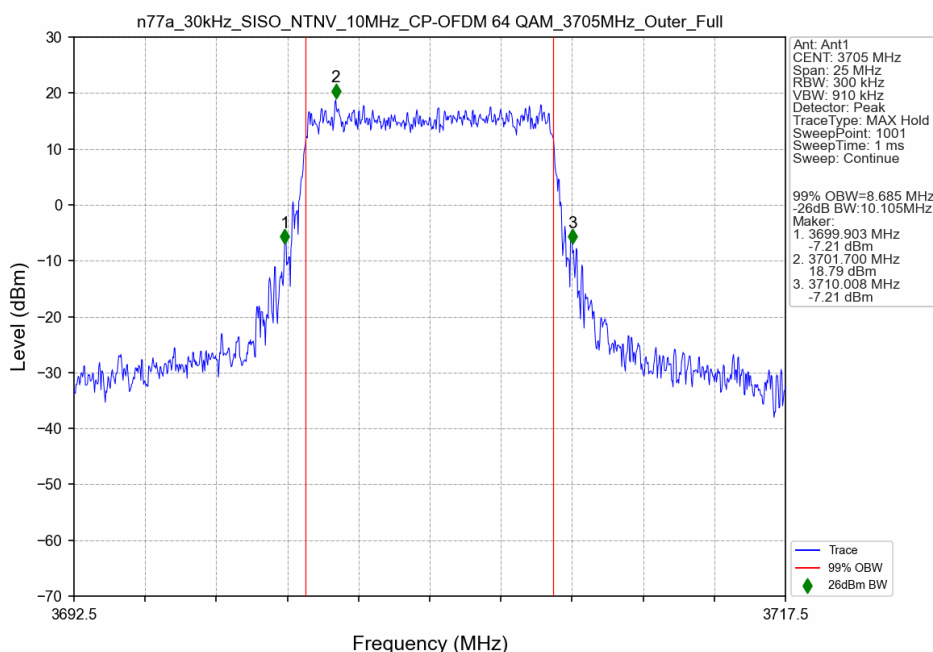
n77a_30kHz_SISO_NTNV_10MHz_CP-OFDM 64 QAM_3705MHz_Outer_Full
