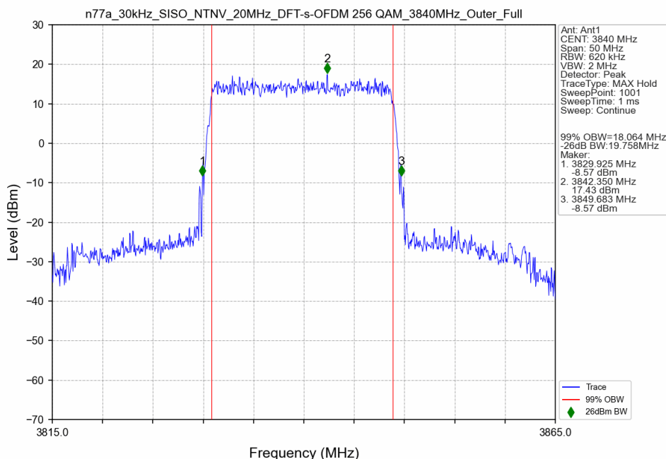
n77a_30kHz_SISO_NTNV_20MHz_DFT-s-OFDM 256 QAM_3840MHz_Outer_Full
