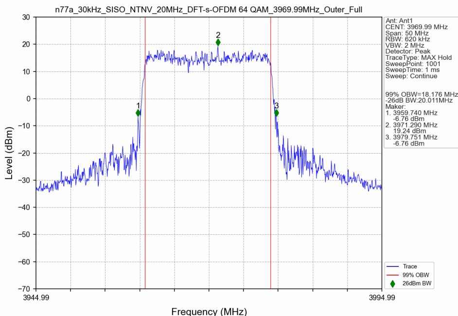
n77a_30kHz_SISO_NTNV_20MHz_DFT-s-OFDM 64 QAM_3969.99MHz_Outer_Full
