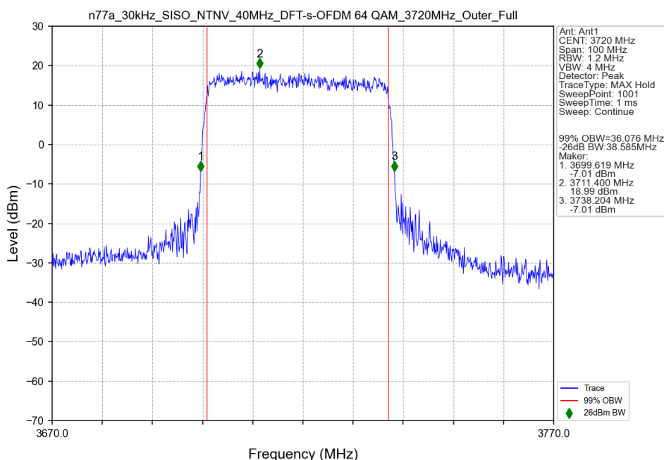
n77a_30kHz_SISO_NTNV_40MHz_DFT-s-OFDM 64 QAM_3720MHz_Outer_Full
