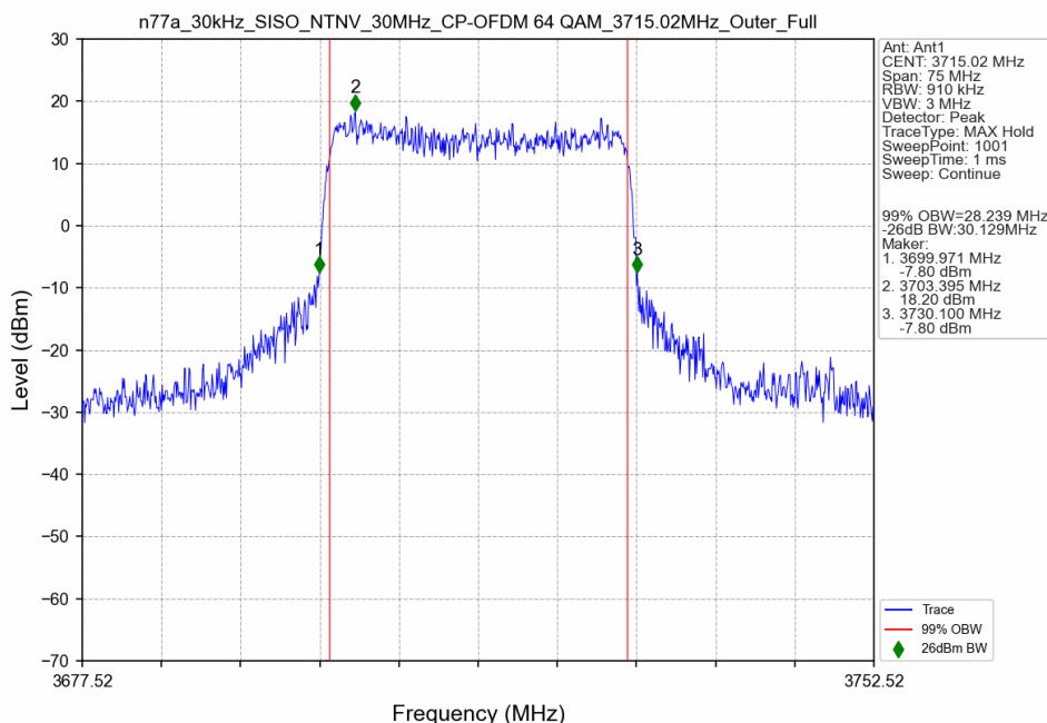
n77a_30kHz_SISO_NTNV_30MHz_CP-OFDM 64 QAM_3715.02MHz_Outer_Full
