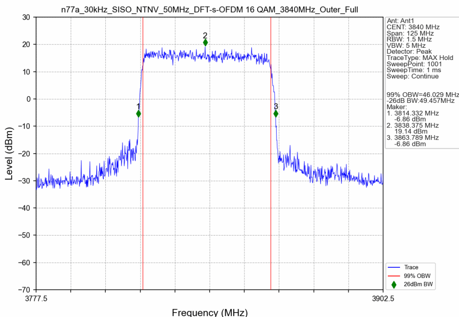
n77a_30kHz_SISO_NTNV_50MHz_DFT-s-OFDM 16 QAM_3840MHz_Outer_Full
