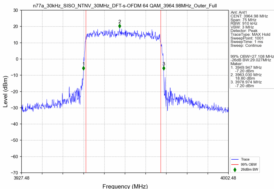
n77a_30kHz_SISO_NTNV_30MHz_DFT-s-OFDM 64 QAM_3964.98MHz_Outer_Full
