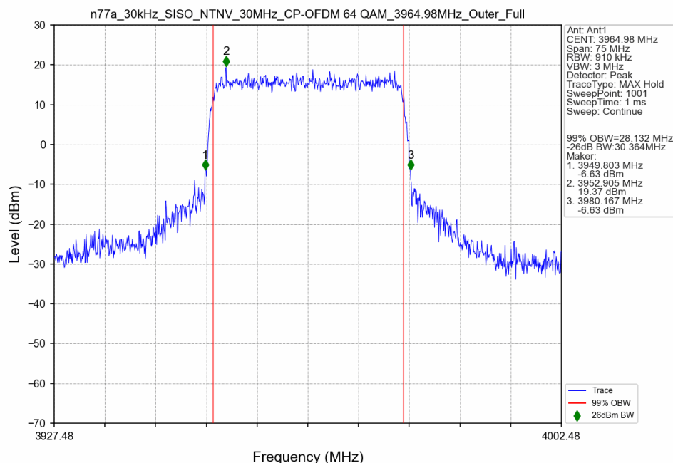
n77a_30kHz_SISO_NTNV_30MHz_CP-OFDM 64 QAM_3964.98MHz_Outer_Full
