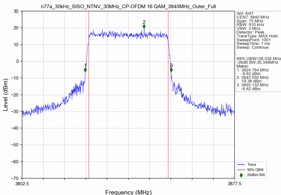
n77a_30kHz_SISO_NTNV_30MHz_CP-OFDM 16 QAM_3840MHz_Outer_Full
