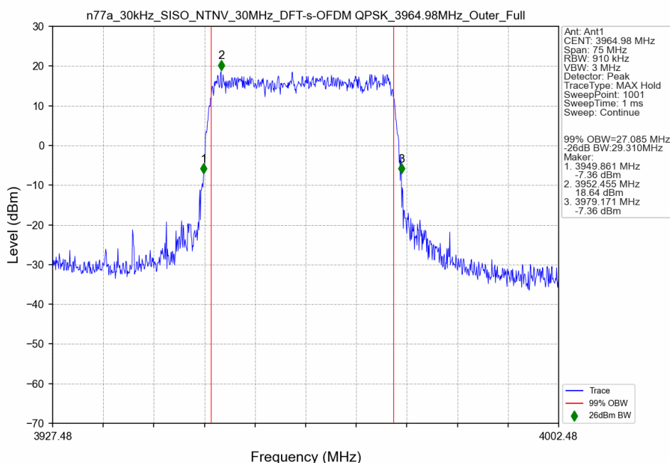
n77a_30kHz_SISO_NTNV_30MHz_DFT-s-OFDM QPSK_3964.98MHz_Outer_Full
