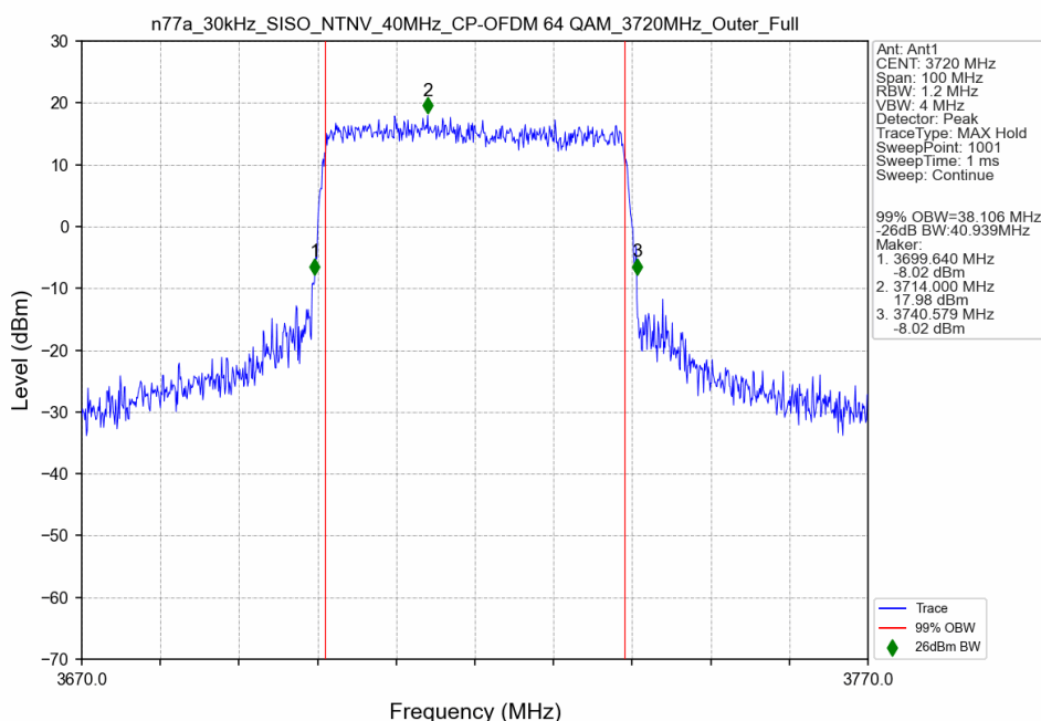
n77a_30kHz_SISO_NTNV_40MHz_CP-OFDM 64 QAM_3720MHz_Outer_Full
