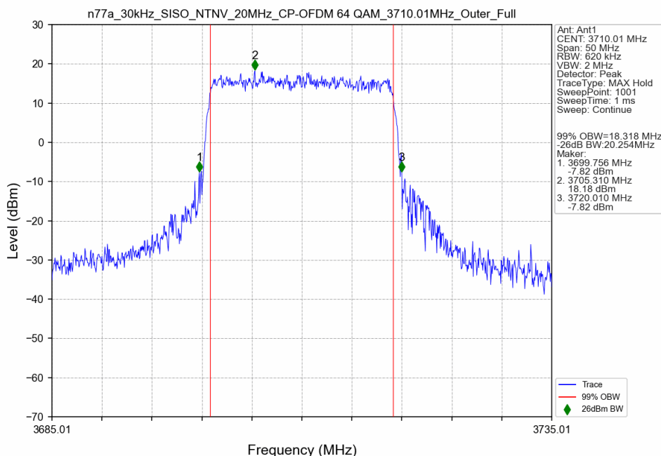
n77a_30kHz_SISO_NTNV_20MHz_CP-OFDM 64 QAM_3710.01MHz_Outer_Full
