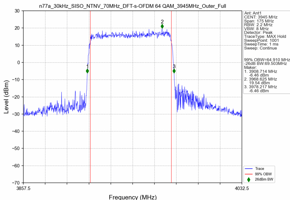
n77a_30kHz_SISO_NTNV_70MHz_DFT-s-OFDM 64 QAM_3945MHz_Outer_Full
