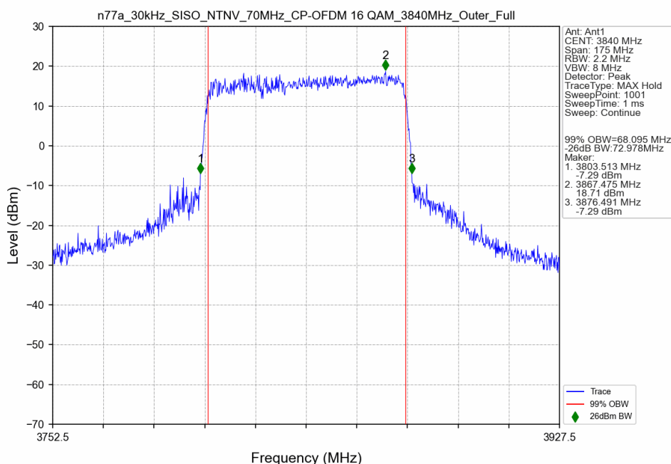
n77a_30kHz_SISO_NTNV_70MHz_CP-OFDM 16 QAM_3840MHz_Outer_Full
