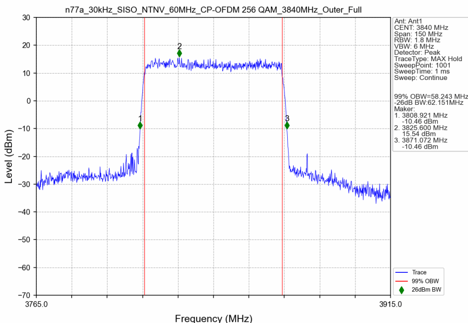
n77a_30kHz_SISO_NTNV_60MHz_CP-OFDM 256 QAM_3840MHz_Outer_Full
