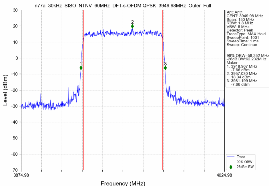
n77a_30kHz_SISO_NTNV_60MHz_DFT-s-OFDM QPSK_3949.98MHz_Outer_Full
