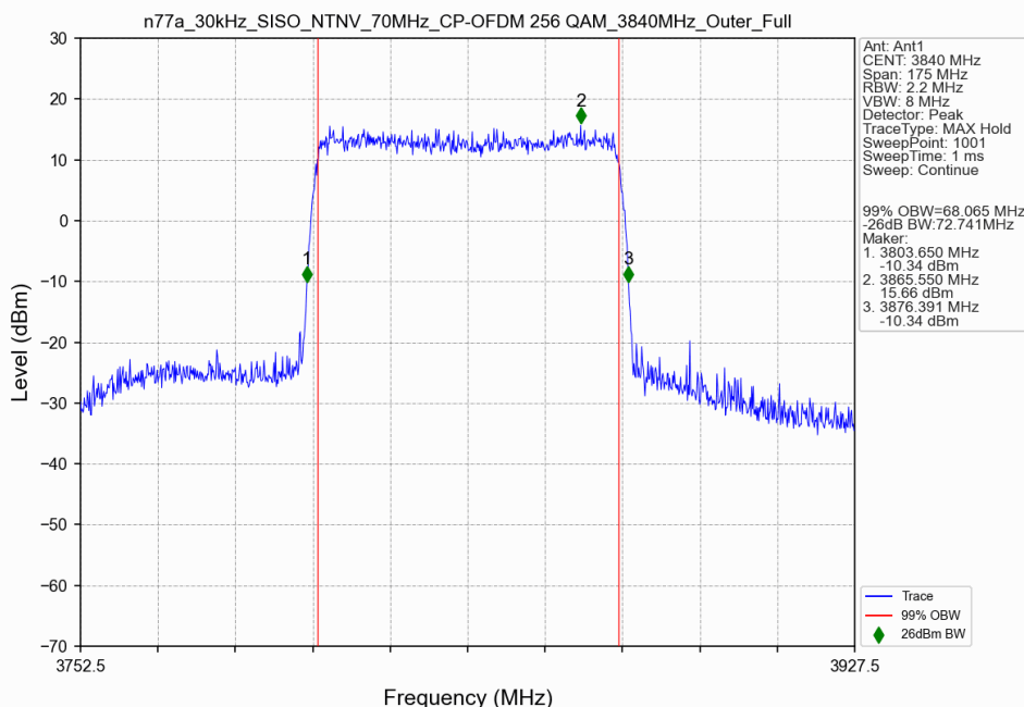
n77a_30kHz_SISO_NTNV_70MHz_CP-OFDM 256 QAM_3840MHz_Outer_Full
