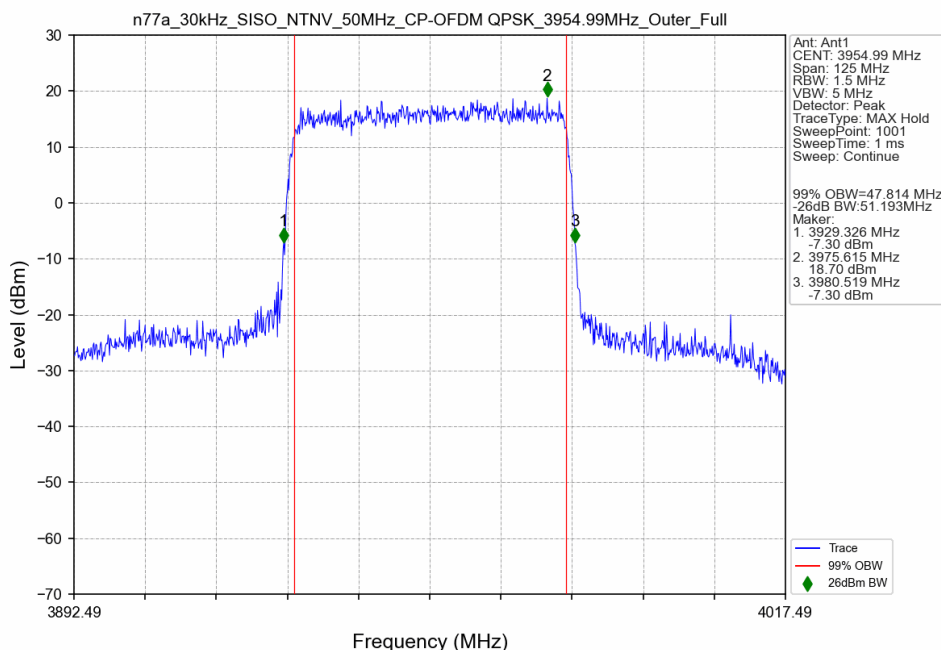
n77a_30kHz_SISO_NTNV_50MHz_CP-OFDM QPSK_3954.99MHz_Outer_Full
