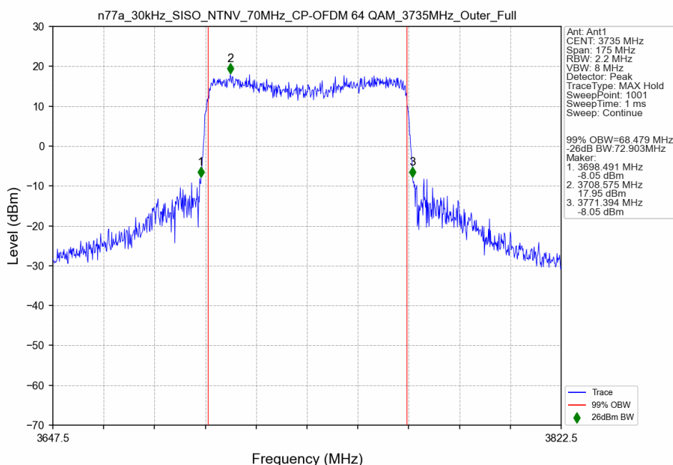
n77a_30kHz_SISO_NTNV_70MHz_CP-OFDM 64 QAM_3735MHz_Outer_Full
