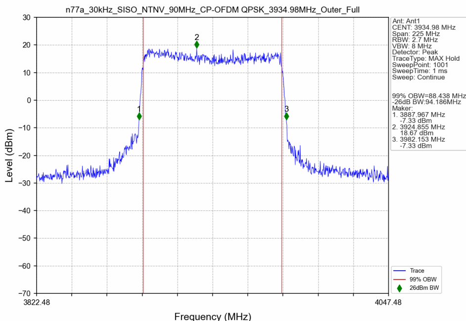
n77a_30kHz_SISO_NTNV_90MHz_CP-OFDM QPSK_3934.98MHz_Outer_Full
