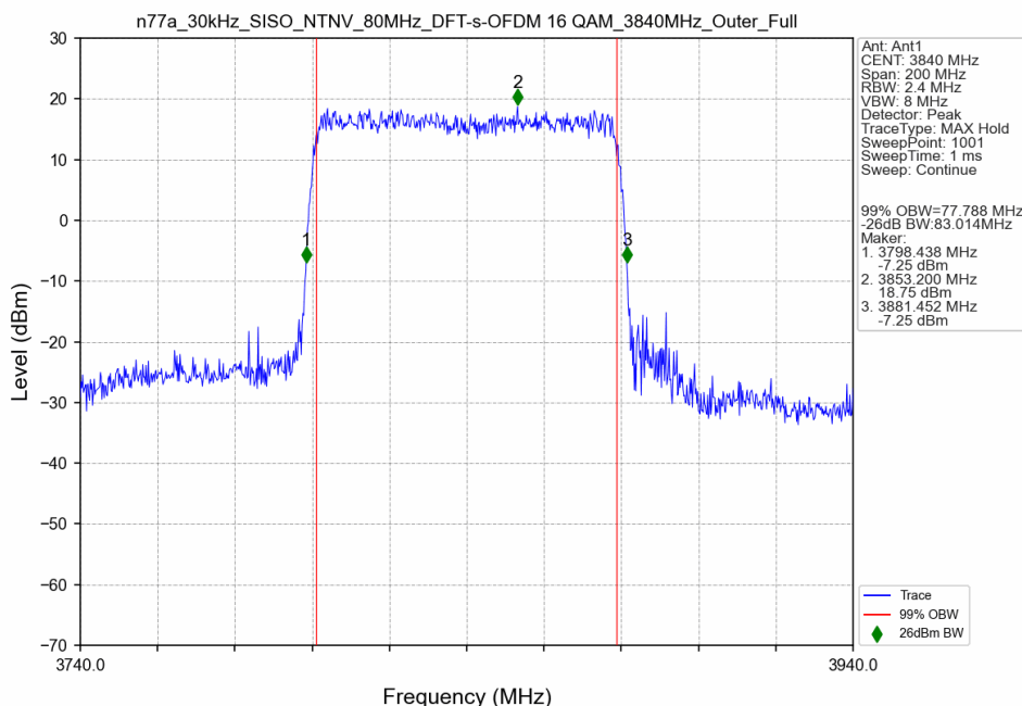
n77a_30kHz_SISO_NTNV_80MHz_DFT-s-OFDM 16 QAM_3840MHz_Outer_Full
