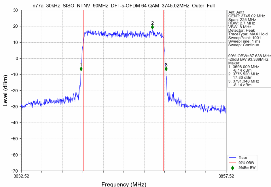
n77a_30kHz_SISO_NTNV_90MHz_DFT-s-OFDM 64 QAM_3745.02MHz_Outer_Full
