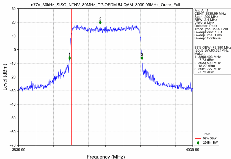
n77a_30kHz_SISO_NTNV_80MHz_CP-OFDM 64 QAM_3939.99MHz_Outer_Full
