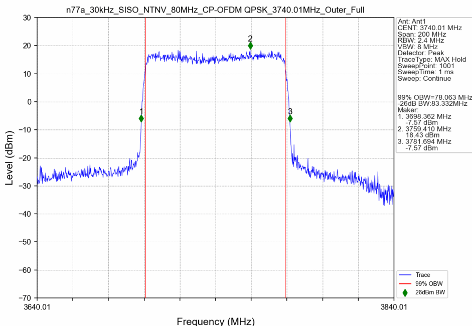
n77a_30kHz_SISO_NTNV_80MHz_CP-OFDM QPSK_3740.01MHz_Outer_Full
