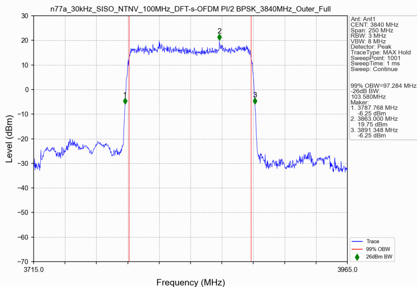
n77a_30kHz_SISO_NTNV_100MHz_DFT-s-OFDM PI/2 BPSK_3840MHz_Outer_Full
