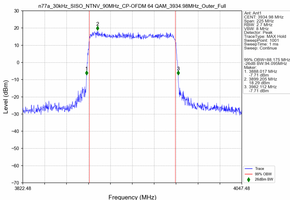
n77a_30kHz_SISO_NTNV_90MHz_CP-OFDM 64 QAM_3934.98MHz_Outer_Full
