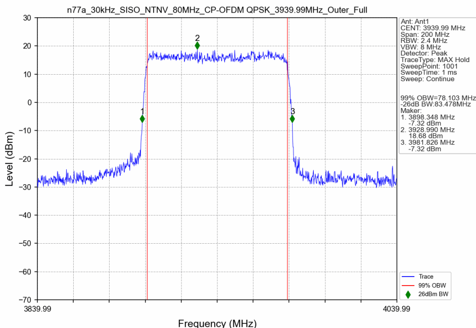
n77a_30kHz_SISO_NTNV_80MHz_CP-OFDM QPSK_3939.99MHz_Outer_Full
