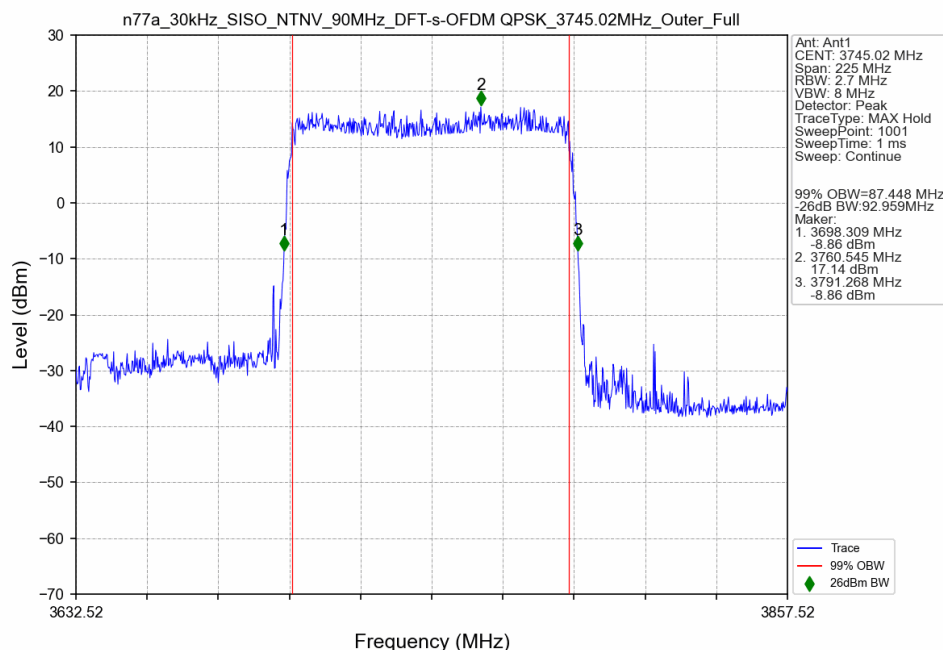
n77a_30kHz_SISO_NTNV_90MHz_DFT-s-OFDM QPSK_3745.02MHz_Outer_Full
