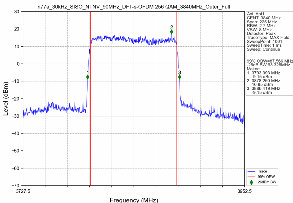
n77a_30kHz_SISO_NTNV_90MHz_DFT-s-OFDM 256 QAM_3840MHz_Outer_Full
