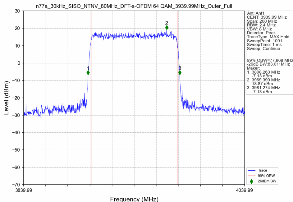
n77a_30kHz_SISO_NTNV_80MHz_DFT-s-OFDM 64 QAM_3939.99MHz_Outer_Full
