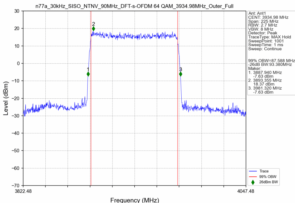
n77a_30kHz_SISO_NTNV_90MHz_DFT-s-OFDM 64 QAM_3934.98MHz_Outer_Full
