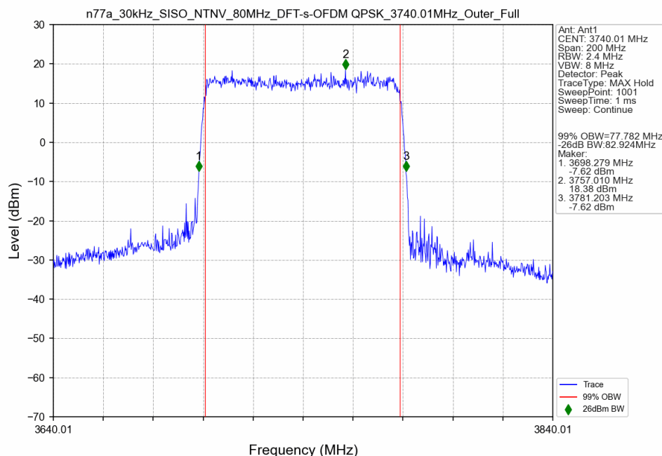
n77a_30kHz_SISO_NTNV_80MHz_DFT-s-OFDM QPSK_3740.01MHz_Outer_Full
