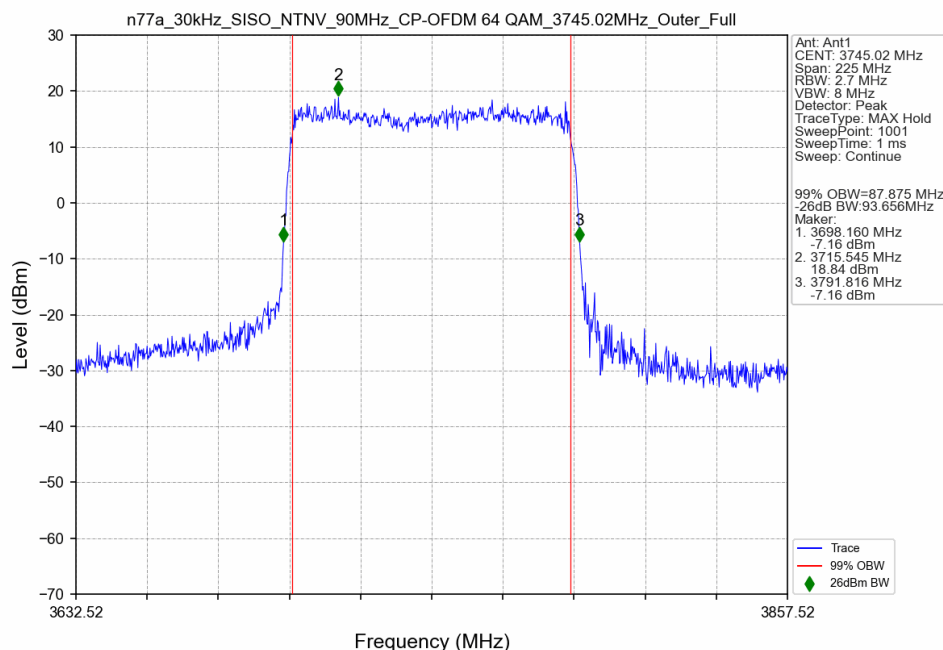
n77a_30kHz_SISO_NTNV_90MHz_CP-OFDM 64 QAM_3745.02MHz_Outer_Full
