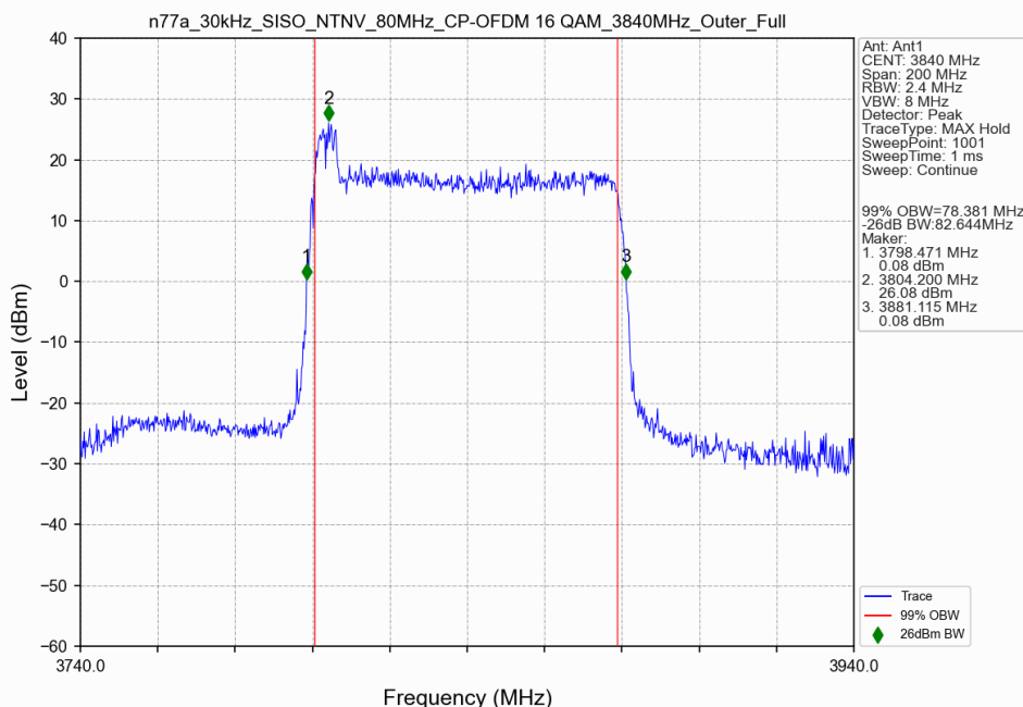
n77a_30kHz_SISO_NTNV_80MHz_CP-OFDM 16 QAM_3840MHz_Outer_Full
