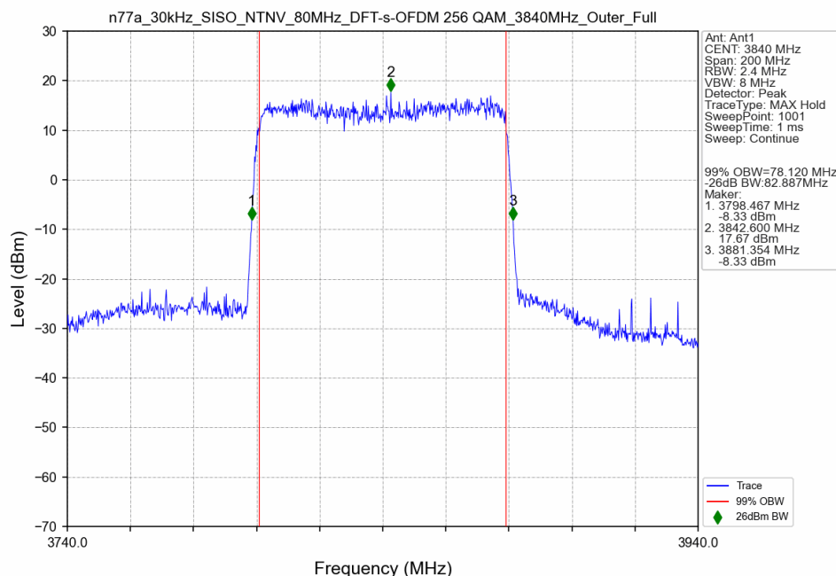
n77a_30kHz_SISO_NTNV_80MHz_DFT-s-OFDM 256 QAM_3840MHz_Outer_Full
