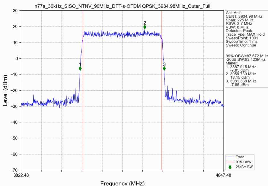
n77a_30kHz_SISO_NTNV_90MHz_DFT-s-OFDM QPSK_3934.98MHz_Outer_Full
