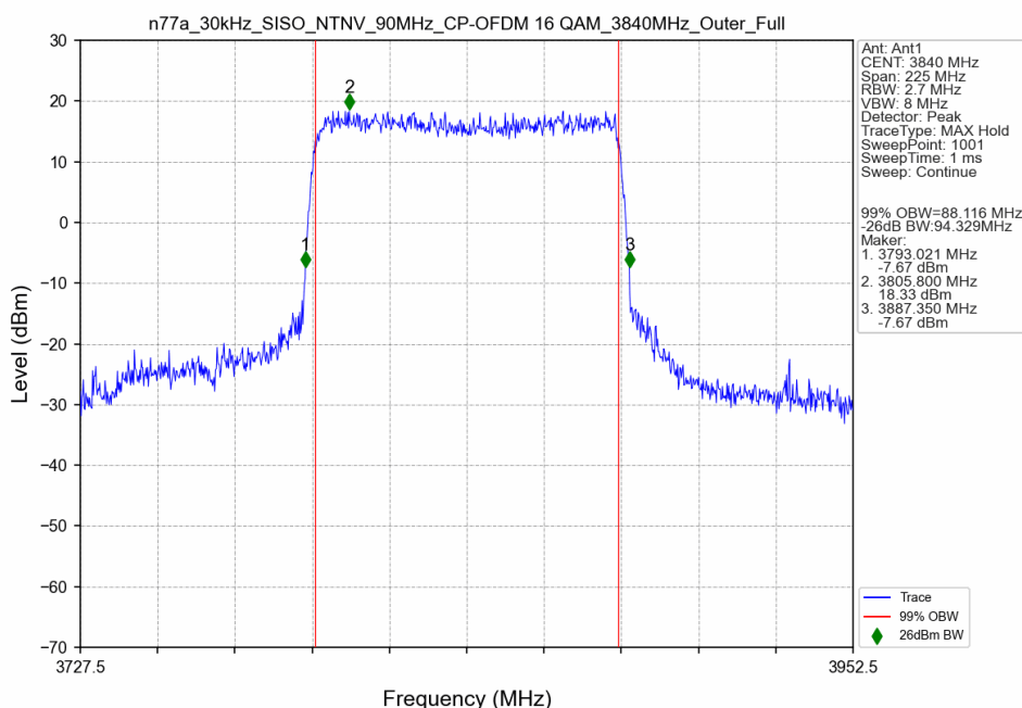
n77a_30kHz_SISO_NTNV_90MHz_CP-OFDM 16 QAM_3840MHz_Outer_Full
