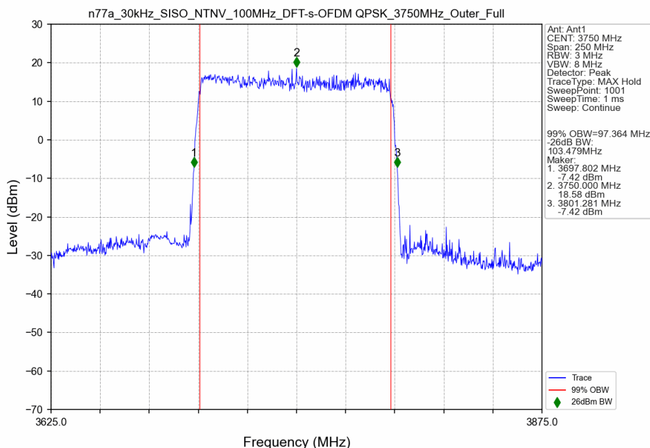
n77a_30kHz_SISO_NTNV_100MHz_DFT-s-OFDM QPSK_3750MHz_Outer_Full
