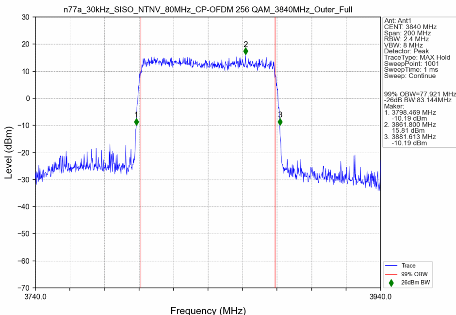
n77a_30kHz_SISO_NTNV_80MHz_CP-OFDM 256 QAM_3840MHz_Outer_Full
