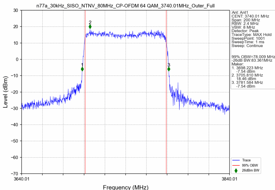
n77a_30kHz_SISO_NTNV_80MHz_CP-OFDM 64 QAM_3740.01MHz_Outer_Full
