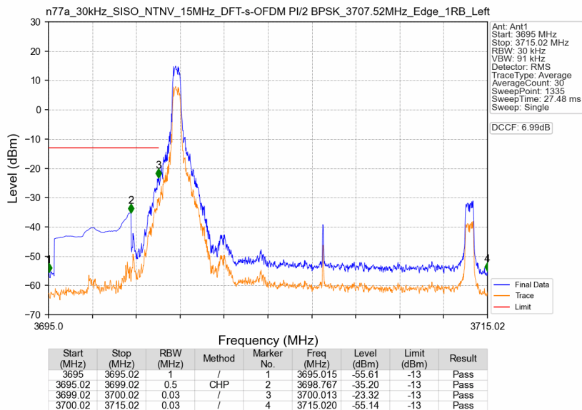
n77a_30kHz_SISO_NTNV_15MHz_DFT-s-OFDM PI/2 BPSK_3707.52MHz_Edge_1RB_Left
