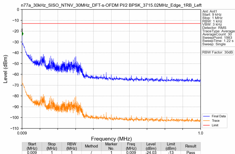
n77a_30kHz_SISO_NTNV_30MHz_DFT-s-OFDM PI/2 BPSK_3715.02MHz_Edge_1RB_Left
