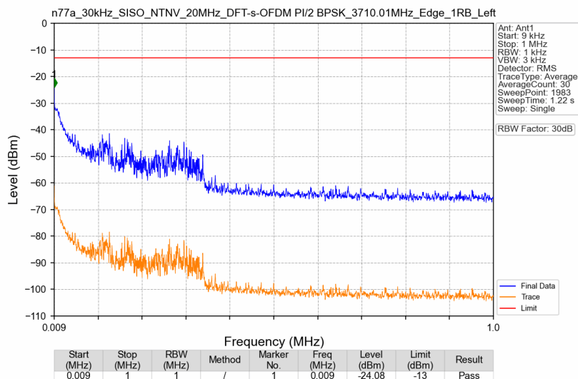
n77a_30kHz_SISO_NTNV_20MHz_DFT-s-OFDM PI/2 BPSK_3710.01MHz_Edge_1RB_Left
