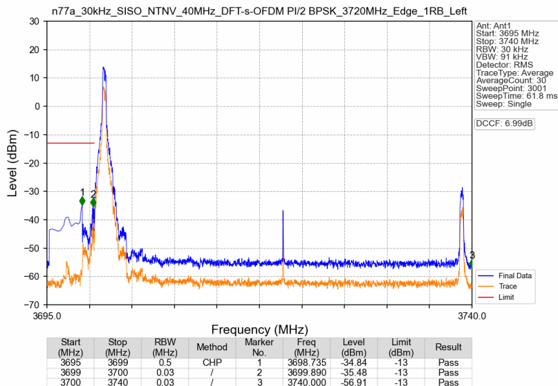
n77a_30kHz_SISO_NTNV_40MHz_DFT-s-OFDM PI/2 BPSK_3720MHz_Edge_1RB_Left
