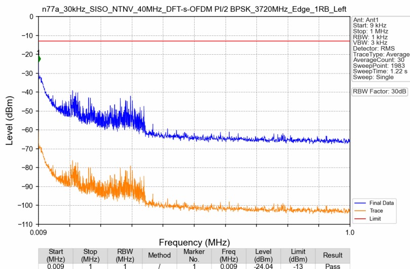
n77a_30kHz_SISO_NTNV_40MHz_DFT-s-OFDM PI/2 BPSK_3720MHz_Edge_1RB_Left
