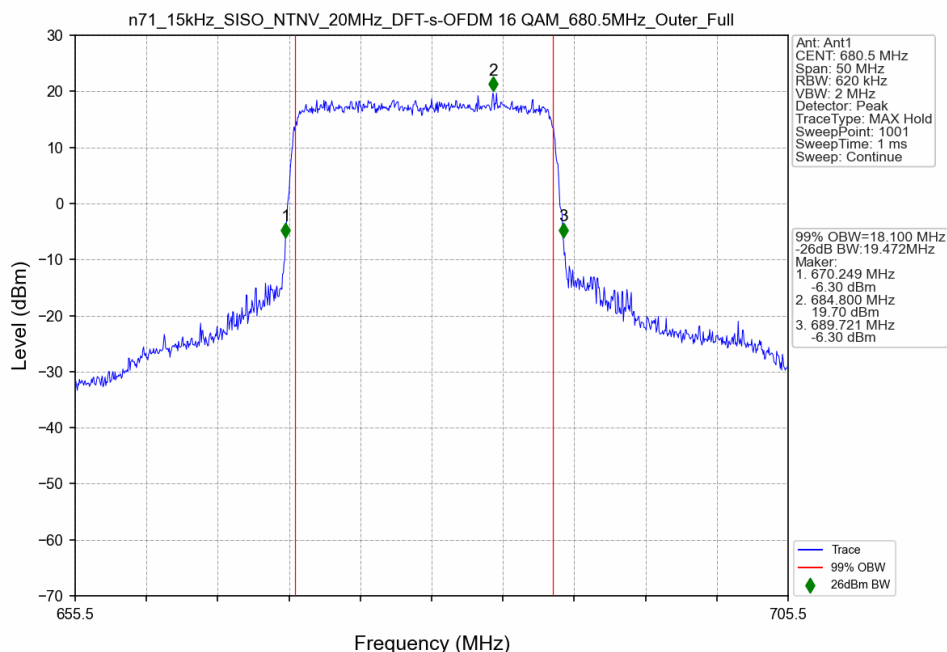
n71_15kHz_SISO_NTNV_20MHz_DFT-s-OFDM 16 QAM_680.5MHz_Outer_Full
