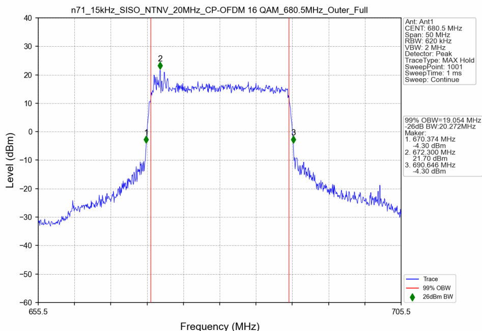
n71_15kHz_SISO_NTNV_20MHz_CP-OFDM 16 QAM_680.5MHz_Outer_Full
