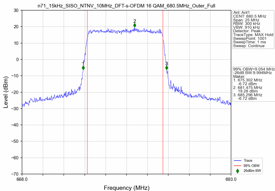
n71_15kHz_SISO_NTNV_10MHz_DFT-s-OFDM 16 QAM_680.5MHz_Outer_Full
