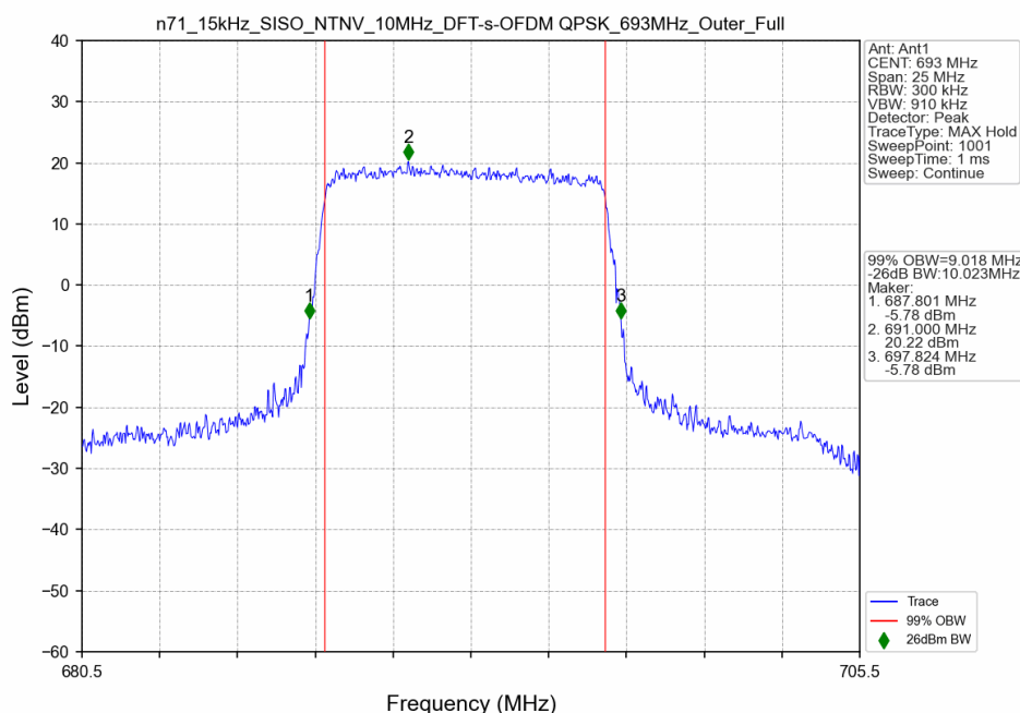
n71_15kHz_SISO_NTNV_10MHz_DFT-s-OFDM QPSK_693MHz_Outer_Full
