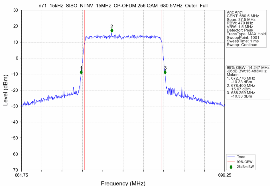
n71_15kHz_SISO_NTNV_15MHz_CP-OFDM 256 QAM_680.5MHz_Outer_Full
