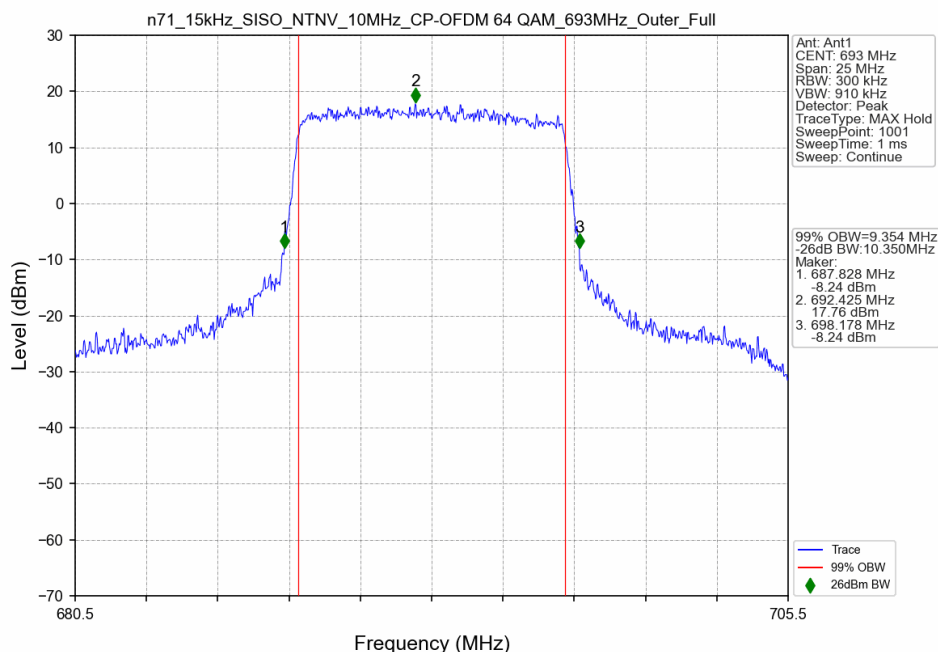
n71_15kHz_SISO_NTNV_10MHz_CP-OFDM 64 QAM_693MHz_Outer_Full
