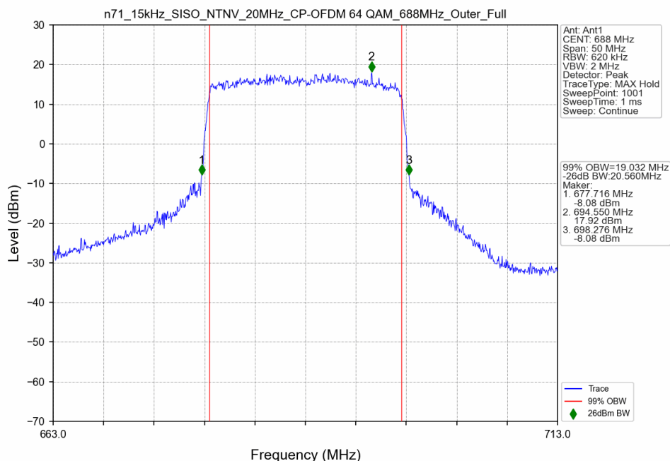
n71_15kHz_SISO_NTNV_20MHz_CP-OFDM 64 QAM_688MHz_Outer_Full
