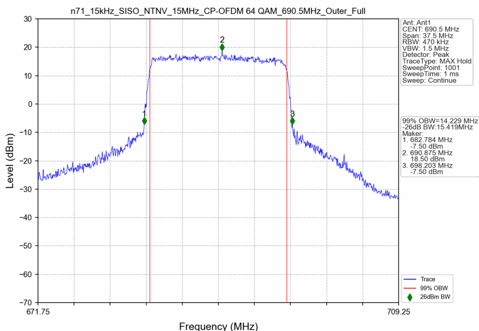
n71_15kHz_SISO_NTNV_15MHz_CP-OFDM 64 QAM_690.5MHz_Outer_Full
