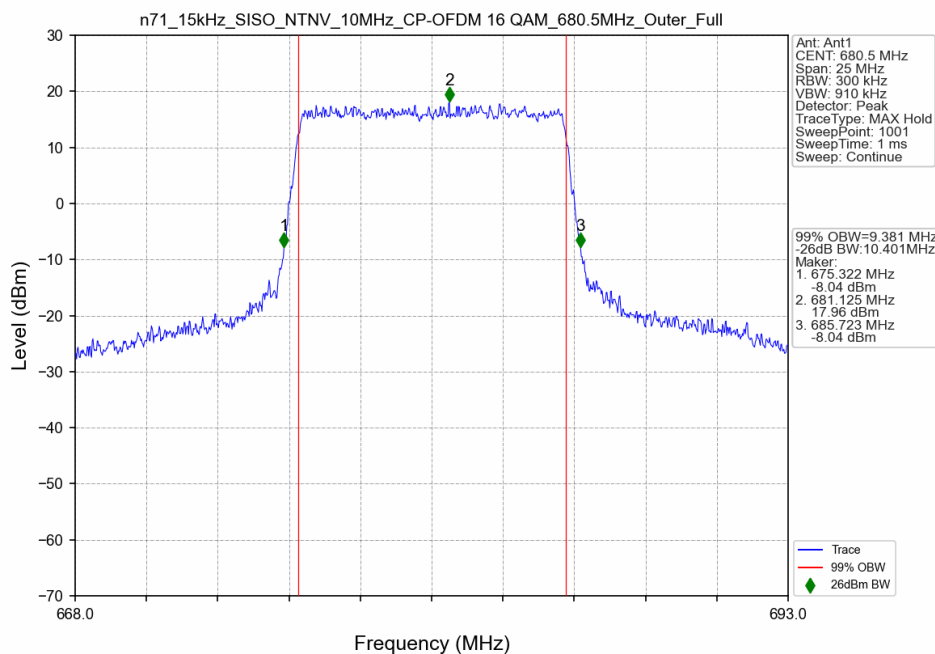
n71_15kHz_SISO_NTNV_10MHz_CP-OFDM 16 QAM_680.5MHz_Outer_Full
