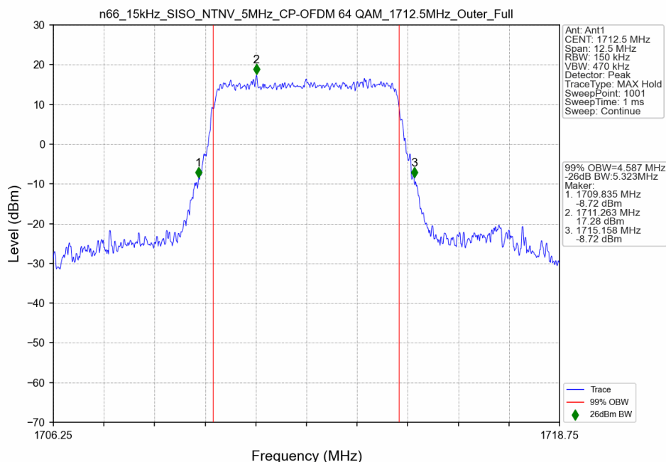
n66_15kHz_SISO_NTNV_5MHz_CP-OFDM 64 QAM_1712.5MHz_Outer_Full
