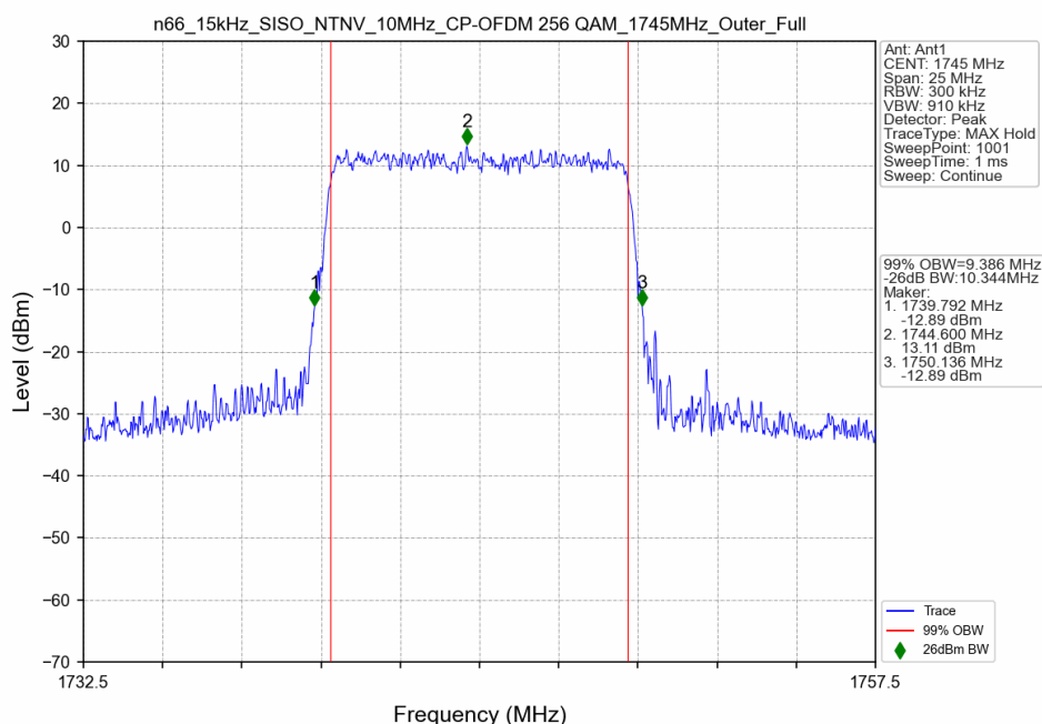
n66_15kHz_SISO_NTNV_10MHz_CP-OFDM 256 QAM_1745MHz_Outer_Full
