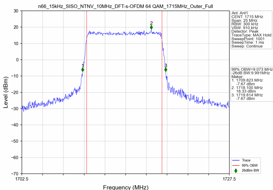
n66_15kHz_SISO_NTNV_10MHz_DFT-s-OFDM 64 QAM_1715MHz_Outer_Full
