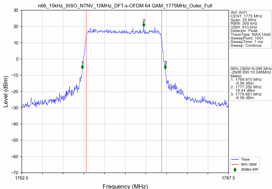
n66_15kHz_SISO_NTNV_10MHz_DFT-s-OFDM 64 QAM_1775MHz_Outer_Full
