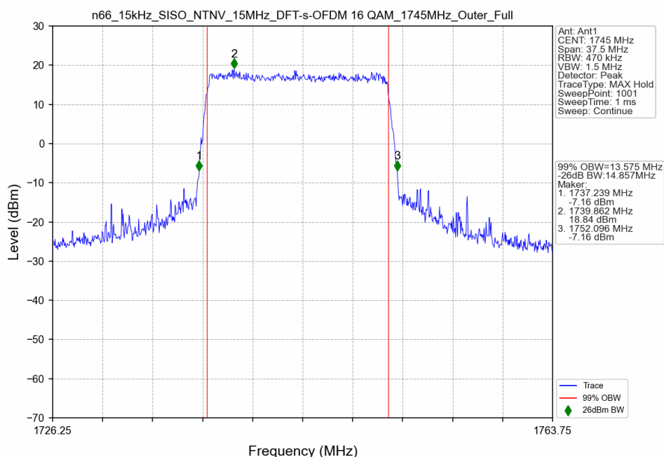
n66_15kHz_SISO_NTNV_15MHz_DFT-s-OFDM 16 QAM_1745MHz_Outer_Full
