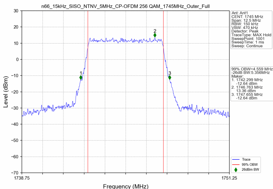
n66_15kHz_SISO_NTNV_5MHz_CP-OFDM 256 QAM_1745MHz_Outer_Full
