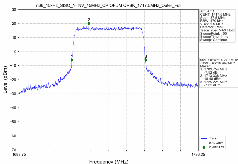
n66_15kHz_SISO_NTNV_15MHz_CP-OFDM QPSK_1717.5MHz_Outer_Full
