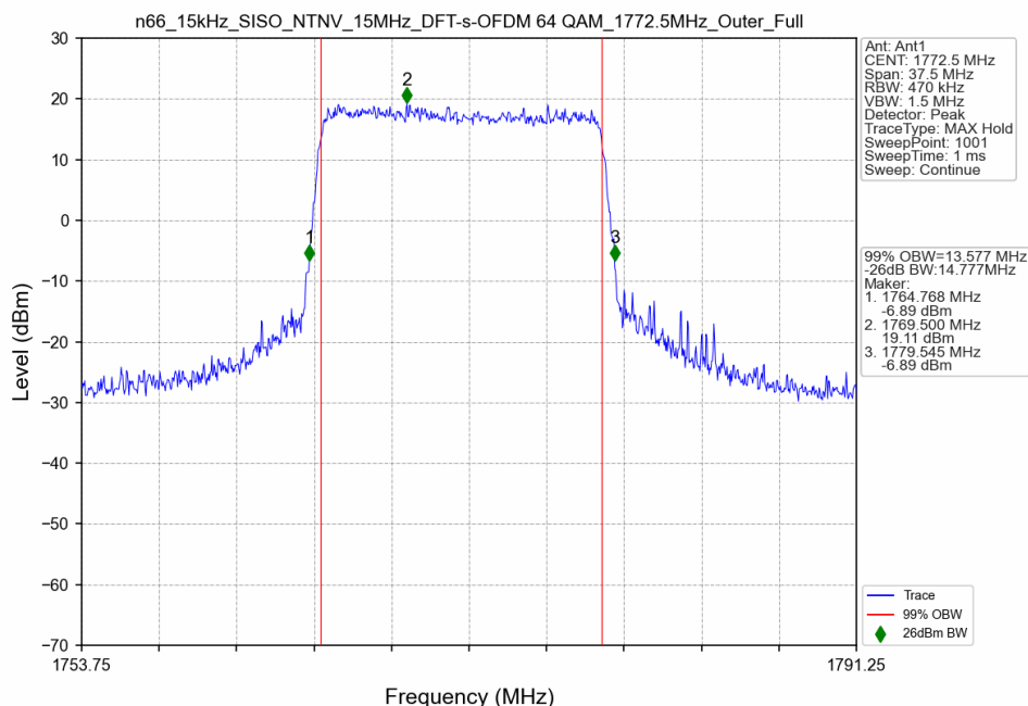
n66_15kHz_SISO_NTNV_15MHz_DFT-s-OFDM 64 QAM_1772.5MHz_Outer_Full
