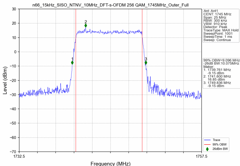
n66_15kHz_SISO_NTNV_10MHz_DFT-s-OFDM 256 QAM_1745MHz_Outer_Full
