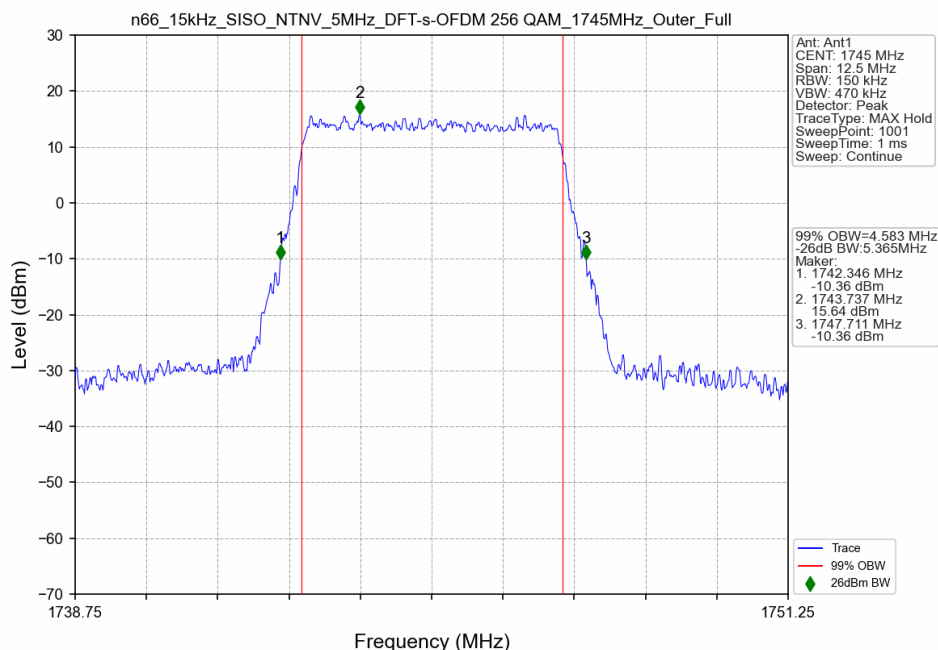
n66_15kHz_SISO_NTNV_5MHz_DFT-s-OFDM 256 QAM_1745MHz_Outer_Full
