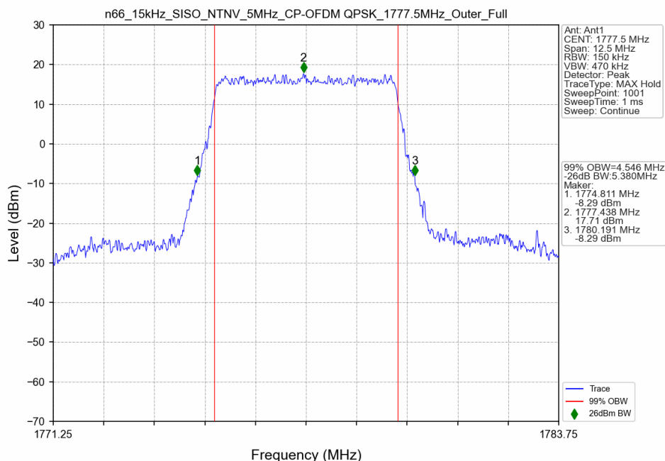
n66_15kHz_SISO_NTNV_5MHz_CP-OFDM QPSK_1777.5MHz_Outer_Full
