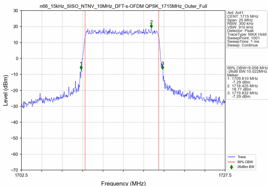
n66_15kHz_SISO_NTNV_10MHz_DFT-s-OFDM QPSK_1715MHz_Outer_Full
