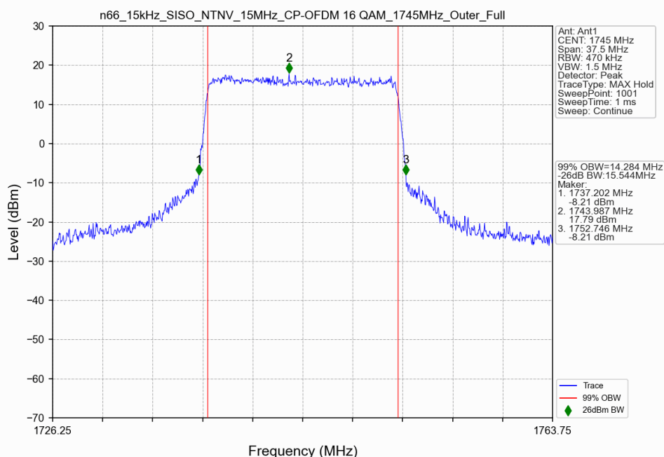
n66_15kHz_SISO_NTNV_15MHz_CP-OFDM 16 QAM_1745MHz_Outer_Full
