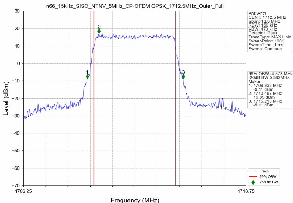
n66_15kHz_SISO_NTNV_5MHz_CP-OFDM QPSK_1712.5MHz_Outer_Full
