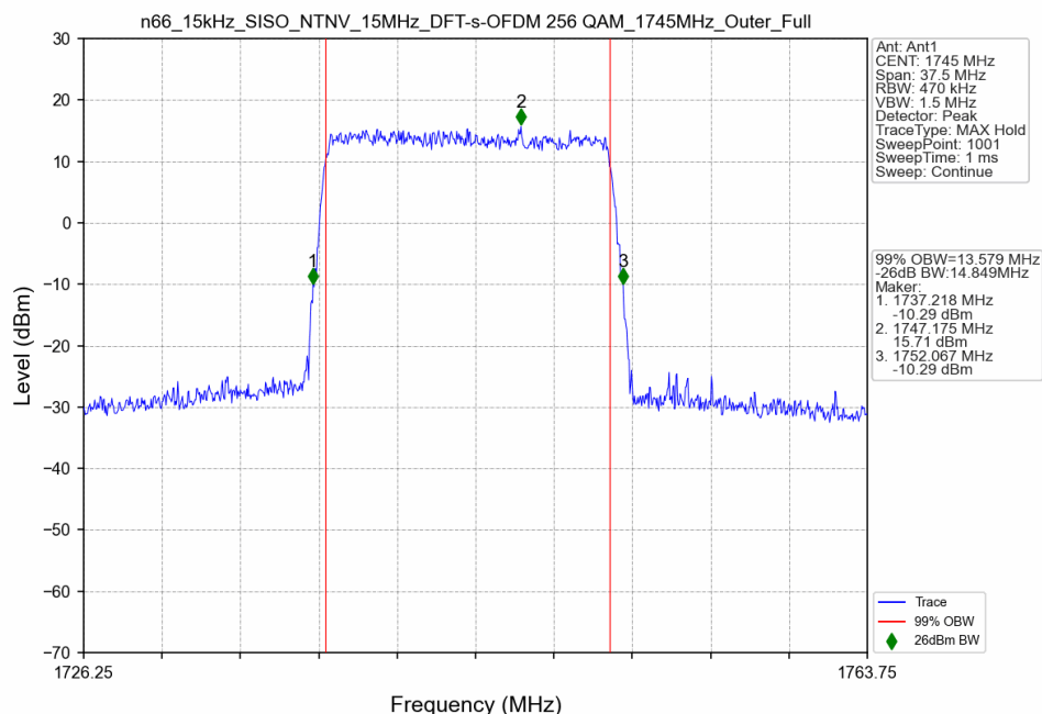
n66_15kHz_SISO_NTNV_15MHz_DFT-s-OFDM 256 QAM_1745MHz_Outer_Full
