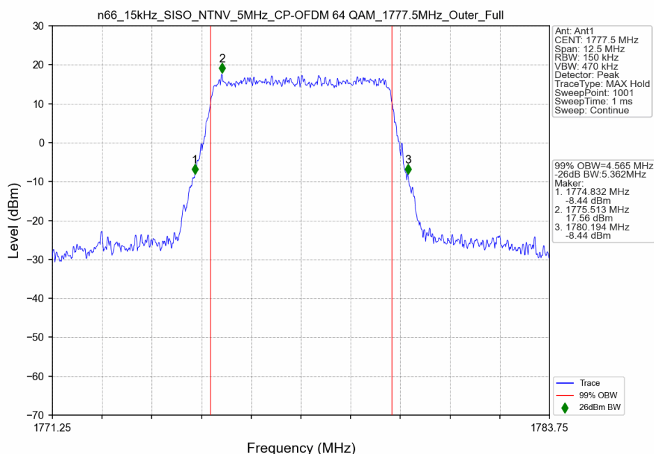
n66_15kHz_SISO_NTNV_5MHz_CP-OFDM 64 QAM_1777.5MHz_Outer_Full
