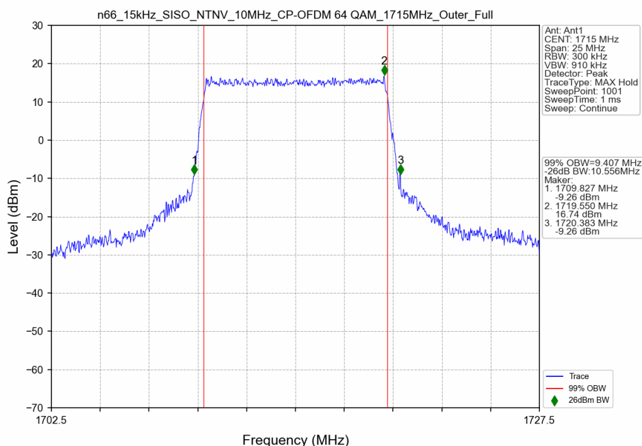
n66_15kHz_SISO_NTNV_10MHz_CP-OFDM 64 QAM_1715MHz_Outer_Full
