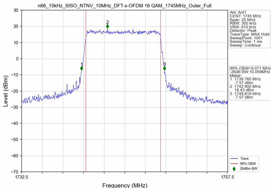
n66_15kHz_SISO_NTNV_10MHz_DFT-s-OFDM 16 QAM_1745MHz_Outer_Full
