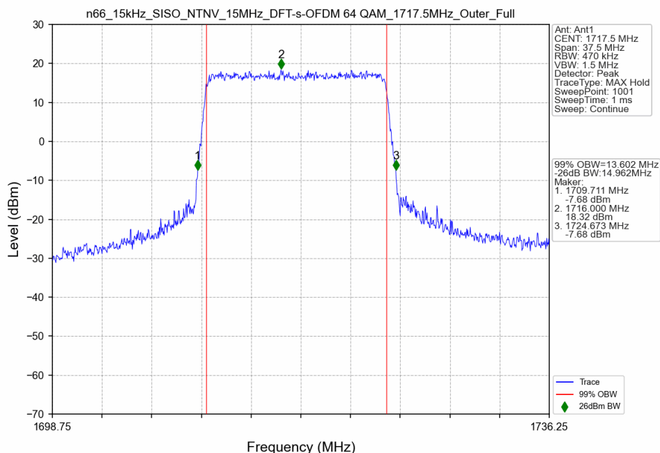
n66_15kHz_SISO_NTNV_15MHz_DFT-s-OFDM 64 QAM_1717.5MHz_Outer_Full
