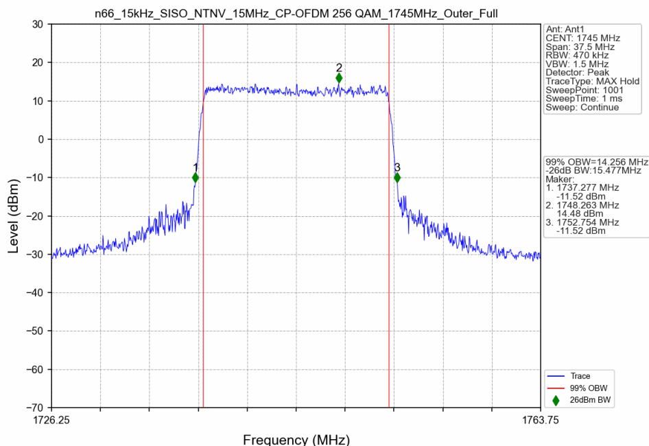
n66_15kHz_SISO_NTNV_15MHz_CP-OFDM 256 QAM_1745MHz_Outer_Full
