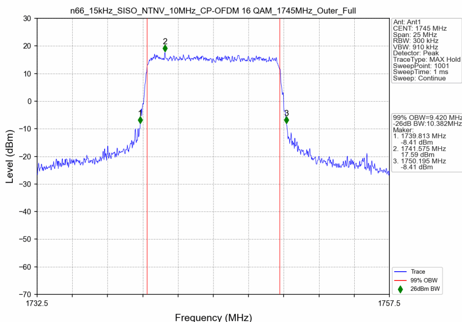
n66_15kHz_SISO_NTNV_10MHz_CP-OFDM 16 QAM_1745MHz_Outer_Full
