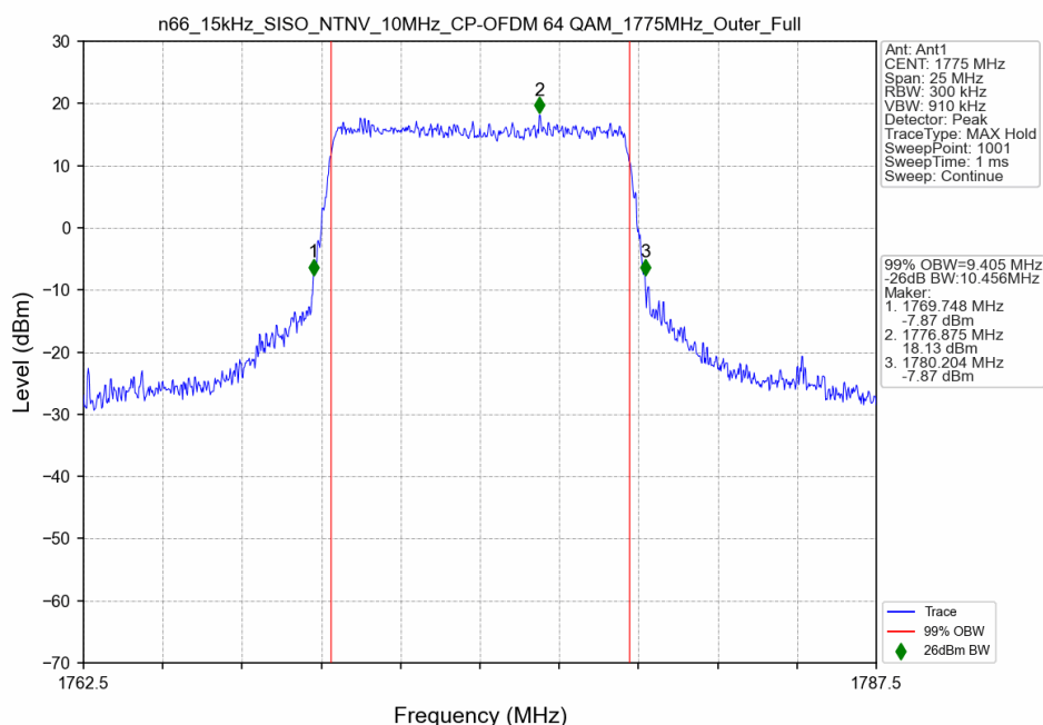
n66_15kHz_SISO_NTNV_10MHz_CP-OFDM 64 QAM_1775MHz_Outer_Full
