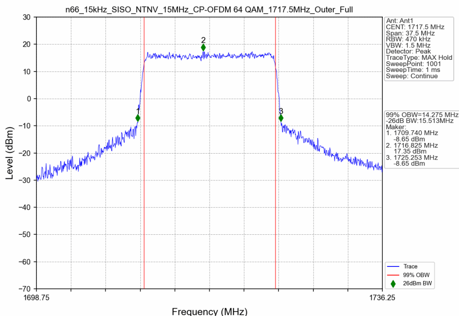
n66_15kHz_SISO_NTNV_15MHz_CP-OFDM 64 QAM_1717.5MHz_Outer_Full
