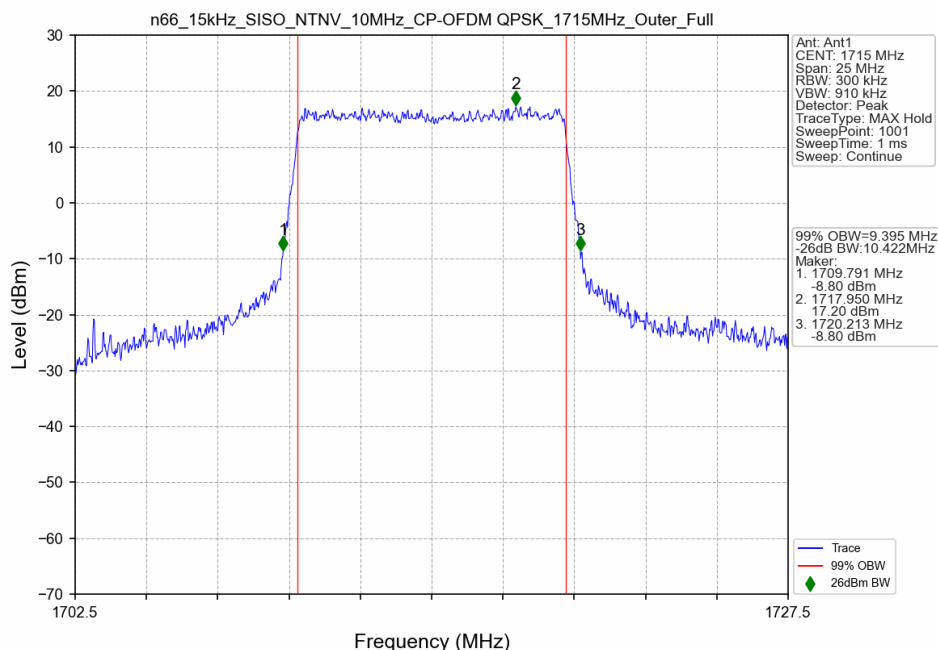
n66_15kHz_SISO_NTNV_10MHz_CP-OFDM QPSK_1715MHz_Outer_Full
