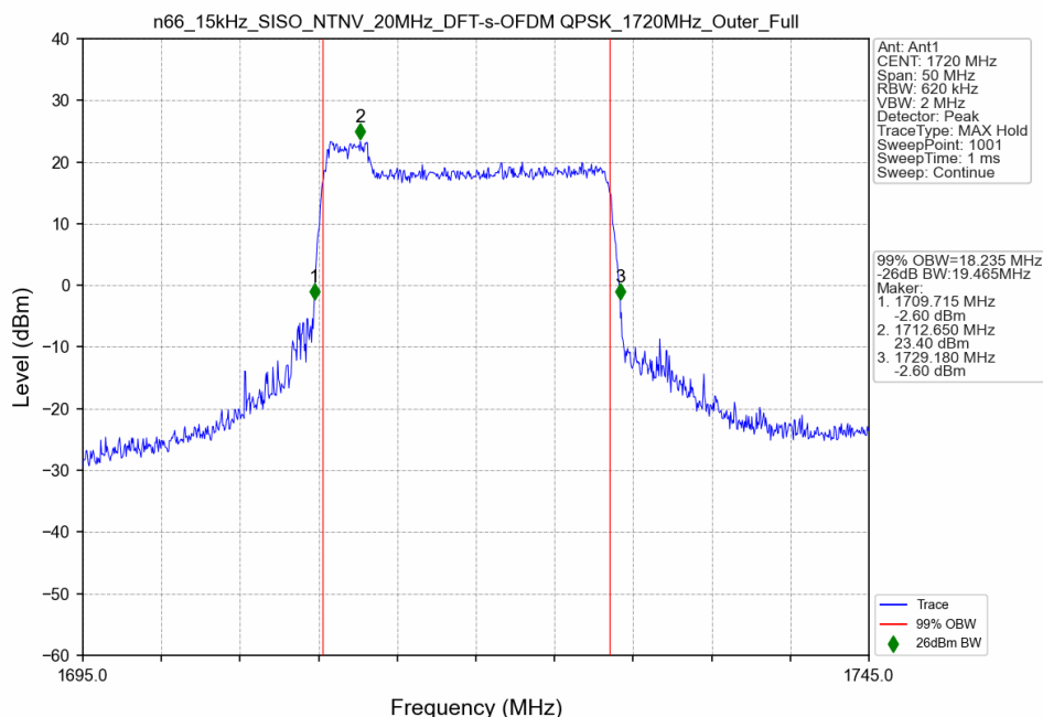
n66_15kHz_SISO_NTNV_20MHz_DFT-s-OFDM QPSK_1720MHz_Outer_Full
