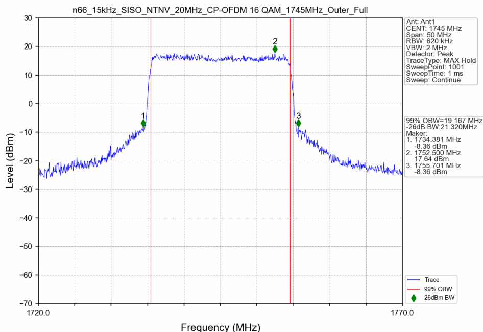
n66_15kHz_SISO_NTNV_20MHz_CP-OFDM 16 QAM_1745MHz_Outer_Full
