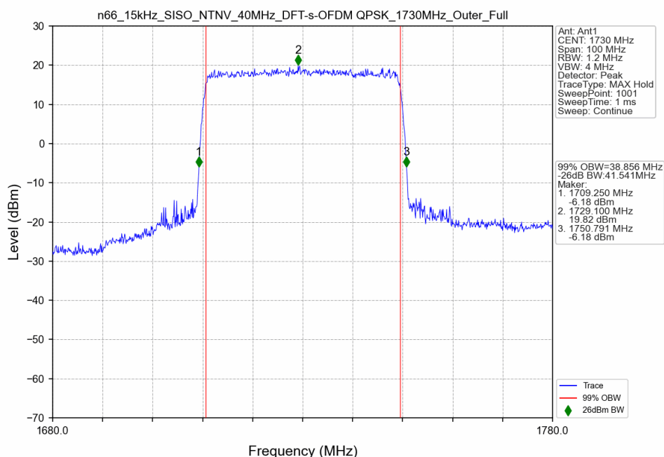
n66_15kHz_SISO_NTNV_40MHz_DFT-s-OFDM QPSK_1730MHz_Outer_Full
