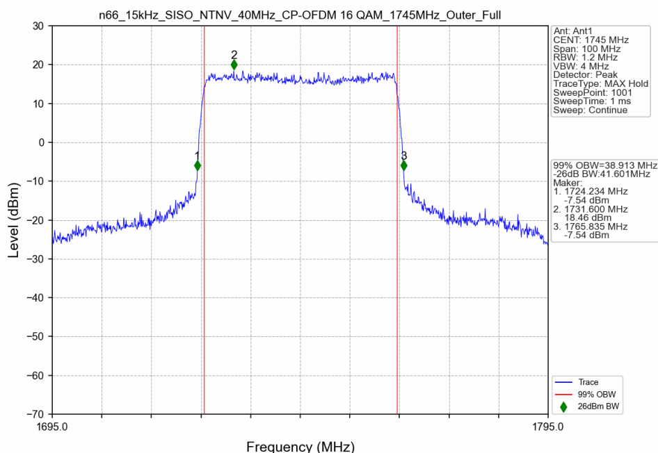
n66_15kHz_SISO_NTNV_40MHz_CP-OFDM 16 QAM_1745MHz_Outer_Full
