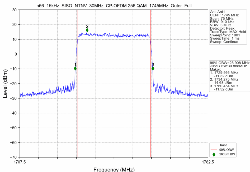
n66_15kHz_SISO_NTNV_30MHz_CP-OFDM 256 QAM_1745MHz_Outer_Full
