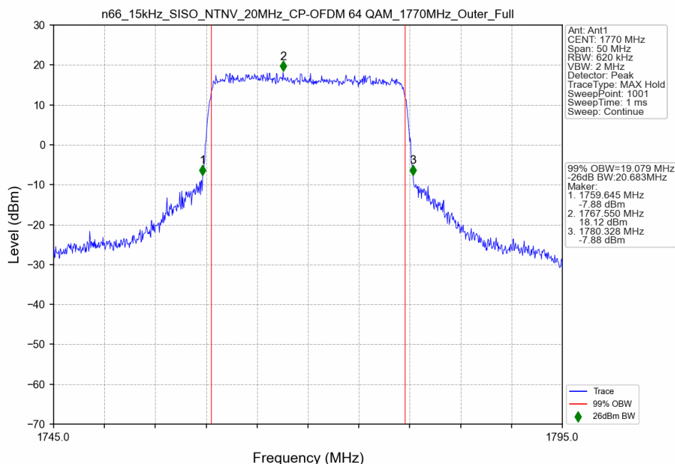
n66_15kHz_SISO_NTNV_20MHz_CP-OFDM 64 QAM_1770MHz_Outer_Full
