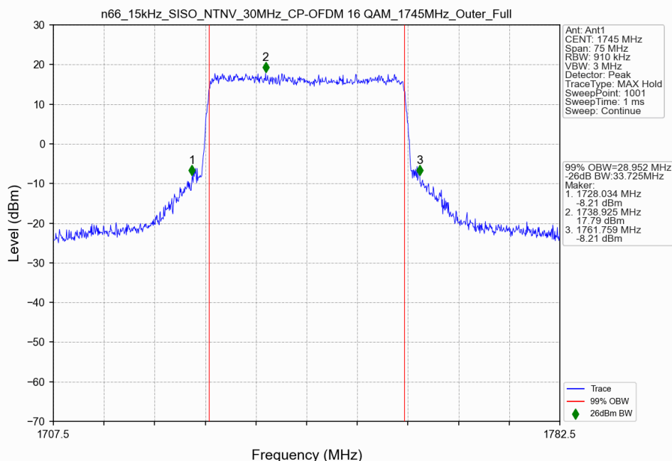
n66_15kHz_SISO_NTNV_30MHz_CP-OFDM 16 QAM_1745MHz_Outer_Full
