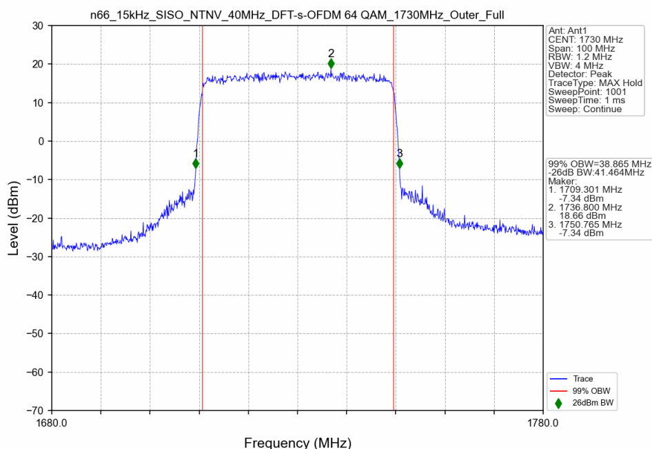
n66_15kHz_SISO_NTNV_40MHz_DFT-s-OFDM 64 QAM_1730MHz_Outer_Full
