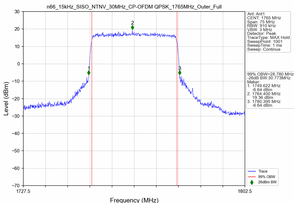
n66_15kHz_SISO_NTNV_30MHz_CP-OFDM QPSK_1765MHz_Outer_Full
