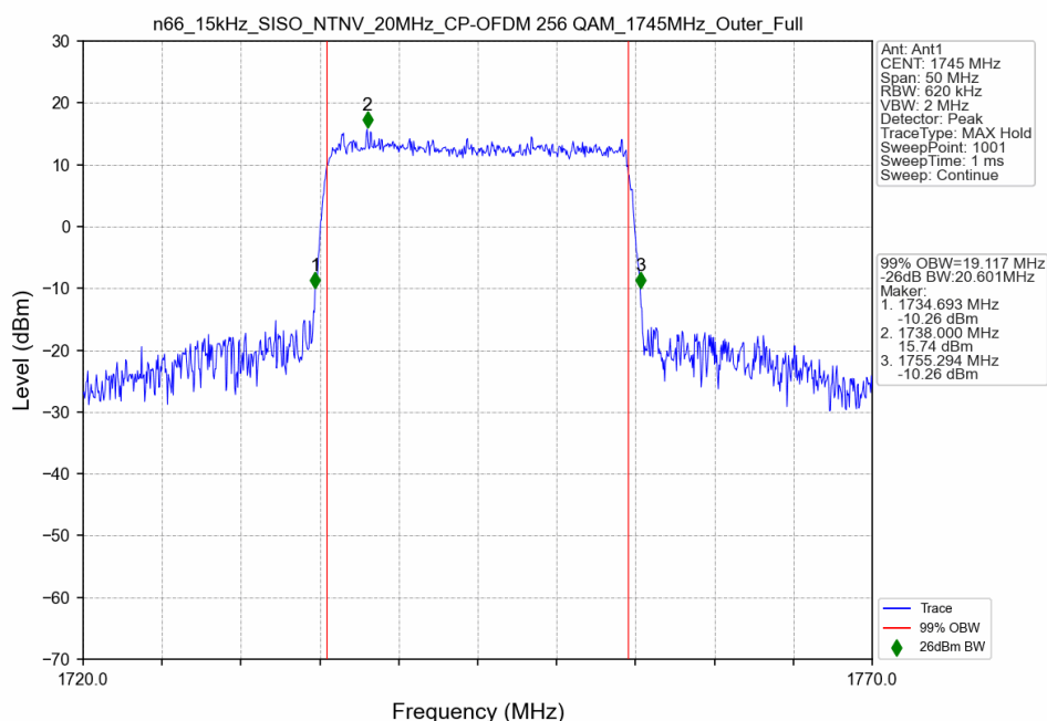
n66_15kHz_SISO_NTNV_20MHz_CP-OFDM 256 QAM_1745MHz_Outer_Full
