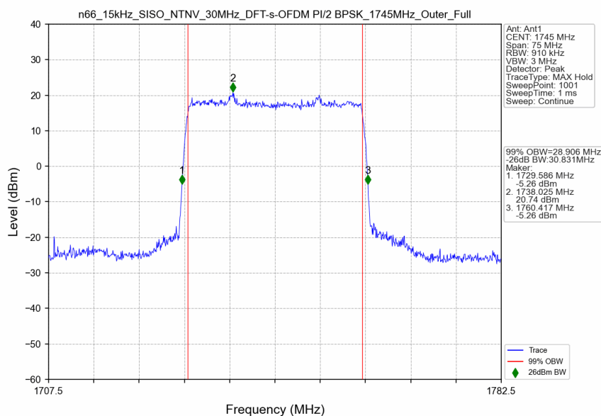
n66_15kHz_SISO_NTNV_30MHz_DFT-s-OFDM PI/2 BPSK_1745MHz_Outer_Full
