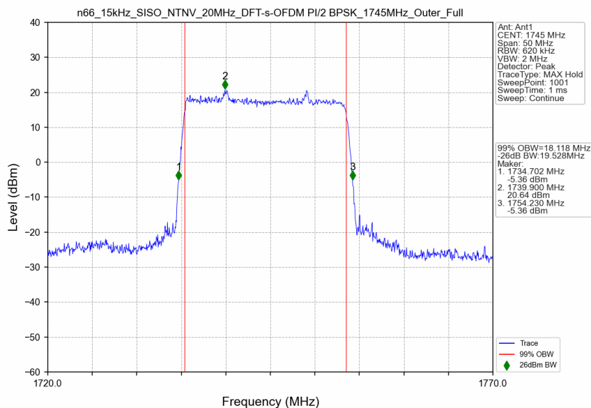
n66_15kHz_SISO_NTNV_20MHz_DFT-s-OFDM PI/2 BPSK_1745MHz_Outer_Full
