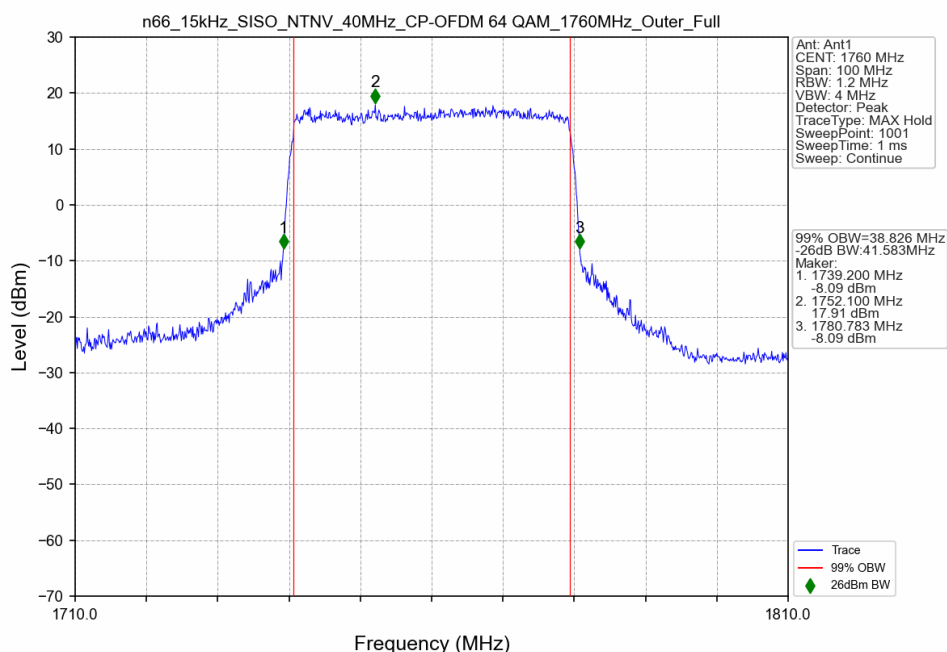
n66_15kHz_SISO_NTNV_40MHz_CP-OFDM 64 QAM_1760MHz_Outer_Full
