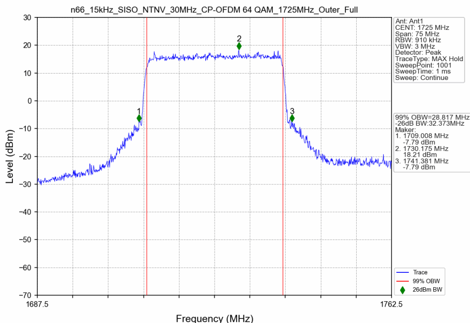
n66_15kHz_SISO_NTNV_30MHz_CP-OFDM 64 QAM_1725MHz_Outer_Full
