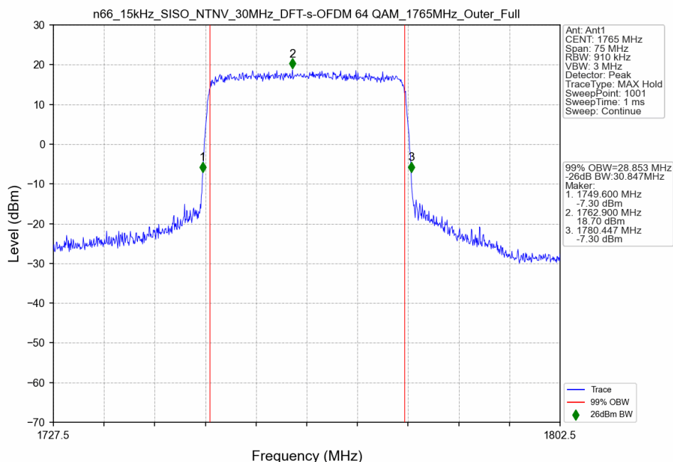
n66_15kHz_SISO_NTNV_30MHz_DFT-s-OFDM 64 QAM_1765MHz_Outer_Full
