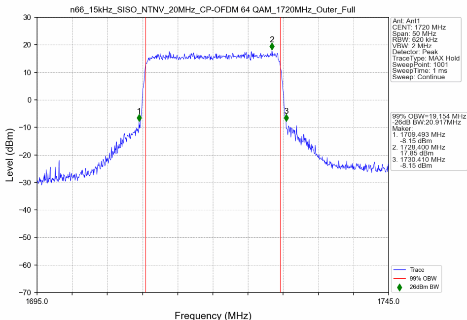
n66_15kHz_SISO_NTNV_20MHz_CP-OFDM 64 QAM_1720MHz_Outer_Full
