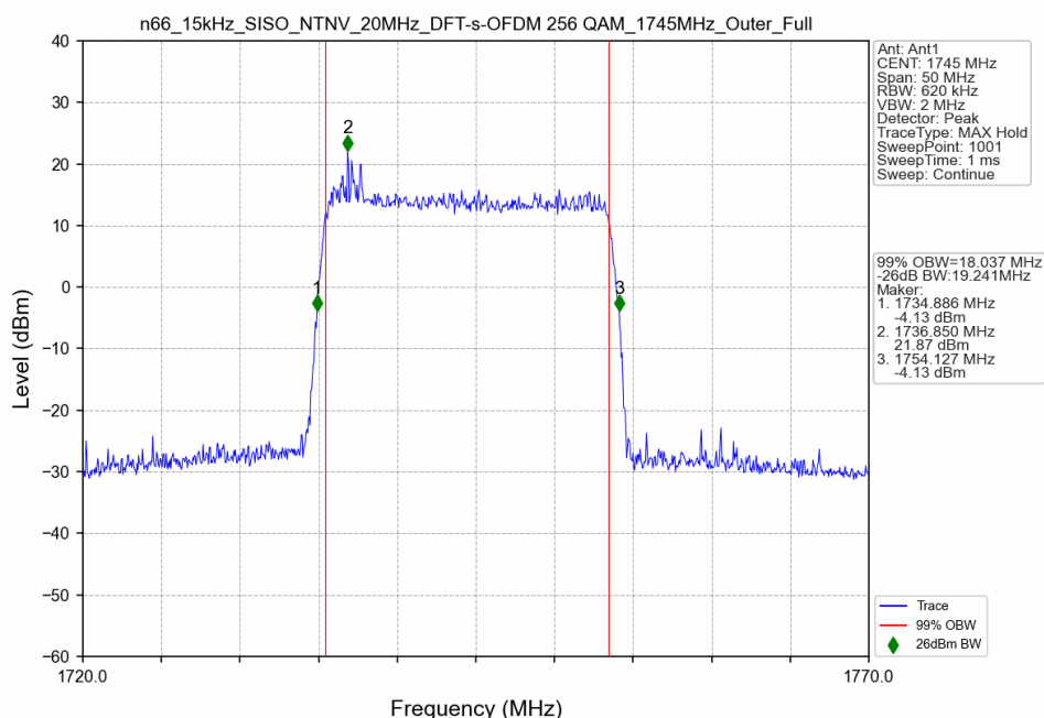
n66_15kHz_SISO_NTNV_20MHz_DFT-s-OFDM 256 QAM_1745MHz_Outer_Full
