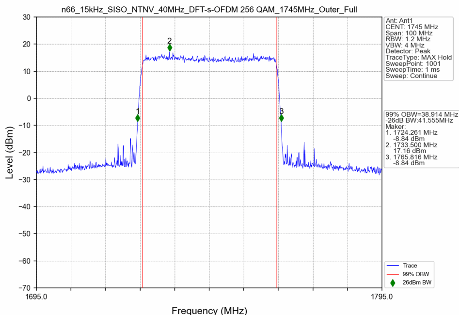
n66_15kHz_SISO_NTNV_40MHz_DFT-s-OFDM 256 QAM_1745MHz_Outer_Full
