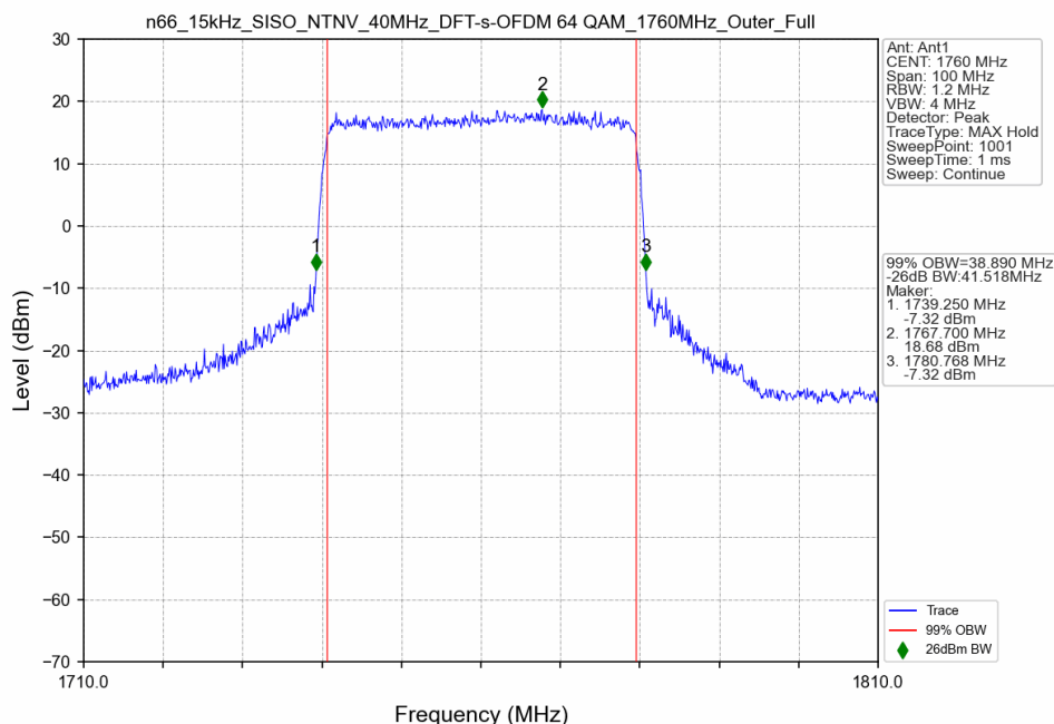
n66_15kHz_SISO_NTNV_40MHz_DFT-s-OFDM 64 QAM_1760MHz_Outer_Full
