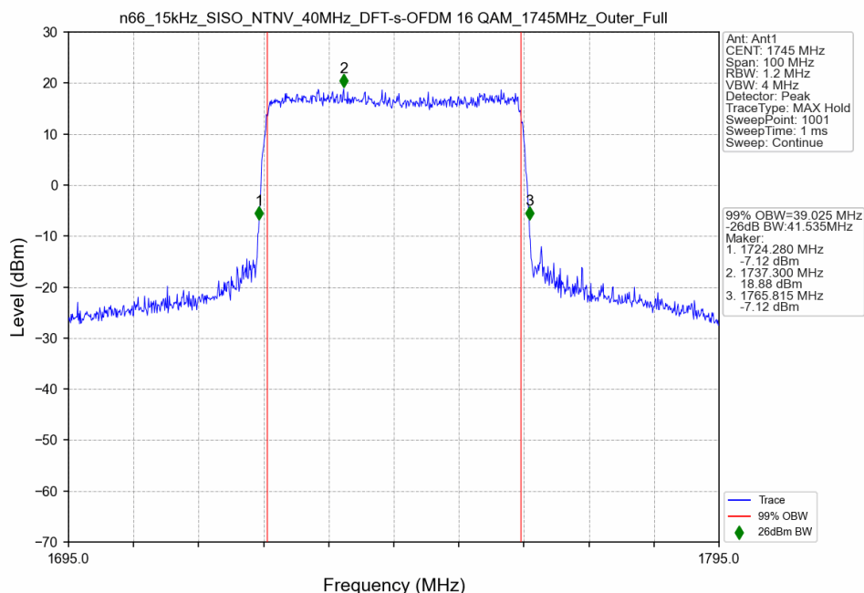
n66_15kHz_SISO_NTNV_40MHz_DFT-s-OFDM 16 QAM_1745MHz_Outer_Full
