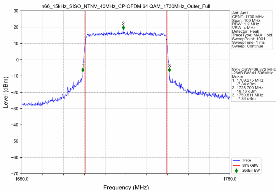
n66_15kHz_SISO_NTNV_40MHz_CP-OFDM 64 QAM_1730MHz_Outer_Full
