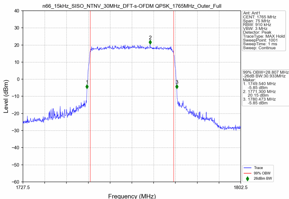
n66_15kHz_SISO_NTNV_30MHz_DFT-s-OFDM QPSK_1765MHz_Outer_Full
