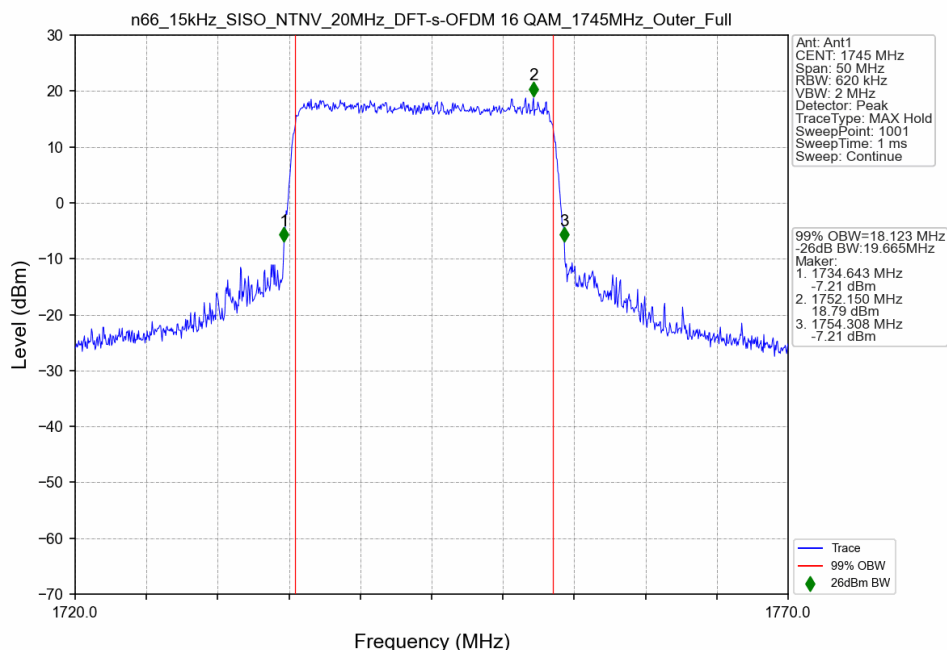
n66_15kHz_SISO_NTNV_20MHz_DFT-s-OFDM 16 QAM_1745MHz_Outer_Full
