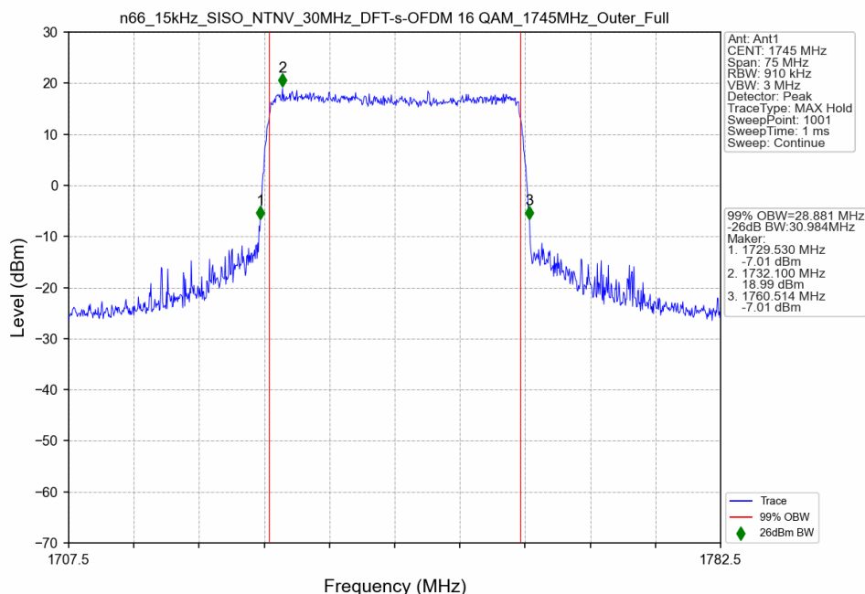
n66_15kHz_SISO_NTNV_30MHz_DFT-s-OFDM 16 QAM_1745MHz_Outer_Full
