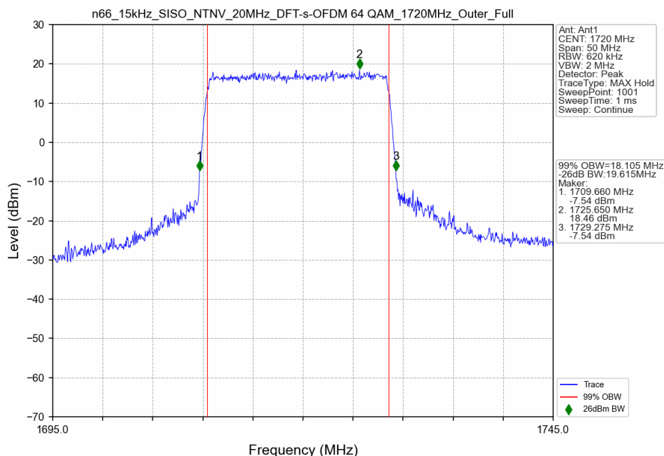
n66_15kHz_SISO_NTNV_20MHz_DFT-s-OFDM 64 QAM_1720MHz_Outer_Full
