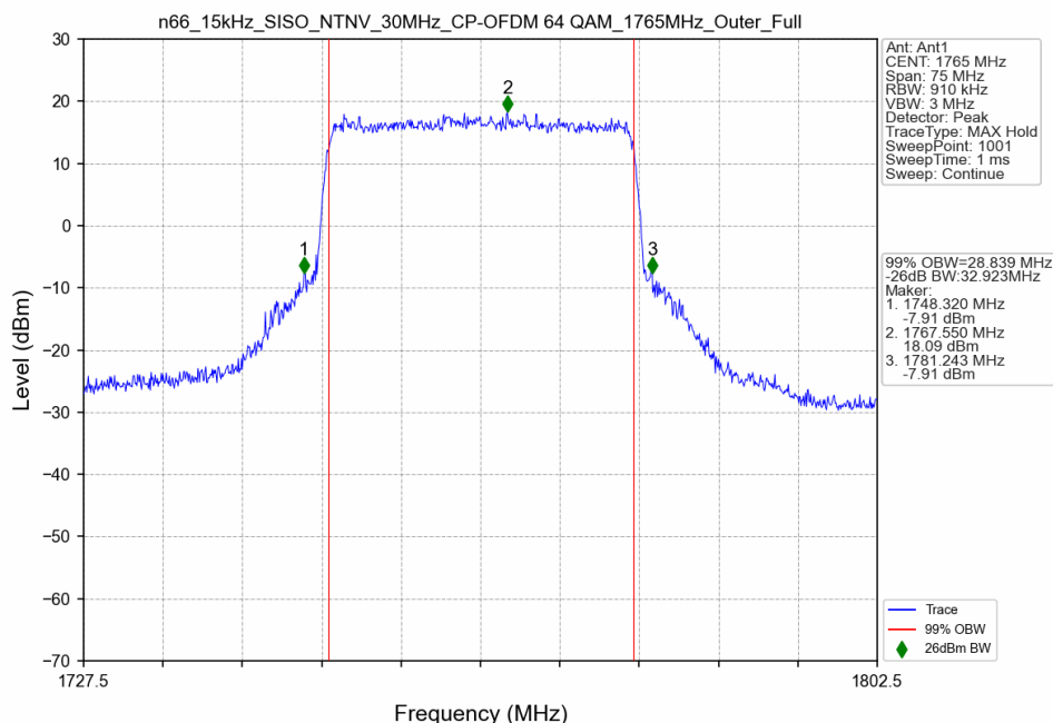
n66_15kHz_SISO_NTNV_30MHz_CP-OFDM 64 QAM_1765MHz_Outer_Full
