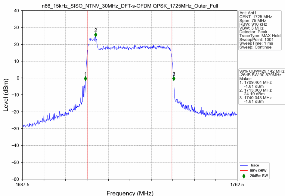
n66_15kHz_SISO_NTNV_30MHz_DFT-s-OFDM QPSK_1725MHz_Outer_Full
