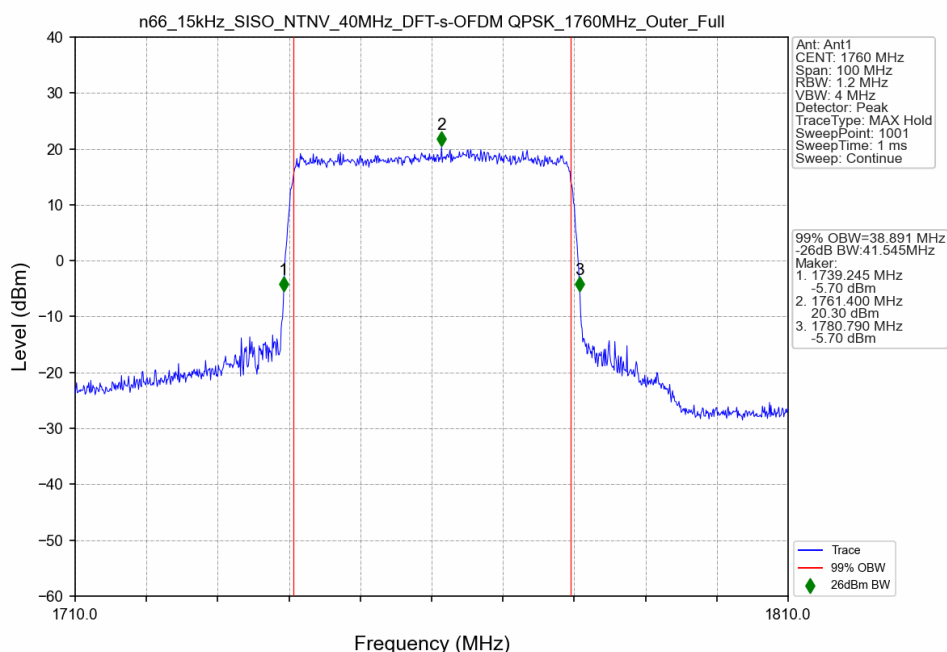
n66_15kHz_SISO_NTNV_40MHz_DFT-s-OFDM QPSK_1760MHz_Outer_Full
