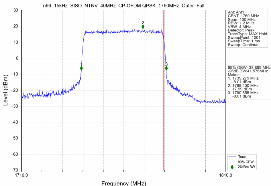
n66_15kHz_SISO_NTNV_40MHz_CP-OFDM QPSK_1760MHz_Outer_Full
