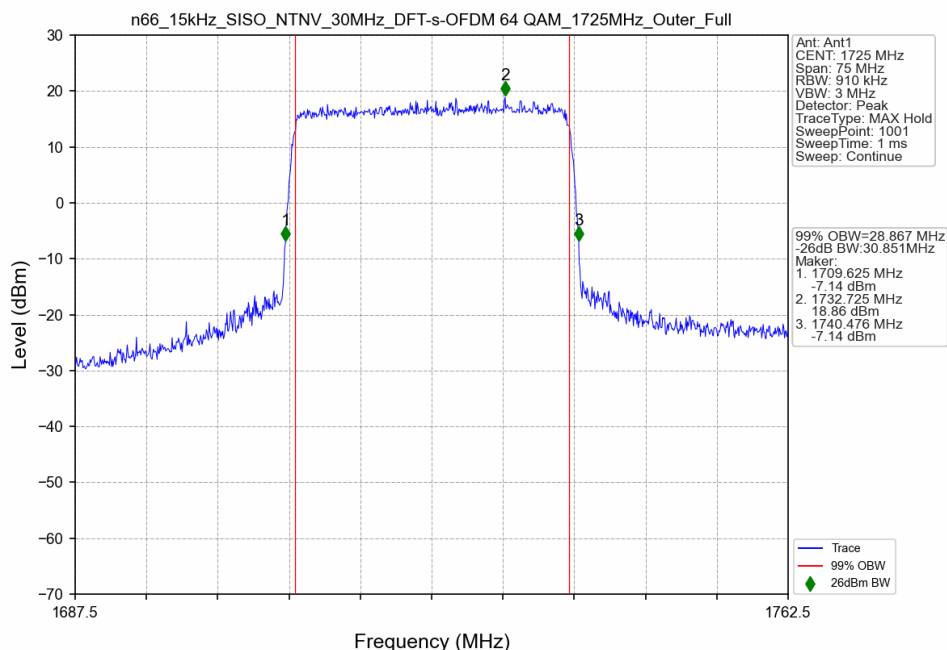
n66_15kHz_SISO_NTNV_30MHz_DFT-s-OFDM 64 QAM_1725MHz_Outer_Full
