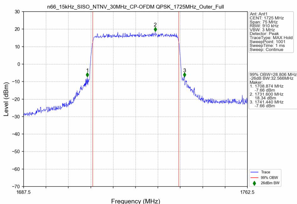
n66_15kHz_SISO_NTNV_30MHz_CP-OFDM QPSK_1725MHz_Outer_Full
