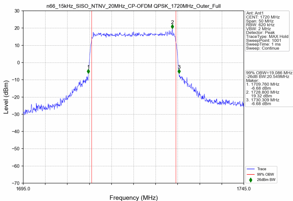
n66_15kHz_SISO_NTNV_20MHz_CP-OFDM QPSK_1720MHz_Outer_Full
