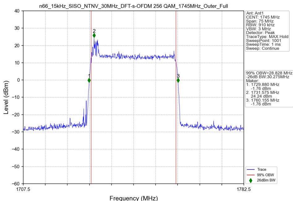
n66_15kHz_SISO_NTNV_30MHz_DFT-s-OFDM 256 QAM_1745MHz_Outer_Full
