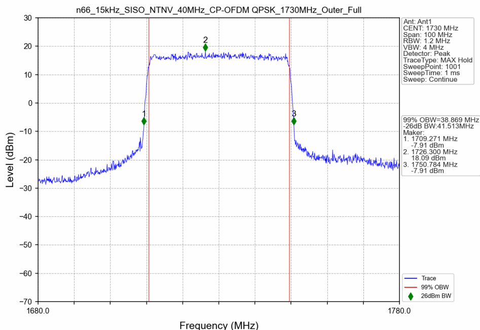
n66_15kHz_SISO_NTNV_40MHz_CP-OFDM QPSK_1730MHz_Outer_Full
