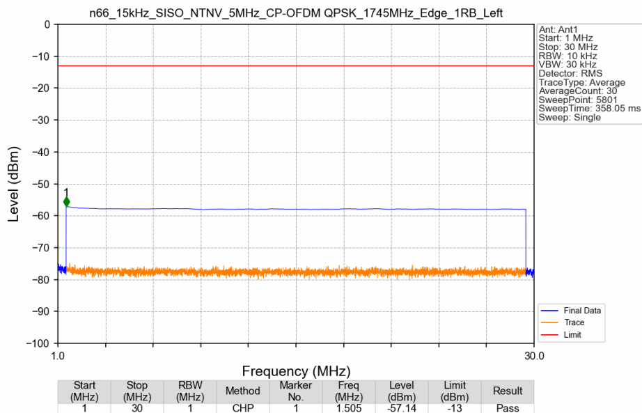
n66_15kHz_SISO_NTNV_5MHz_CP-OFDM QPSK_1745MHz_Edge_1RB_Left
