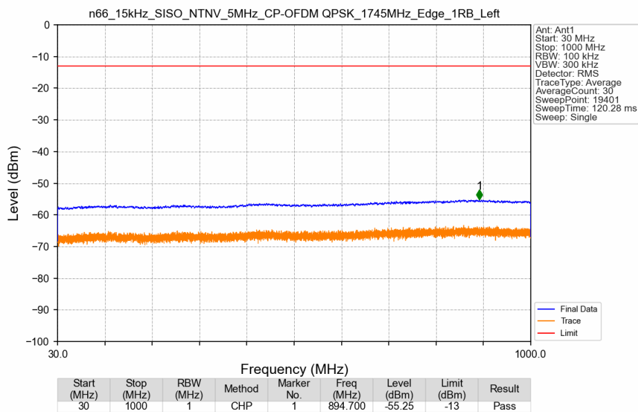
n66_15kHz_SISO_NTNV_5MHz_CP-OFDM QPSK_1745MHz_Edge_1RB_Left
