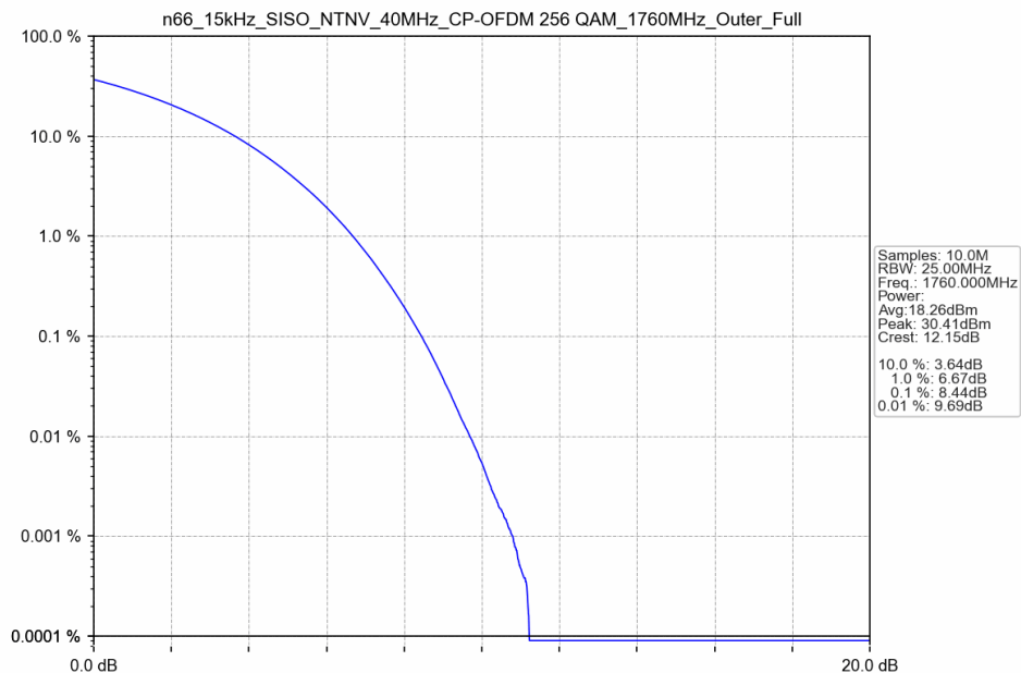
n66_15kHz_SISO_NTNV_40MHz_CP-OFDM 256 QAM_1760MHz_Outer_Full
