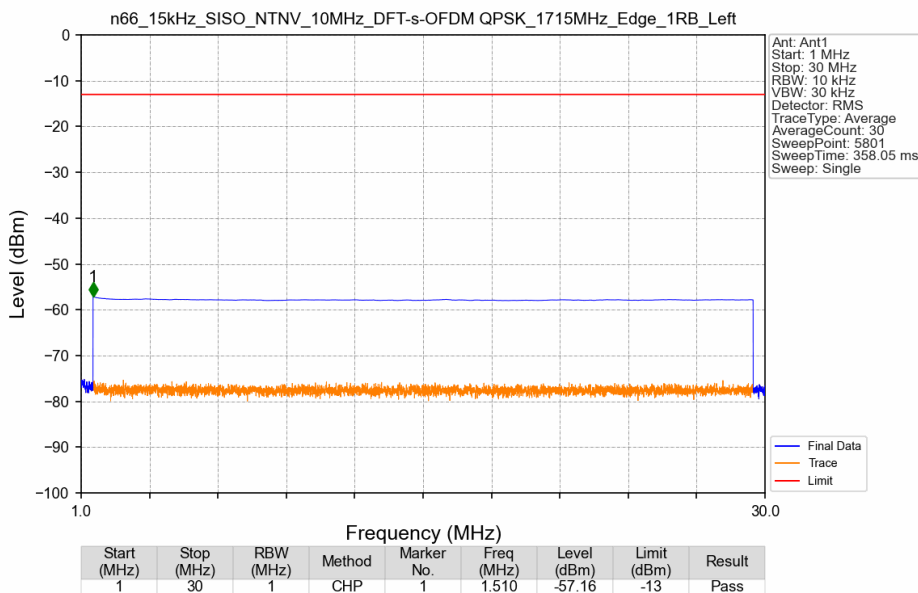
n66_15kHz_SISO_NTNV_10MHz_DFT-s-OFDM QPSK_1715MHz_Edge_1RB_Left
