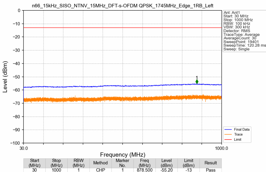
n66_15kHz_SISO_NTNV_15MHz_DFT-s-OFDM QPSK_1745MHz_Edge_1RB_Left
