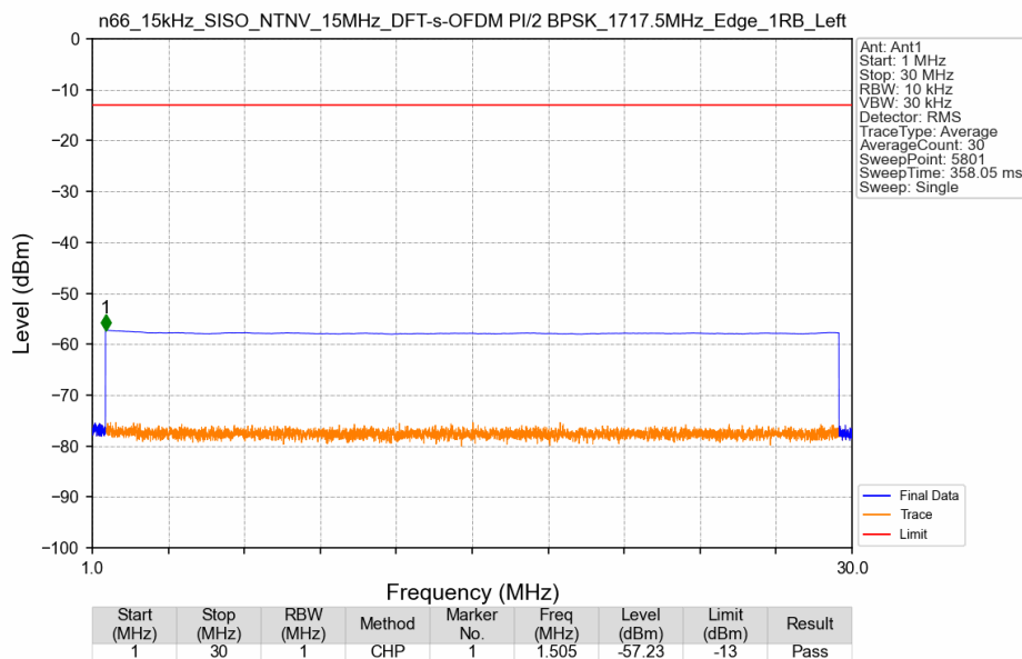
n66_15kHz_SISO_NTNV_15MHz_DFT-s-OFDM PI/2 BPSK_1717.5MHz_Edge_1RB_Left
