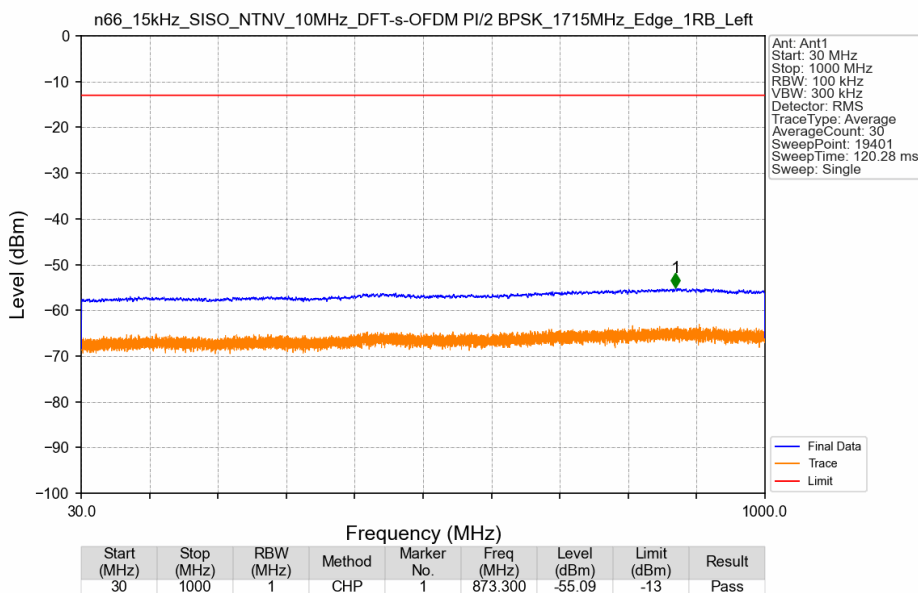
n66_15kHz_SISO_NTNV_10MHz_DFT-s-OFDM PI/2 BPSK_1715MHz_Edge_1RB_Left
