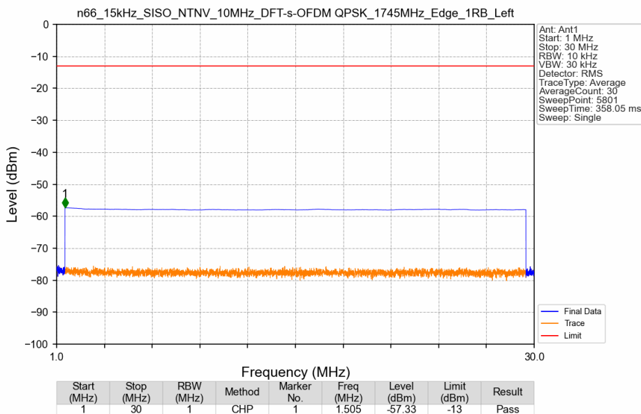
n66_15kHz_SISO_NTNV_10MHz_DFT-s-OFDM QPSK_1745MHz_Edge_1RB_Left
