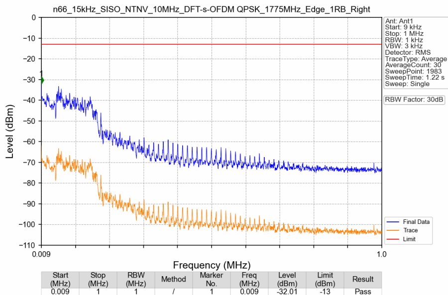
n66_15kHz_SISO_NTNV_10MHz_DFT-s-OFDM QPSK_1775MHz_Edge_1RB_Right
