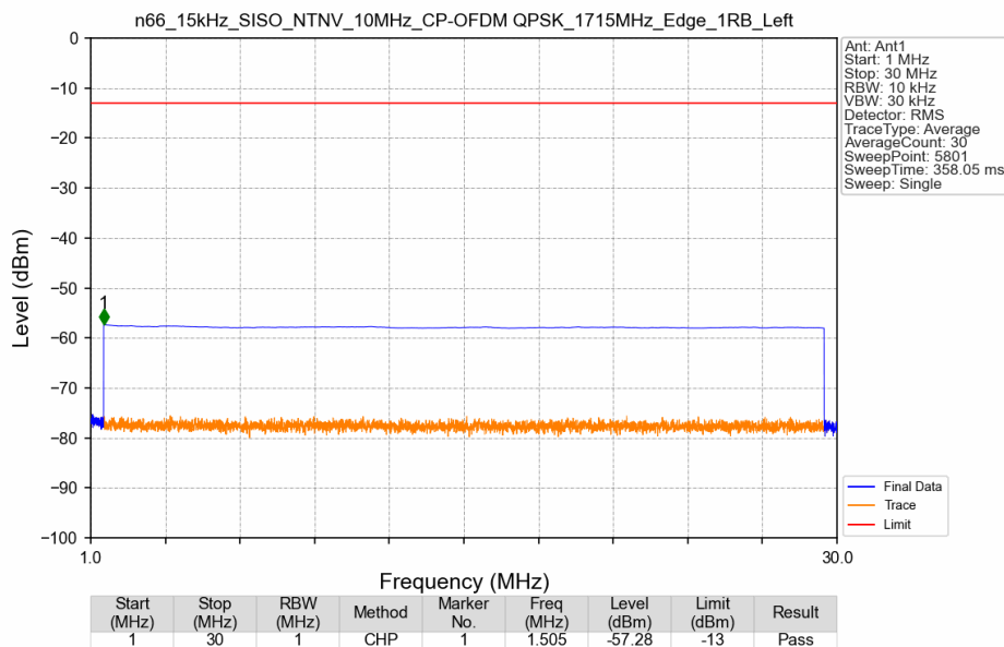
n66_15kHz_SISO_NTNV_10MHz_CP-OFDM QPSK_1715MHz_Edge_1RB_Left
