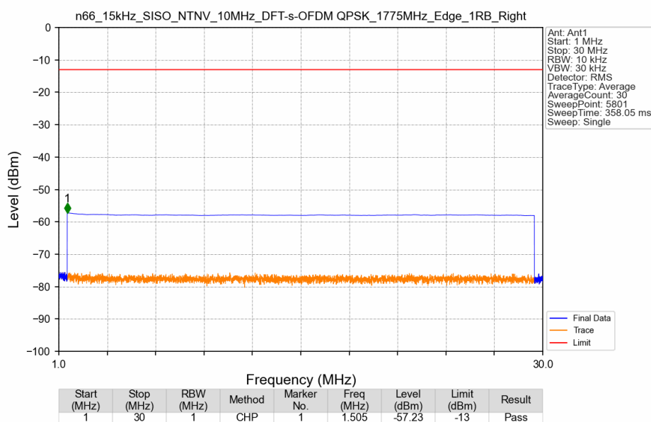
n66_15kHz_SISO_NTNV_10MHz_DFT-s-OFDM QPSK_1775MHz_Edge_1RB_Right
