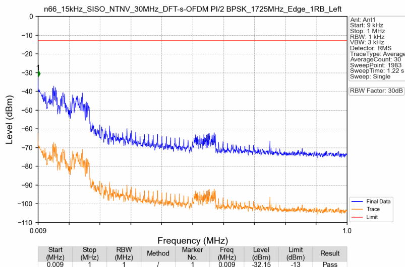
n66_15kHz_SISO_NTNV_30MHz_DFT-s-OFDM PI/2 BPSK_1725MHz_Edge_1RB_Left
