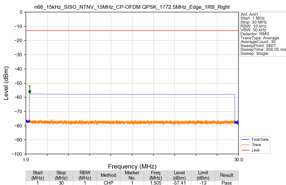
n66_15kHz_SISO_NTNV_15MHz_CP-OFDM QPSK_1772.5MHz_Edge_1RB_Right
