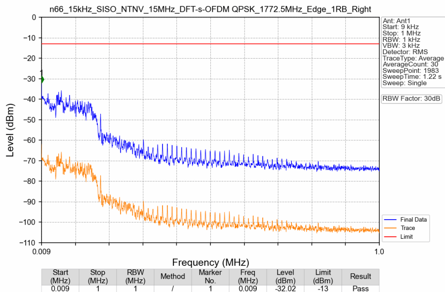
n66_15kHz_SISO_NTNV_15MHz_DFT-s-OFDM QPSK_1772.5MHz_Edge_1RB_Right
