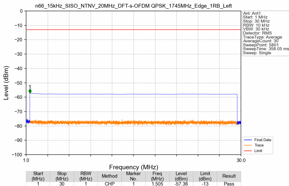
n66_15kHz_SISO_NTNV_20MHz_DFT-s-OFDM QPSK_1745MHz_Edge_1RB_Left
