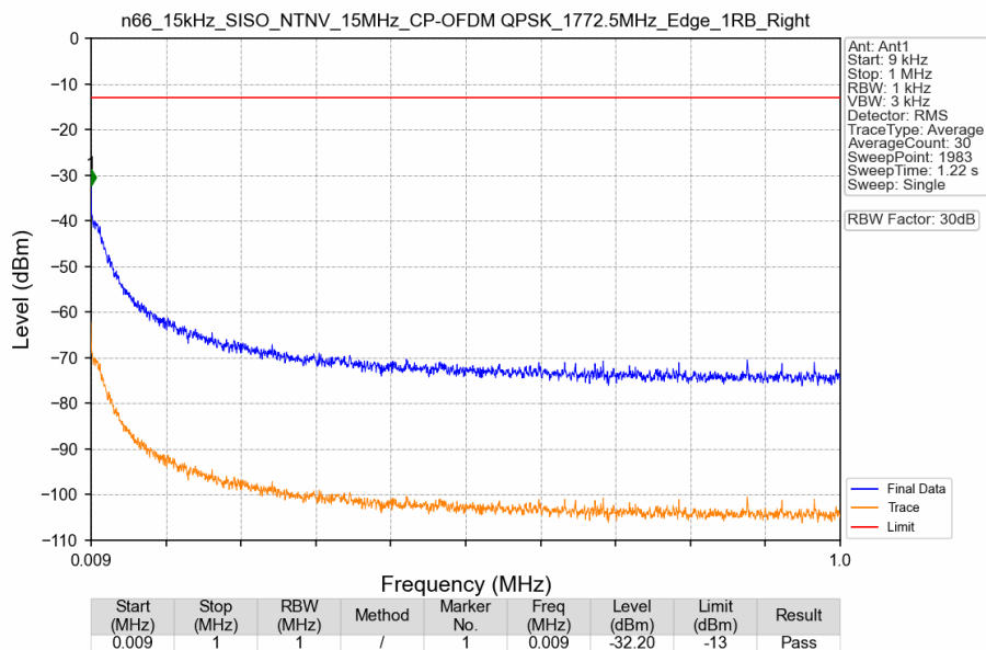
n66_15kHz_SISO_NTNV_15MHz_CP-OFDM QPSK_1772.5MHz_Edge_1RB_Right
