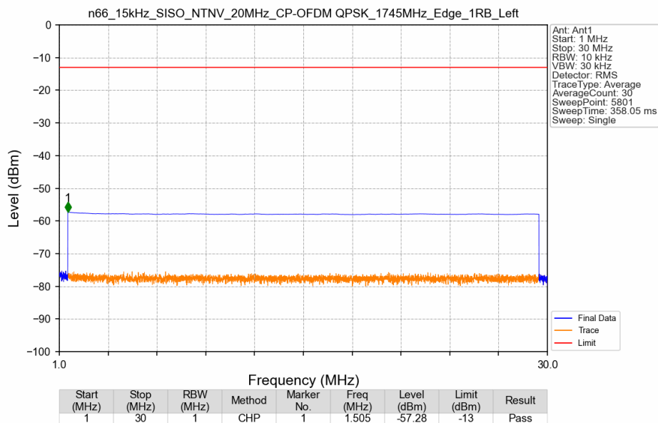
n66_15kHz_SISO_NTNV_20MHz_CP-OFDM QPSK_1745MHz_Edge_1RB_Left
