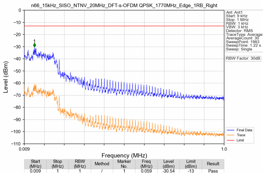
n66_15kHz_SISO_NTNV_20MHz_DFT-s-OFDM QPSK_1770MHz_Edge_1RB_Right
