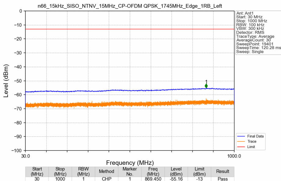
n66_15kHz_SISO_NTNV_15MHz_CP-OFDM QPSK_1745MHz_Edge_1RB_Left
