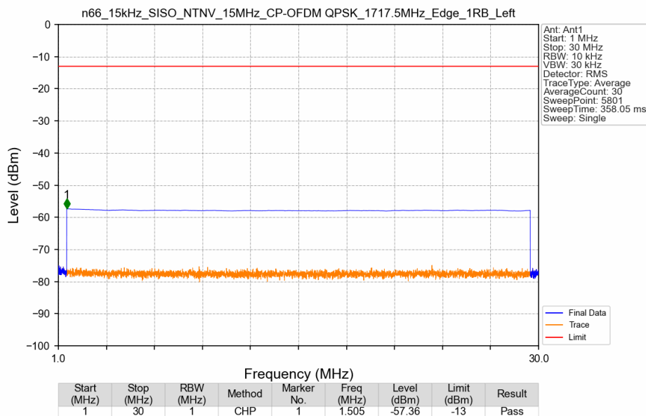
n66_15kHz_SISO_NTNV_15MHz_CP-OFDM QPSK_1717.5MHz_Edge_1RB_Left
