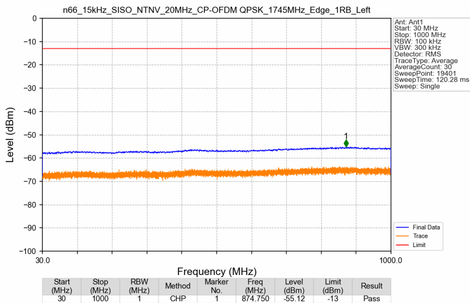
n66_15kHz_SISO_NTNV_20MHz_CP-OFDM QPSK_1745MHz_Edge_1RB_Left
