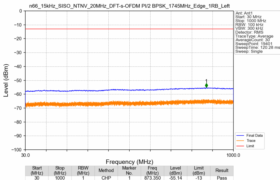
n66_15kHz_SISO_NTNV_20MHz_DFT-s-OFDM PI/2 BPSK_1745MHz_Edge_1RB_Left
