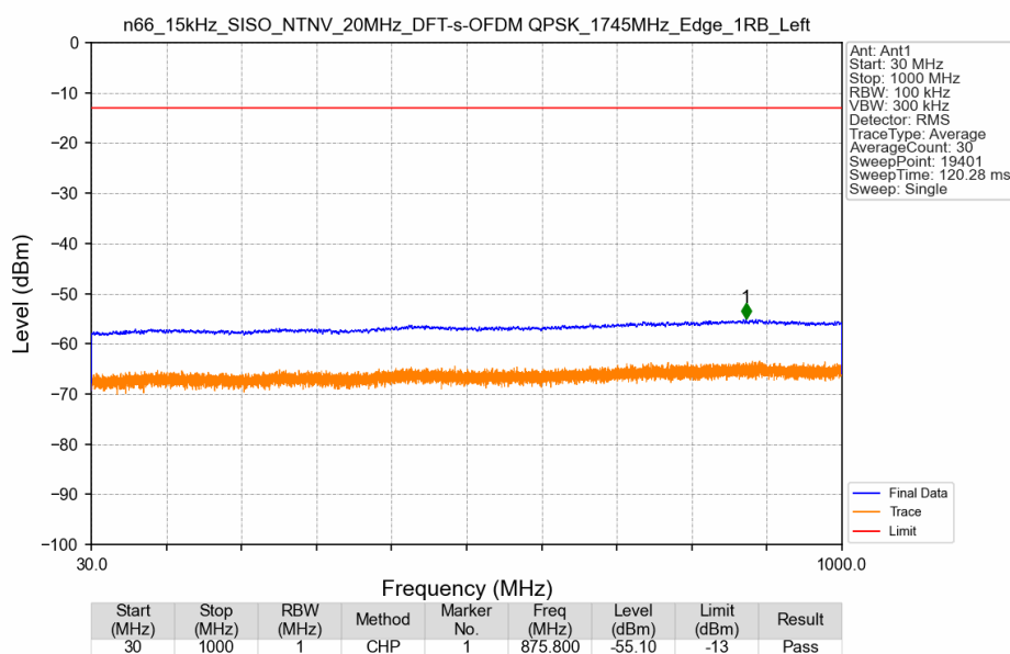
n66_15kHz_SISO_NTNV_20MHz_DFT-s-OFDM QPSK_1745MHz_Edge_1RB_Left
