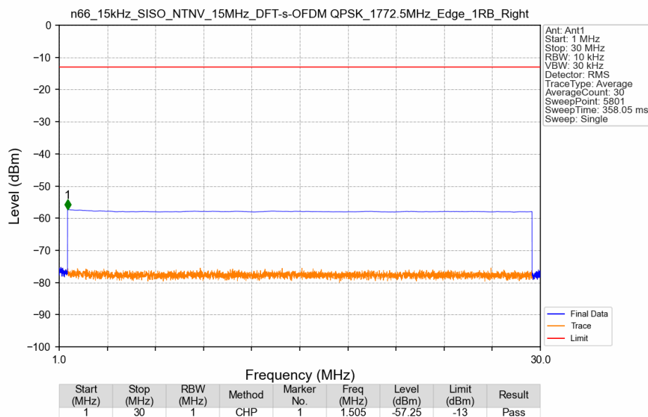
n66_15kHz_SISO_NTNV_15MHz_DFT-s-OFDM QPSK_1772.5MHz_Edge_1RB_Right
