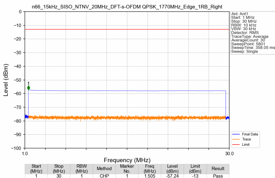
n66_15kHz_SISO_NTNV_20MHz_DFT-s-OFDM QPSK_1770MHz_Edge_1RB_Right
