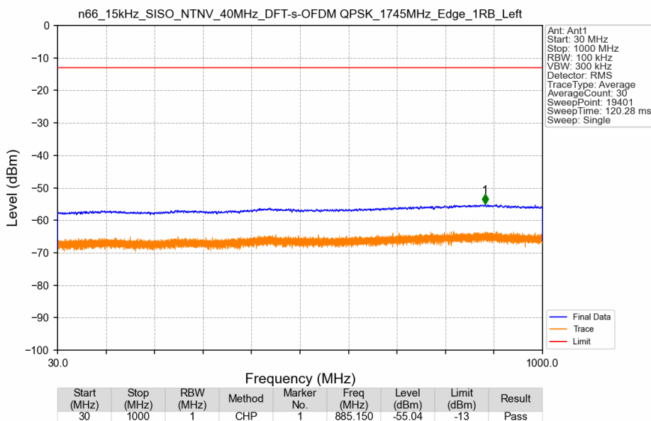
n66_15kHz_SISO_NTNV_40MHz_DFT-s-OFDM QPSK_1745MHz_Edge_1RB_Left
