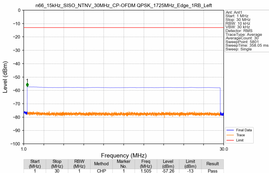
n66_15kHz_SISO_NTNV_30MHz_CP-OFDM QPSK_1725MHz_Edge_1RB_Left
