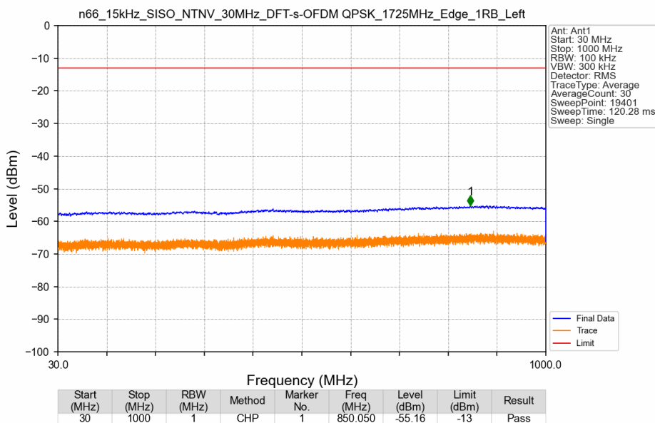
n66_15kHz_SISO_NTNV_30MHz_DFT-s-OFDM QPSK_1725MHz_Edge_1RB_Left
