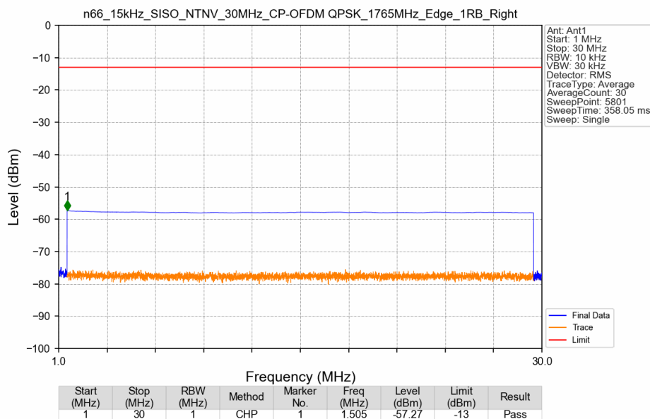
n66_15kHz_SISO_NTNV_30MHz_CP-OFDM QPSK_1765MHz_Edge_1RB_Right
