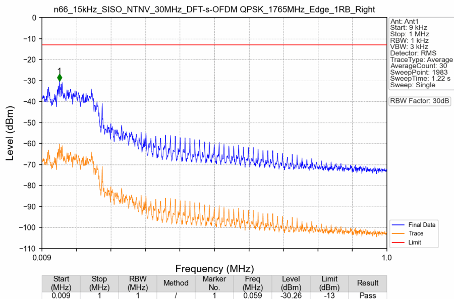
n66_15kHz_SISO_NTNV_30MHz_DFT-s-OFDM QPSK_1765MHz_Edge_1RB_Right
