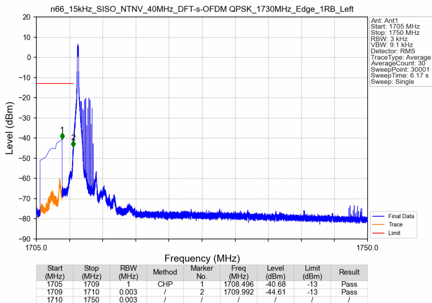
n66_15kHz_SISO_NTNV_40MHz_DFT-s-OFDM QPSK_1730MHz_Edge_1RB_Left
