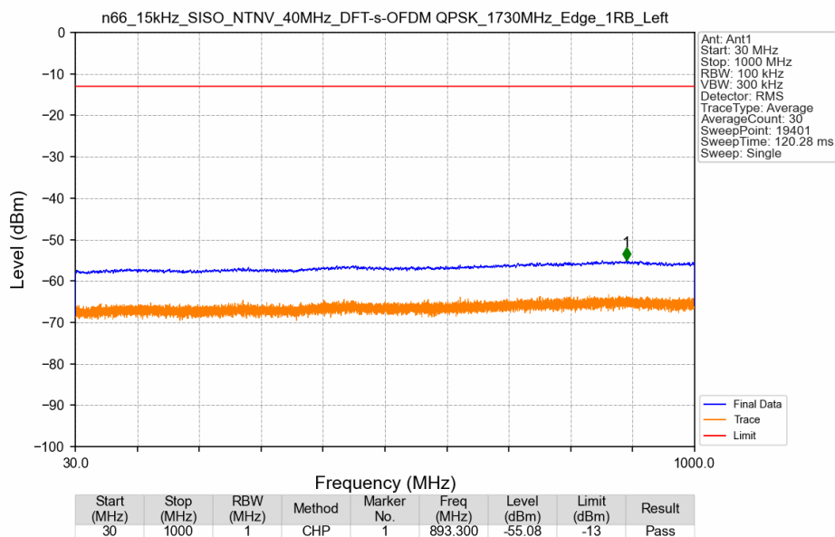
n66_15kHz_SISO_NTNV_40MHz_DFT-s-OFDM QPSK_1730MHz_Edge_1RB_Left
