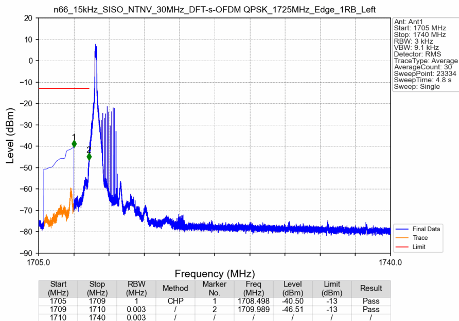
n66_15kHz_SISO_NTNV_30MHz_DFT-s-OFDM QPSK_1725MHz_Edge_1RB_Left
