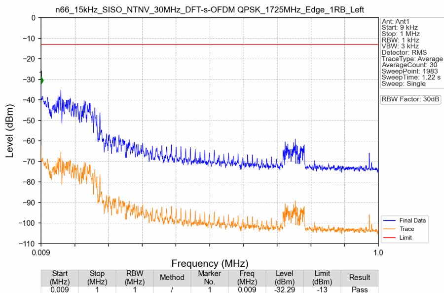
n66_15kHz_SISO_NTNV_30MHz_DFT-s-OFDM QPSK_1725MHz_Edge_1RB_Left
