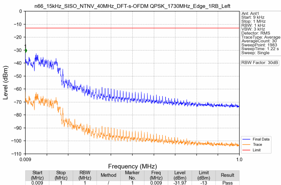
n66_15kHz_SISO_NTNV_40MHz_DFT-s-OFDM QPSK_1730MHz_Edge_1RB_Left
