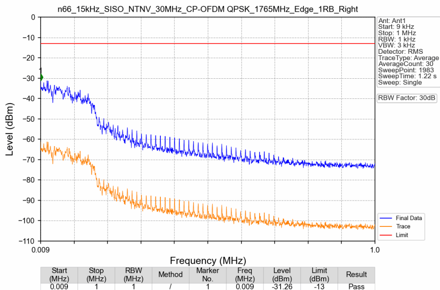
n66_15kHz_SISO_NTNV_30MHz_CP-OFDM QPSK_1765MHz_Edge_1RB_Right
