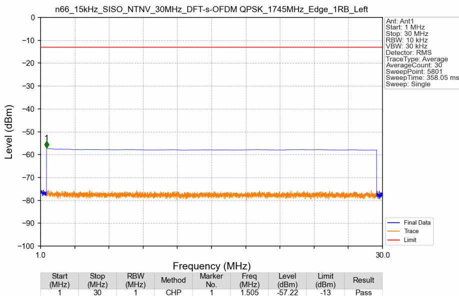
n66_15kHz_SISO_NTNV_30MHz_DFT-s-OFDM QPSK_1745MHz_Edge_1RB_Left
