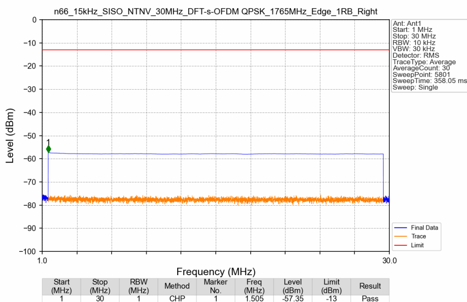
n66_15kHz_SISO_NTNV_30MHz_DFT-s-OFDM QPSK_1765MHz_Edge_1RB_Right
