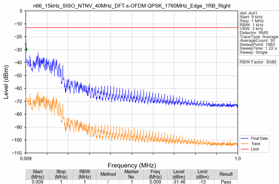
n66_15kHz_SISO_NTNV_40MHz_DFT-s-OFDM QPSK_1760MHz_Edge_1RB_Right
