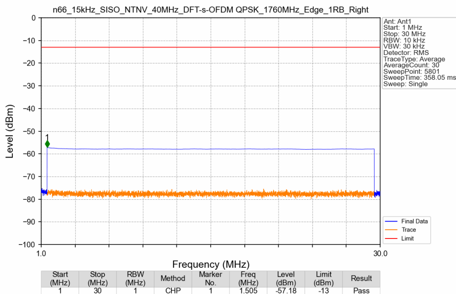
n66_15kHz_SISO_NTNV_40MHz_DFT-s-OFDM QPSK_1760MHz_Edge_1RB_Right
