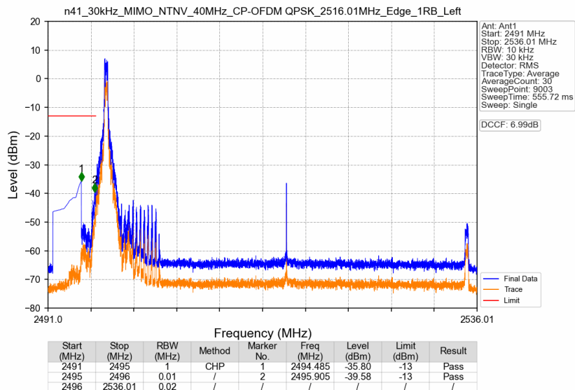
n41_30kHz_MIMO_NTNV_40MHz_CP-OFDM QPSK_2516.01MHz_Edge_1RB_Left
