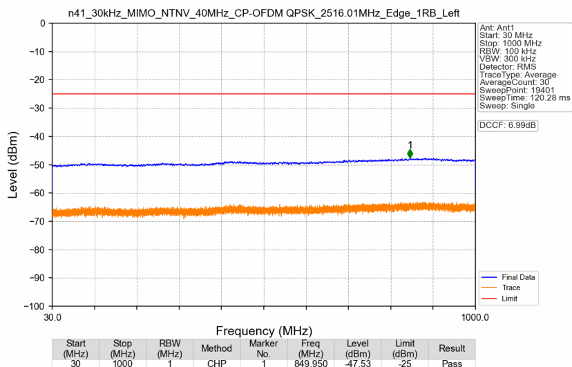
n41_30kHz_MIMO_NTNV_40MHz_CP-OFDM QPSK_2516.01MHz_Edge_1RB_Left
