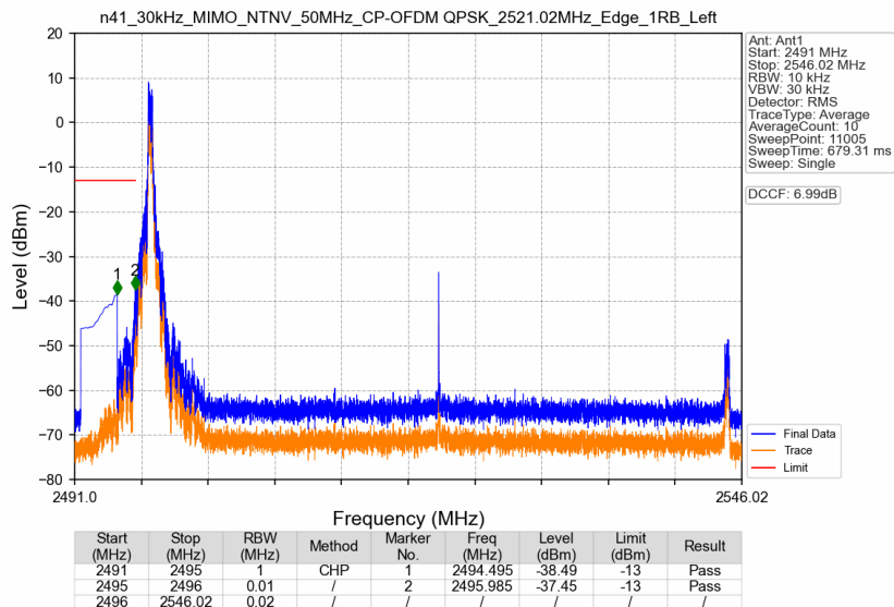
n41_30kHz_MIMO_NTNV_50MHz_CP-OFDM QPSK_2521.02MHz_Edge_1RB_Left
