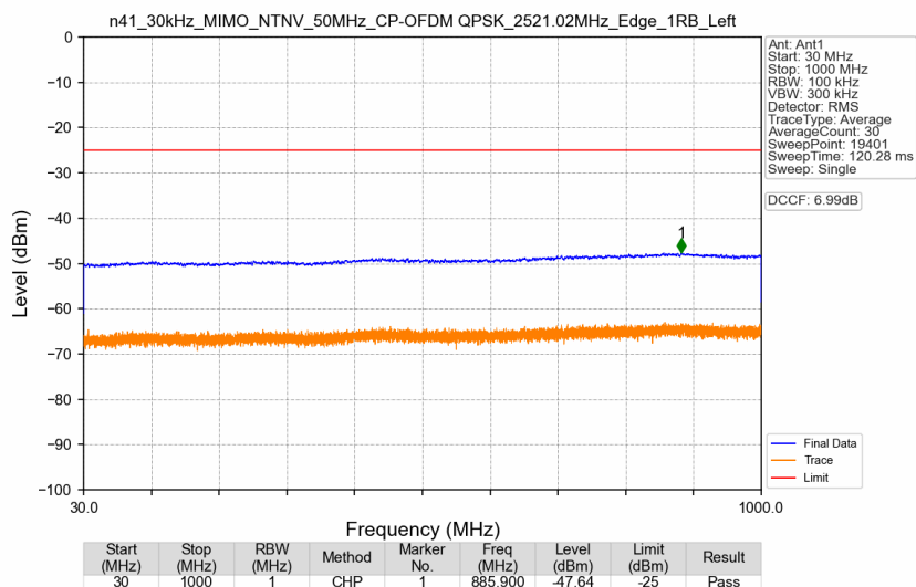
n41_30kHz_MIMO_NTNV_50MHz_CP-OFDM QPSK_2521.02MHz_Edge_1RB_Left
