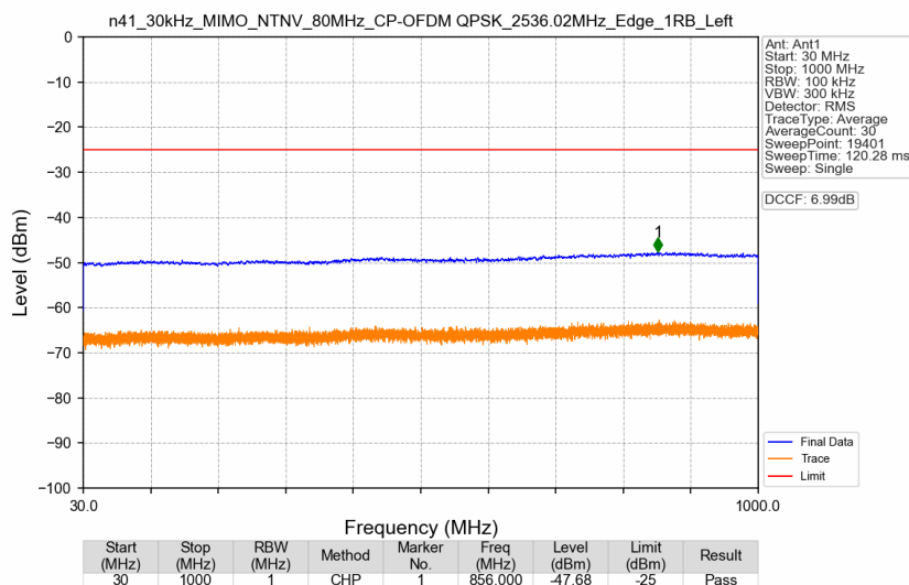
n41_30kHz_MIMO_NTNV_80MHz_CP-OFDM QPSK_2536.02MHz_Edge_1RB_Left
