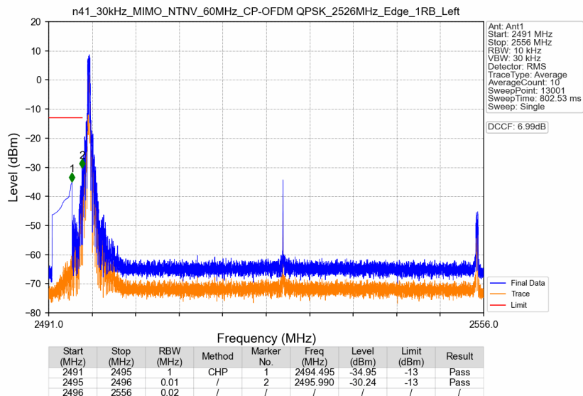
n41_30kHz_MIMO_NTNV_60MHz_CP-OFDM QPSK_2526MHz_Edge_1RB_Left
