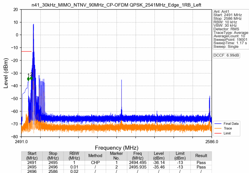
n41_30kHz_MIMO_NTNV_90MHz_CP-OFDM QPSK_2541MHz_Edge_1RB_Left
