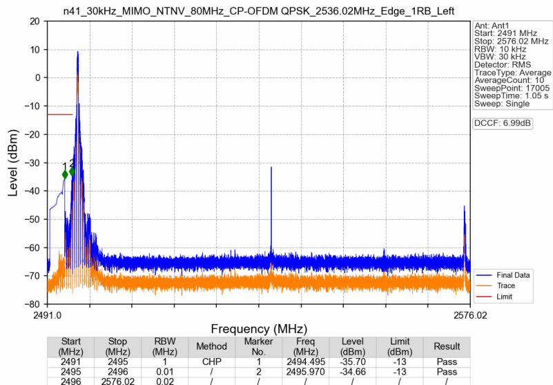
n41_30kHz_MIMO_NTNV_80MHz_CP-OFDM QPSK_2536.02MHz_Edge_1RB_Left
