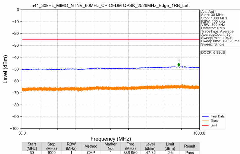
n41_30kHz_MIMO_NTNV_60MHz_CP-OFDM QPSK_2526MHz_Edge_1RB_Left
