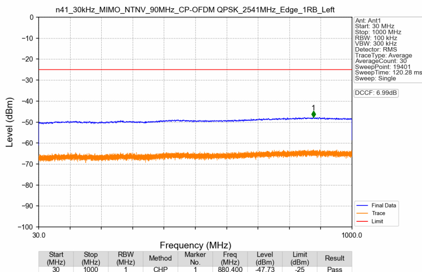
n41_30kHz_MIMO_NTNV_90MHz_CP-OFDM QPSK_2541MHz_Edge_1RB_Left
