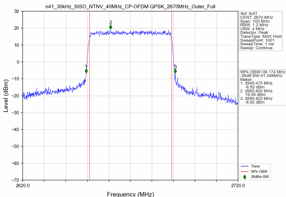
n41_30kHz_SISO_NTNV_40MHz_CP-OFDM QPSK_2670MHz_Outer_Full
