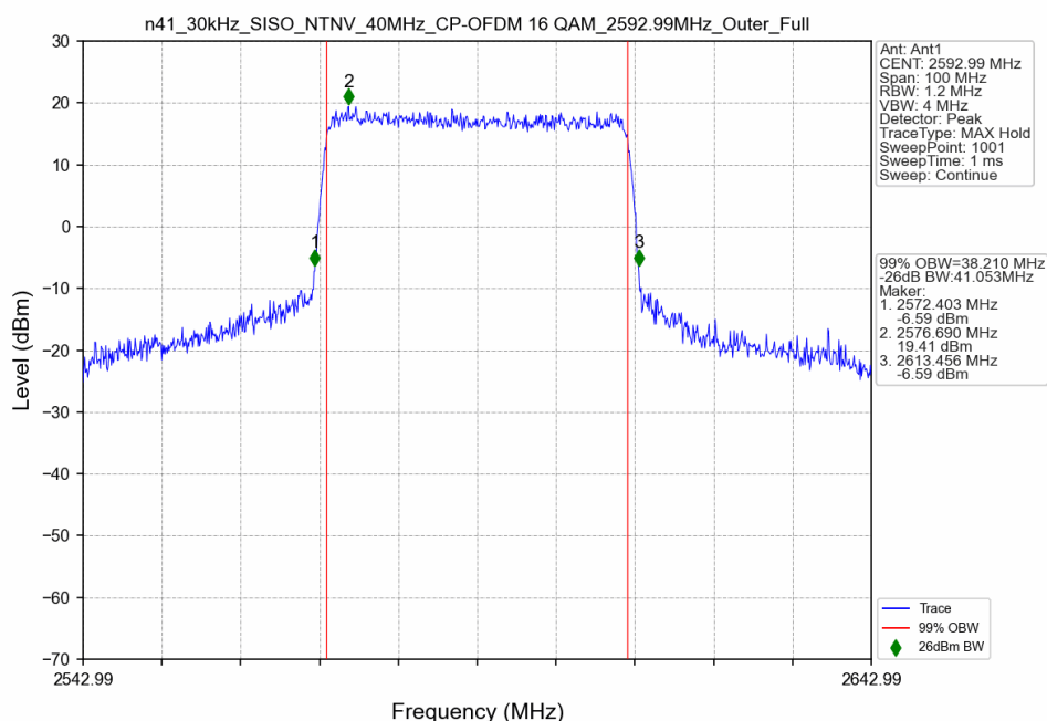
n41_30kHz_SISO_NTNV_40MHz_CP-OFDM 16 QAM_2592.99MHz_Outer_Full
