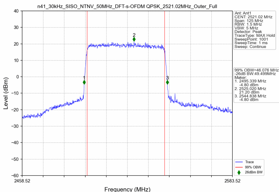
n41_30kHz_SISO_NTNV_50MHz_DFT-s-OFDM QPSK_2521.02MHz_Outer_Full
