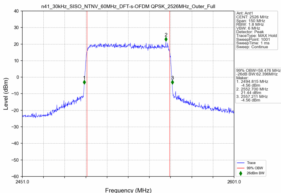
n41_30kHz_SISO_NTNV_60MHz_DFT-s-OFDM QPSK_2526MHz_Outer_Full
