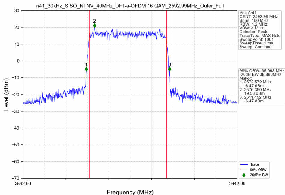
n41_30kHz_SISO_NTNV_40MHz_DFT-s-OFDM 16 QAM_2592.99MHz_Outer_Full
