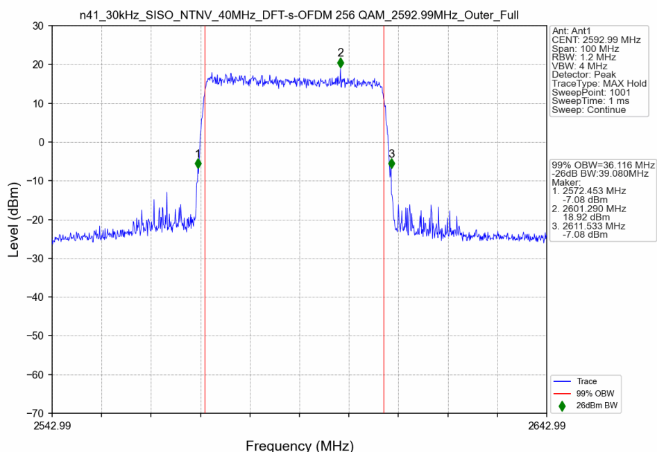
n41_30kHz_SISO_NTNV_40MHz_DFT-s-OFDM 256 QAM_2592.99MHz_Outer_Full
