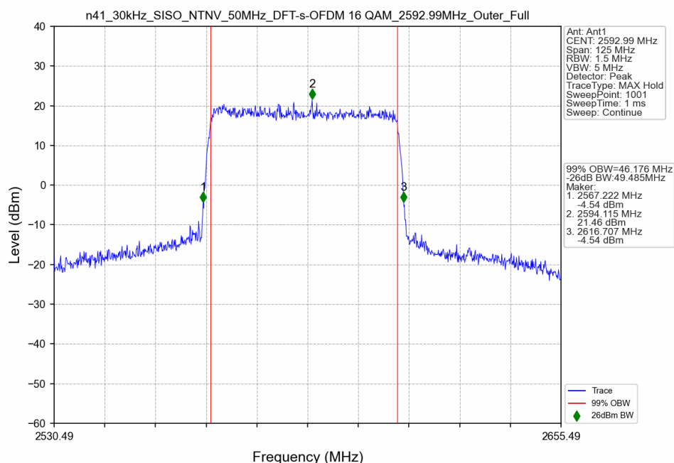
n41_30kHz_SISO_NTNV_50MHz_DFT-s-OFDM 16 QAM_2592.99MHz_Outer_Full
