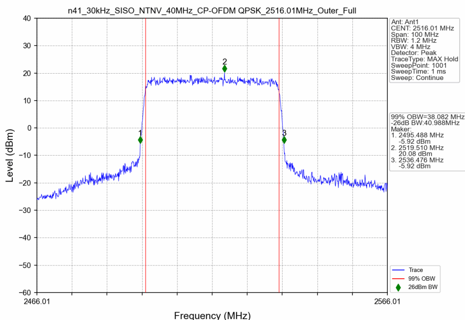
n41_30kHz_SISO_NTNV_40MHz_CP-OFDM QPSK_2516.01MHz_Outer_Full
