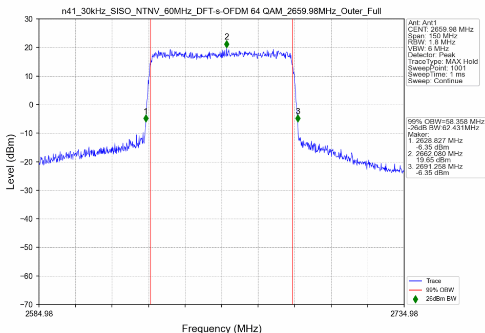
n41_30kHz_SISO_NTNV_60MHz_DFT-s-OFDM 64 QAM_2659.98MHz_Outer_Full
