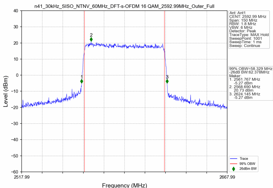
n41_30kHz_SISO_NTNV_60MHz_DFT-s-OFDM 16 QAM_2592.99MHz_Outer_Full
