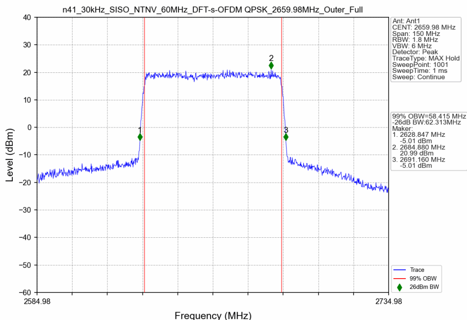
n41_30kHz_SISO_NTNV_60MHz_DFT-s-OFDM QPSK_2659.98MHz_Outer_Full
