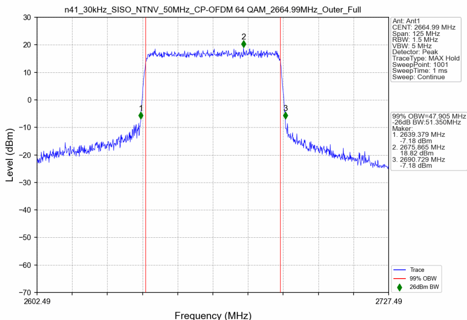
n41_30kHz_SISO_NTNV_50MHz_CP-OFDM 64 QAM_2664.99MHz_Outer_Full
