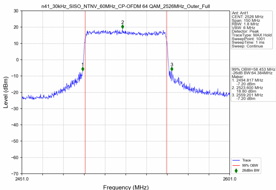
n41_30kHz_SISO_NTNV_60MHz_CP-OFDM 64 QAM_2526MHz_Outer_Full
