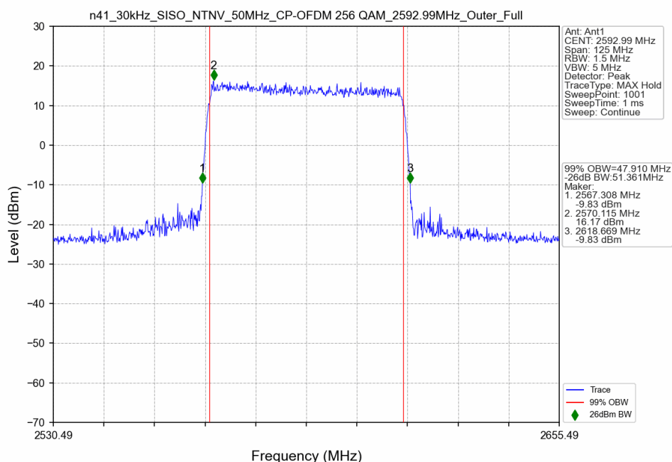
n41_30kHz_SISO_NTNV_50MHz_CP-OFDM 256 QAM_2592.99MHz_Outer_Full
