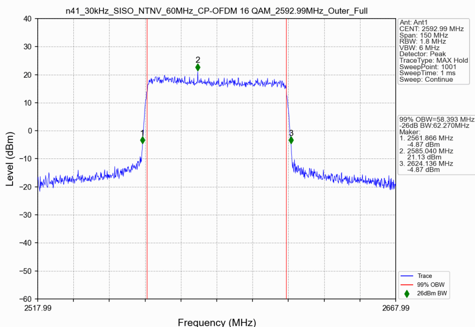
n41_30kHz_SISO_NTNV_60MHz_CP-OFDM 16 QAM_2592.99MHz_Outer_Full
