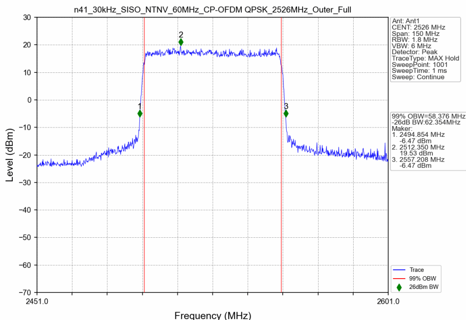
n41_30kHz_SISO_NTNV_60MHz_CP-OFDM QPSK_2526MHz_Outer_Full
