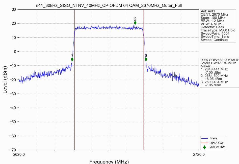
n41_30kHz_SISO_NTNV_40MHz_CP-OFDM 64 QAM_2670MHz_Outer_Full
