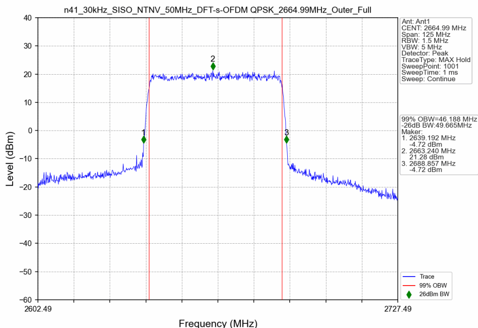
n41_30kHz_SISO_NTNV_50MHz_DFT-s-OFDM QPSK_2664.99MHz_Outer_Full
