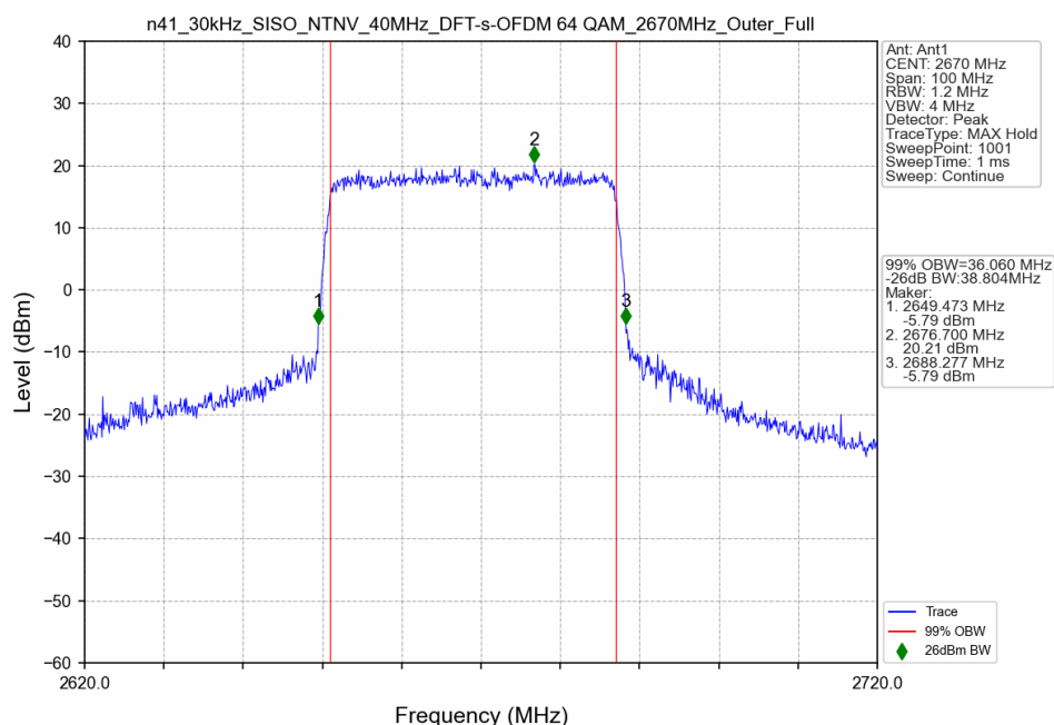
n41_30kHz_SISO_NTNV_40MHz_DFT-s-OFDM 64 QAM_2670MHz_Outer_Full
