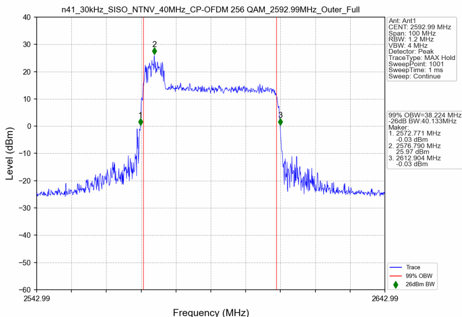
n41_30kHz_SISO_NTNV_40MHz_CP-OFDM 256 QAM_2592.99MHz_Outer_Full
