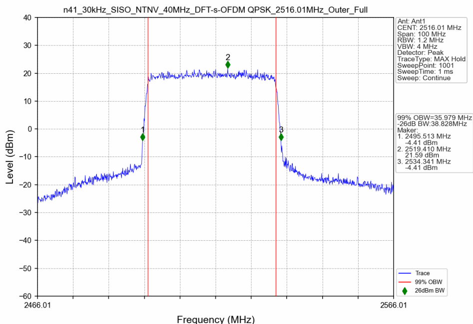
n41_30kHz_SISO_NTNV_40MHz_DFT-s-OFDM QPSK_2516.01MHz_Outer_Full
