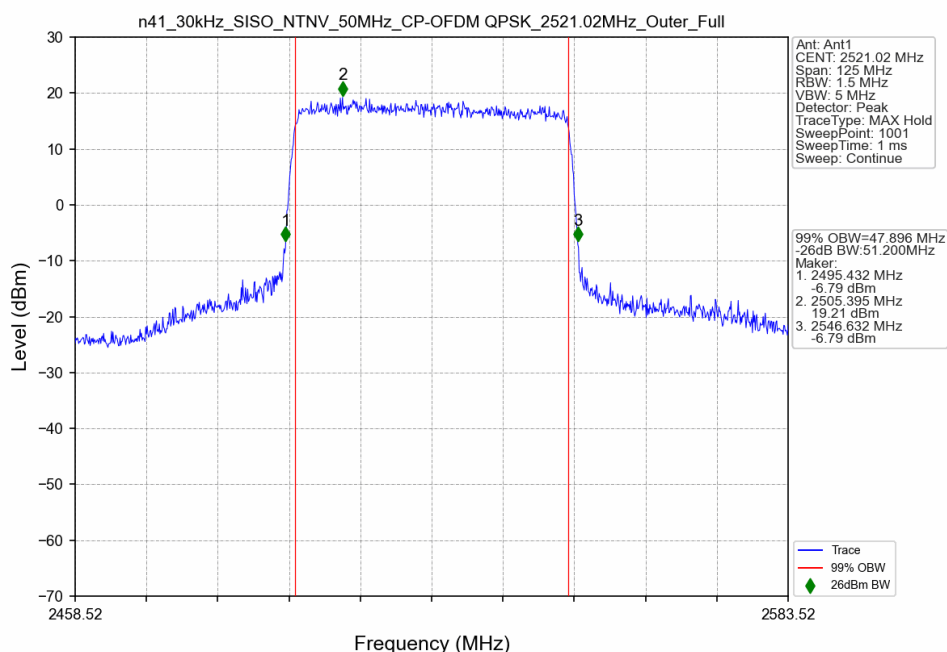
n41_30kHz_SISO_NTNV_50MHz_CP-OFDM QPSK_2521.02MHz_Outer_Full
