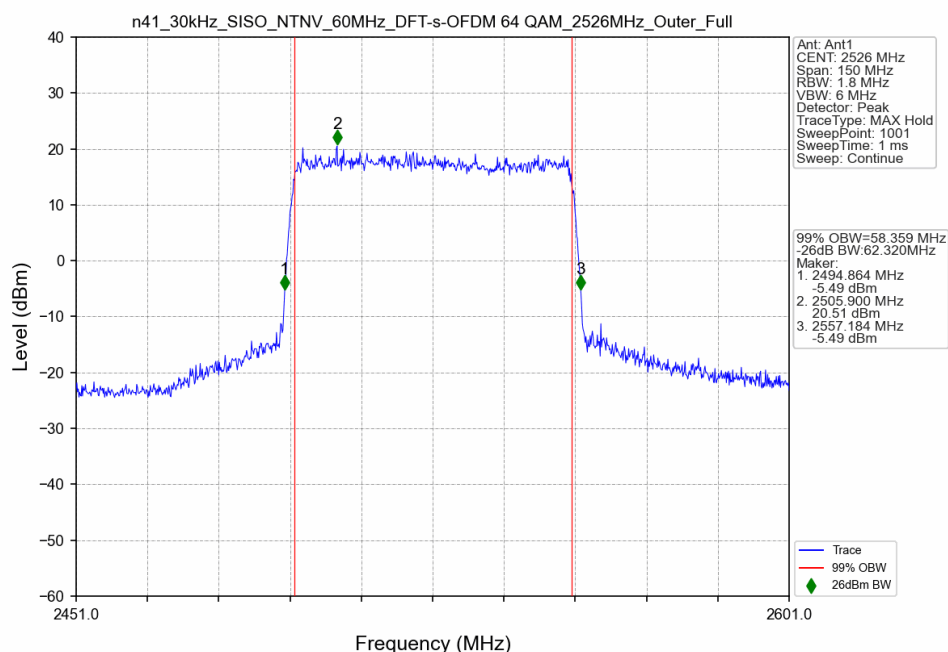
n41_30kHz_SISO_NTNV_60MHz_DFT-s-OFDM 64 QAM_2526MHz_Outer_Full
