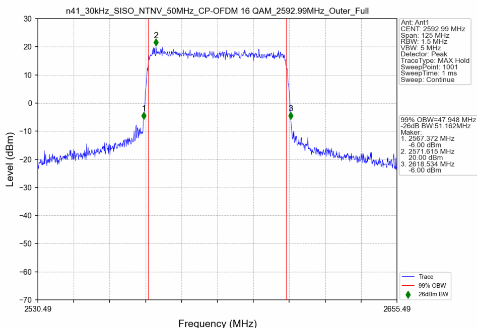
n41_30kHz_SISO_NTNV_50MHz_CP-OFDM 16 QAM_2592.99MHz_Outer_Full
