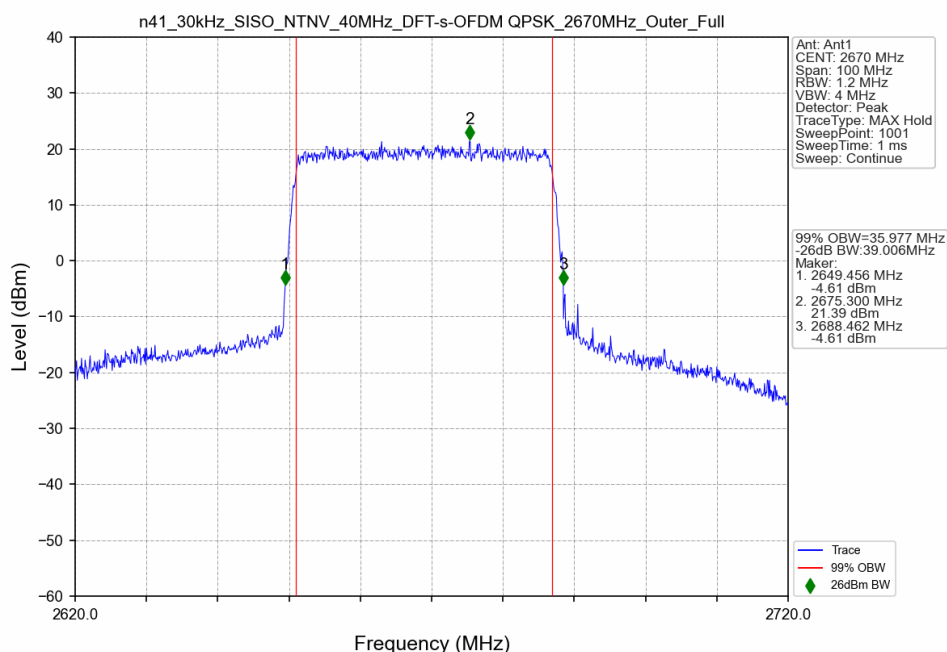
n41_30kHz_SISO_NTNV_40MHz_DFT-s-OFDM QPSK_2670MHz_Outer_Full
