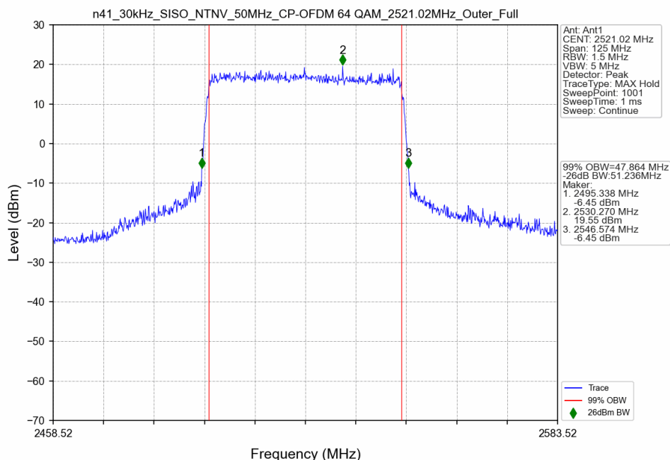
n41_30kHz_SISO_NTNV_50MHz_CP-OFDM 64 QAM_2521.02MHz_Outer_Full
