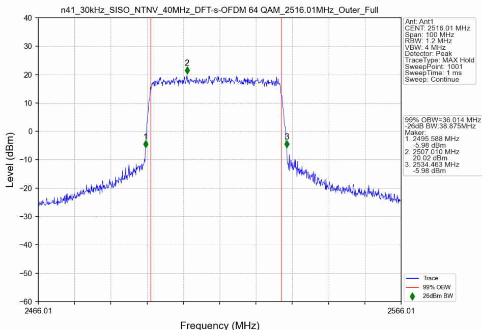
n41_30kHz_SISO_NTNV_40MHz_DFT-s-OFDM 64 QAM_2516.01MHz_Outer_Full
