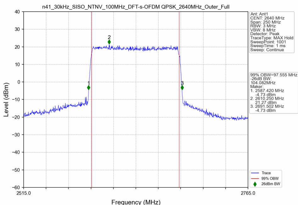
n41_30kHz_SISO_NTNV_100MHz_DFT-s-OFDM QPSK_2640MHz_Outer_Full
