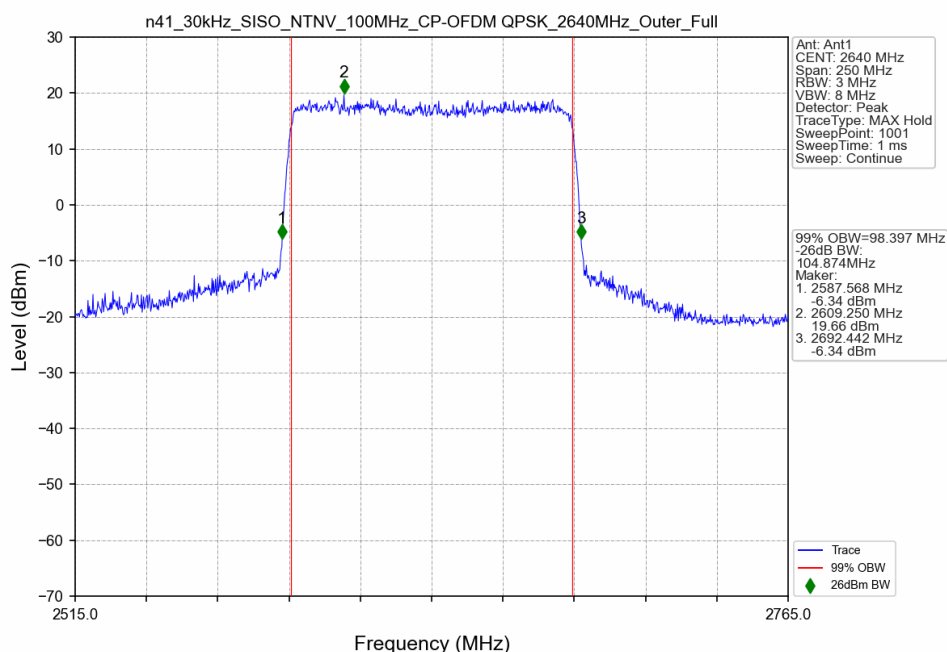
n41_30kHz_SISO_NTNV_100MHz_CP-OFDM QPSK_2640MHz_Outer_Full
