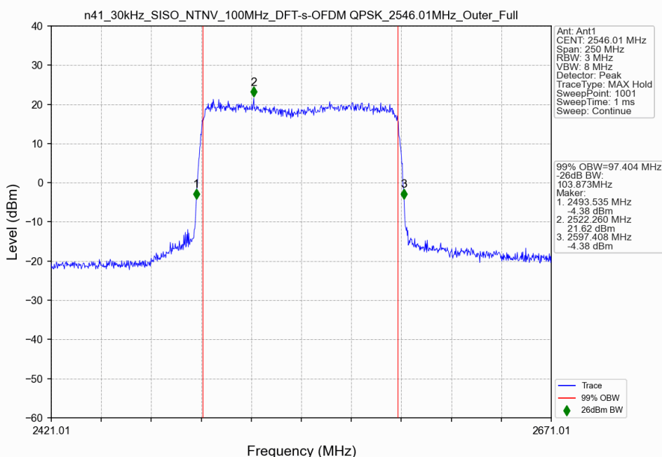
n41_30kHz_SISO_NTNV_100MHz_DFT-s-OFDM QPSK_2546.01MHz_Outer_Full
