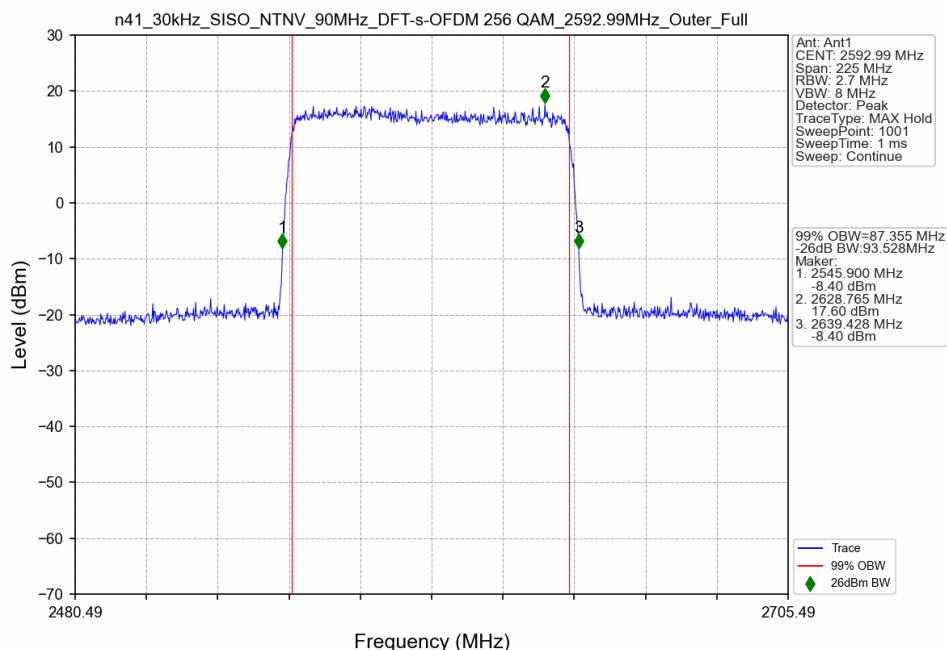
n41_30kHz_SISO_NTNV_90MHz_DFT-s-OFDM 256 QAM_2592.99MHz_Outer_Full
