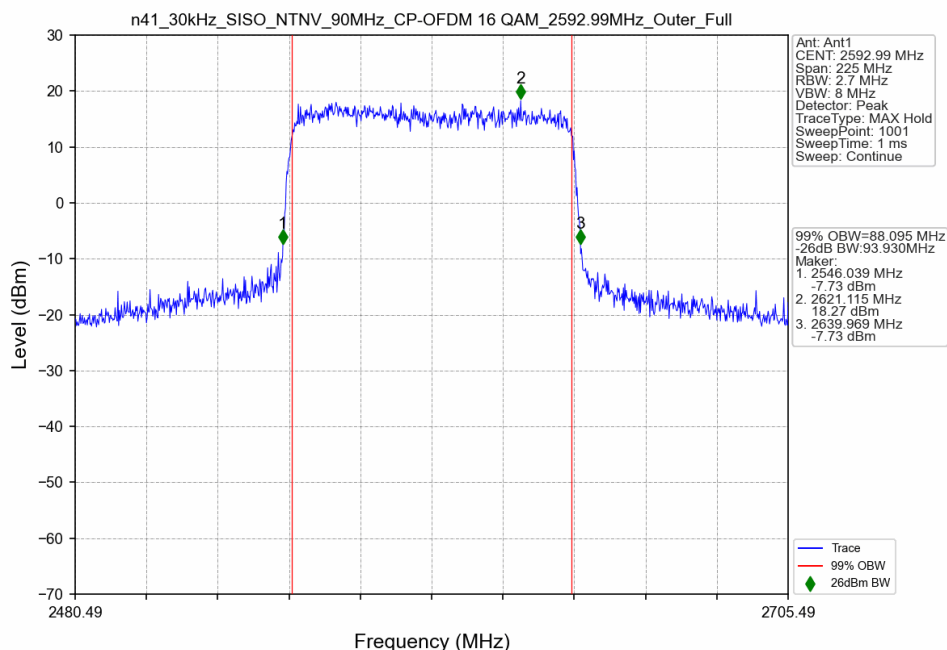
n41_30kHz_SISO_NTNV_90MHz_CP-OFDM 16 QAM_2592.99MHz_Outer_Full
