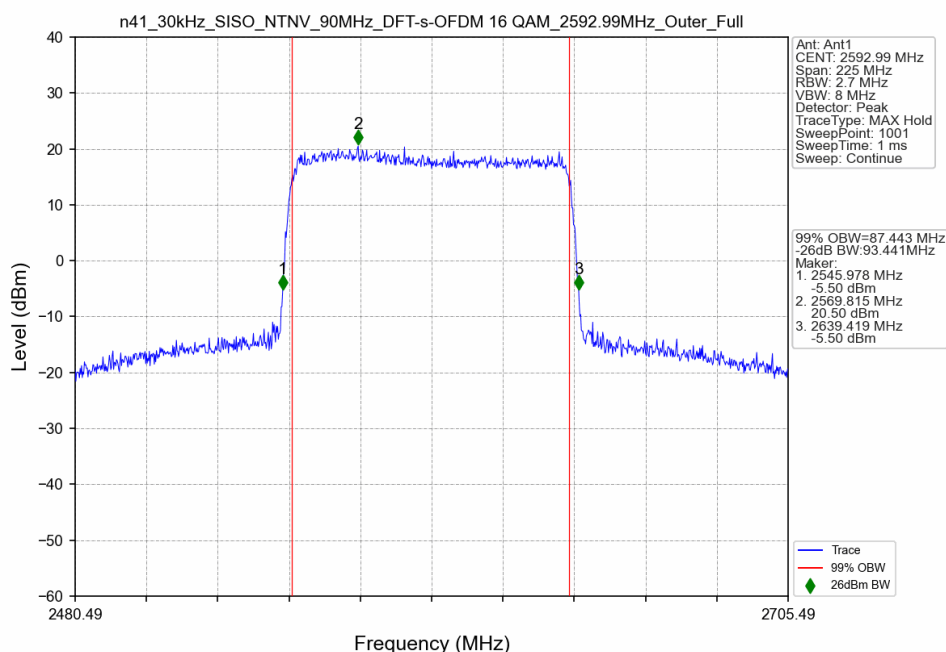
n41_30kHz_SISO_NTNV_90MHz_DFT-s-OFDM 16 QAM_2592.99MHz_Outer_Full
