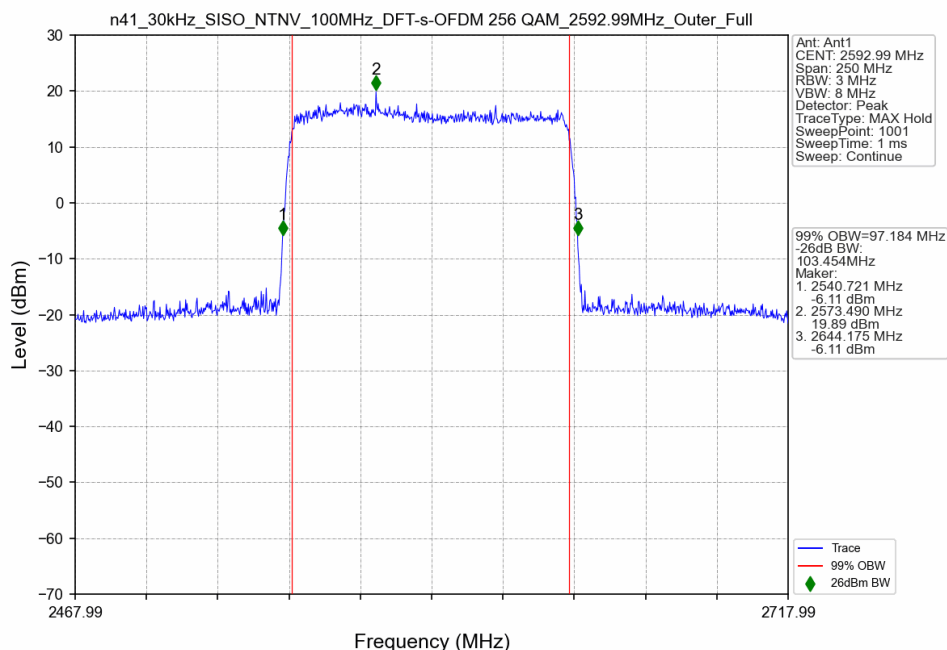
n41_30kHz_SISO_NTNV_100MHz_DFT-s-OFDM 256 QAM_2592.99MHz_Outer_Full
