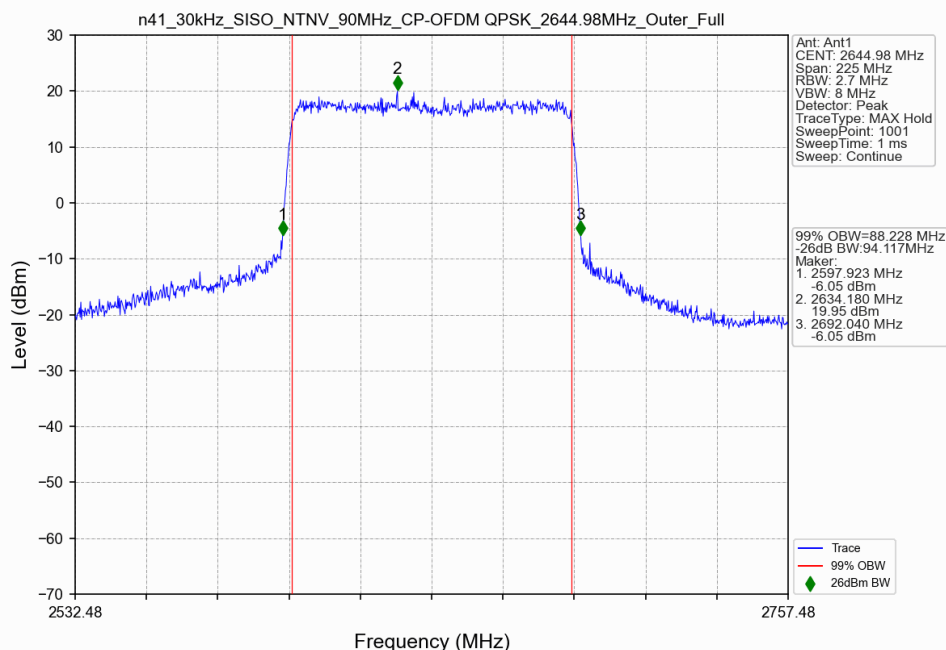
n41_30kHz_SISO_NTNV_90MHz_CP-OFDM QPSK_2644.98MHz_Outer_Full
