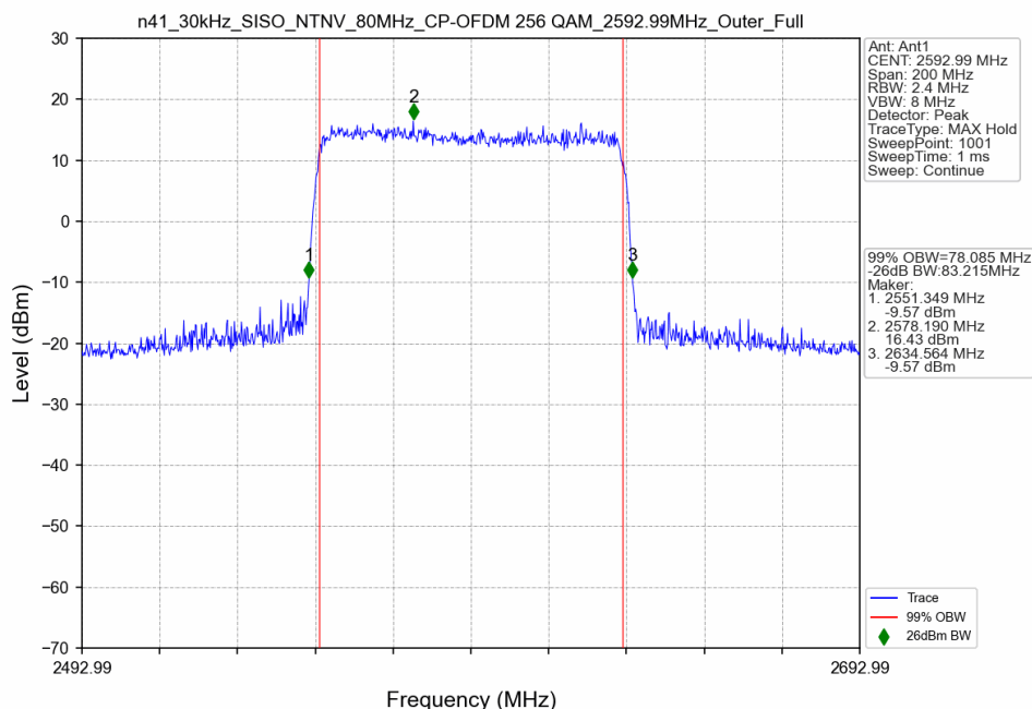
n41_30kHz_SISO_NTNV_80MHz_CP-OFDM 256 QAM_2592.99MHz_Outer_Full
