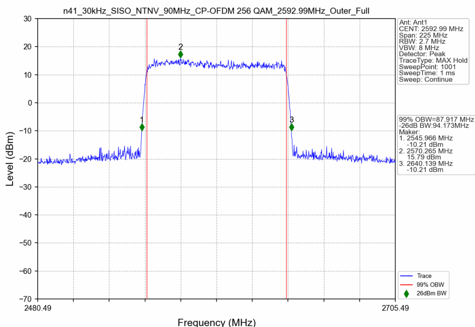
n41_30kHz_SISO_NTNV_90MHz_CP-OFDM 256 QAM_2592.99MHz_Outer_Full
