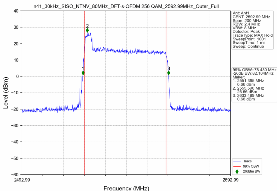
n41_30kHz_SISO_NTNV_80MHz_DFT-s-OFDM 256 QAM_2592.99MHz_Outer_Full
