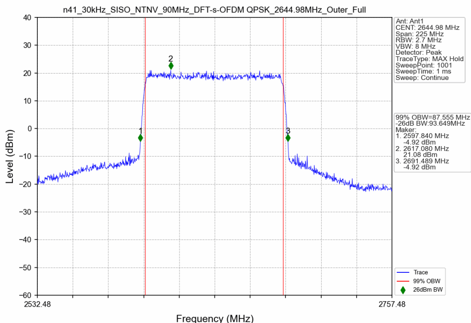
n41_30kHz_SISO_NTNV_90MHz_DFT-s-OFDM QPSK_2644.98MHz_Outer_Full
