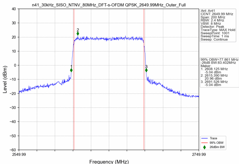
n41_30kHz_SISO_NTNV_80MHz_DFT-s-OFDM QPSK_2649.99MHz_Outer_Full
