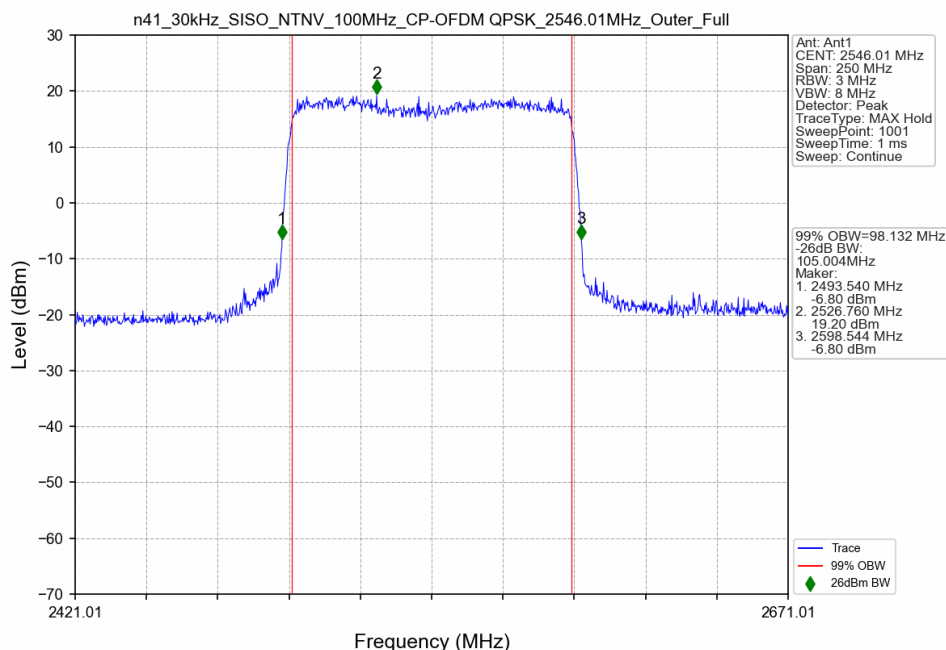
n41_30kHz_SISO_NTNV_100MHz_CP-OFDM QPSK_2546.01MHz_Outer_Full
