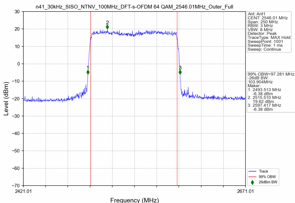
n41_30kHz_SISO_NTNV_100MHz_DFT-s-OFDM 64 QAM_2546.01MHz_Outer_Full
