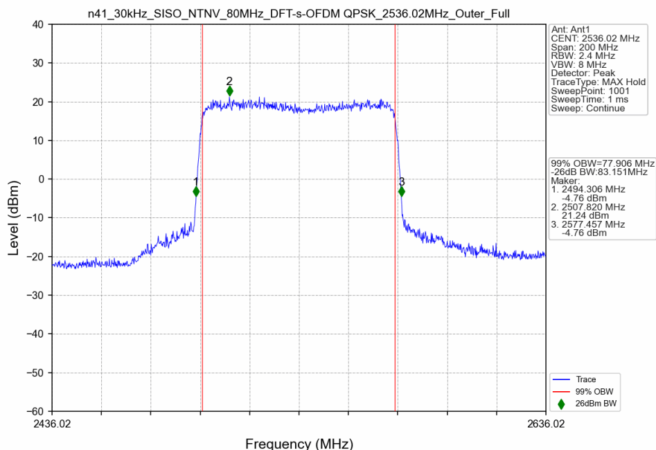
n41_30kHz_SISO_NTNV_80MHz_DFT-s-OFDM QPSK_2536.02MHz_Outer_Full
