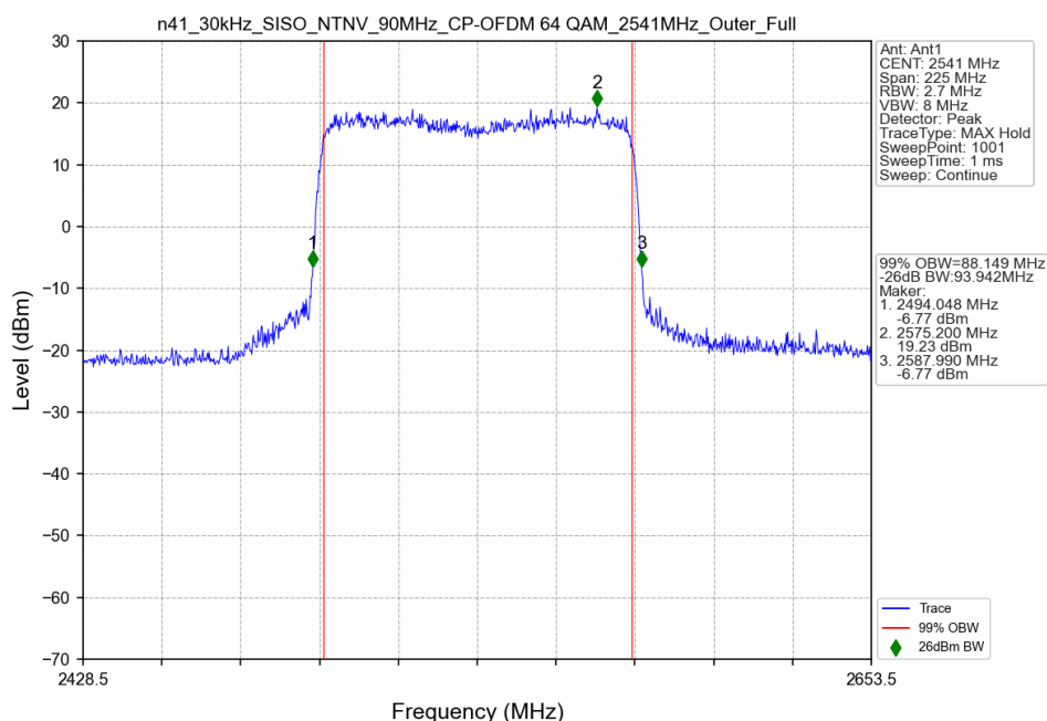
n41_30kHz_SISO_NTNV_90MHz_CP-OFDM 64 QAM_2541MHz_Outer_Full
