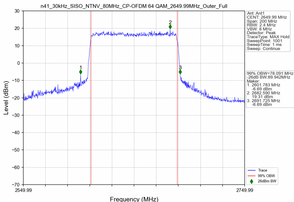
n41_30kHz_SISO_NTNV_80MHz_CP-OFDM 64 QAM_2649.99MHz_Outer_Full
