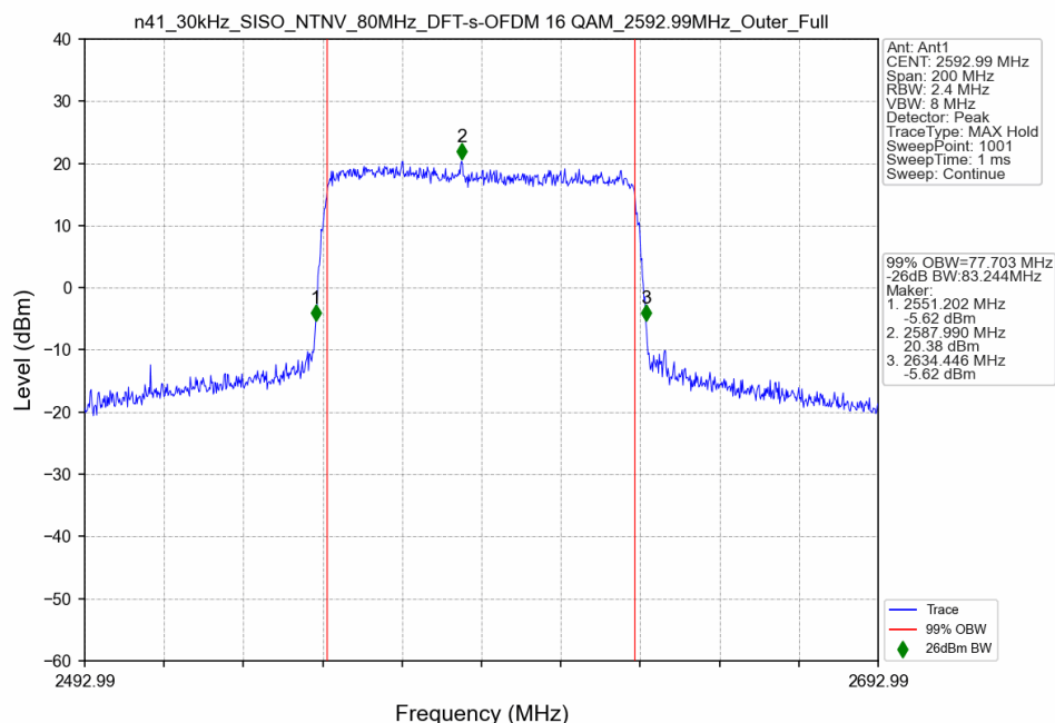
n41_30kHz_SISO_NTNV_80MHz_DFT-s-OFDM 16 QAM_2592.99MHz_Outer_Full
