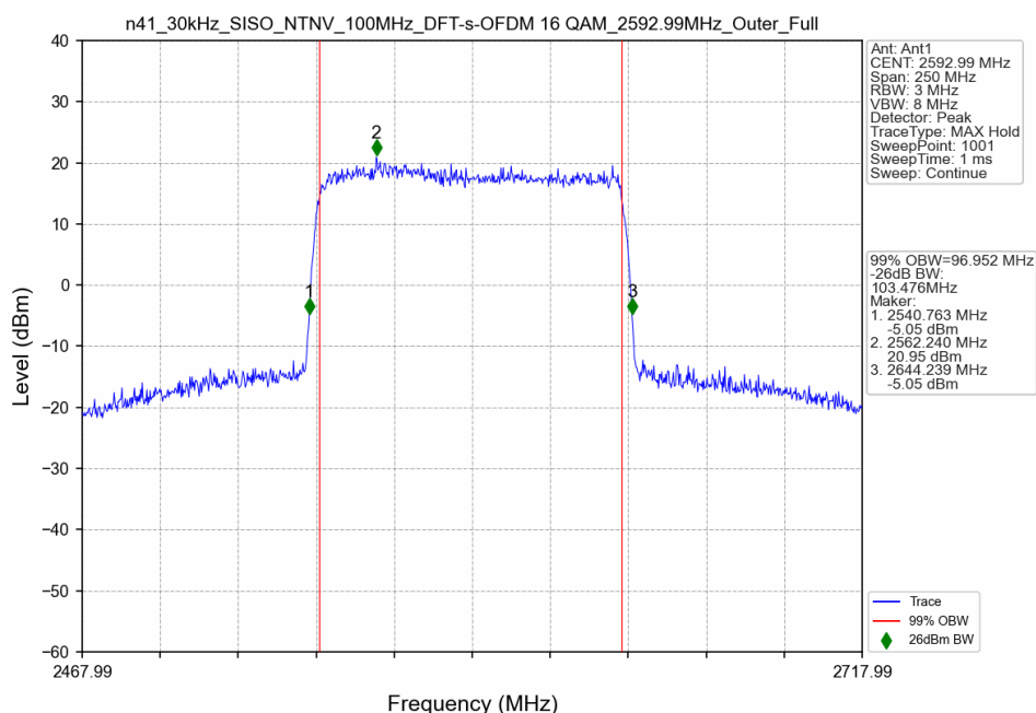
n41_30kHz_SISO_NTNV_100MHz_DFT-s-OFDM 16 QAM_2592.99MHz_Outer_Full
