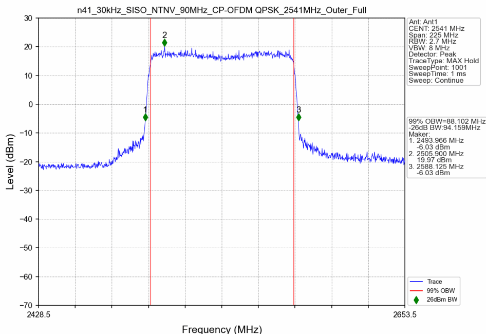
n41_30kHz_SISO_NTNV_90MHz_CP-OFDM QPSK_2541MHz_Outer_Full
