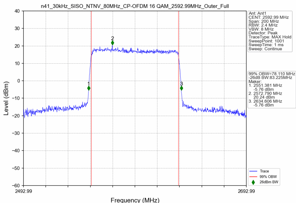
n41_30kHz_SISO_NTNV_80MHz_CP-OFDM 16 QAM_2592.99MHz_Outer_Full
