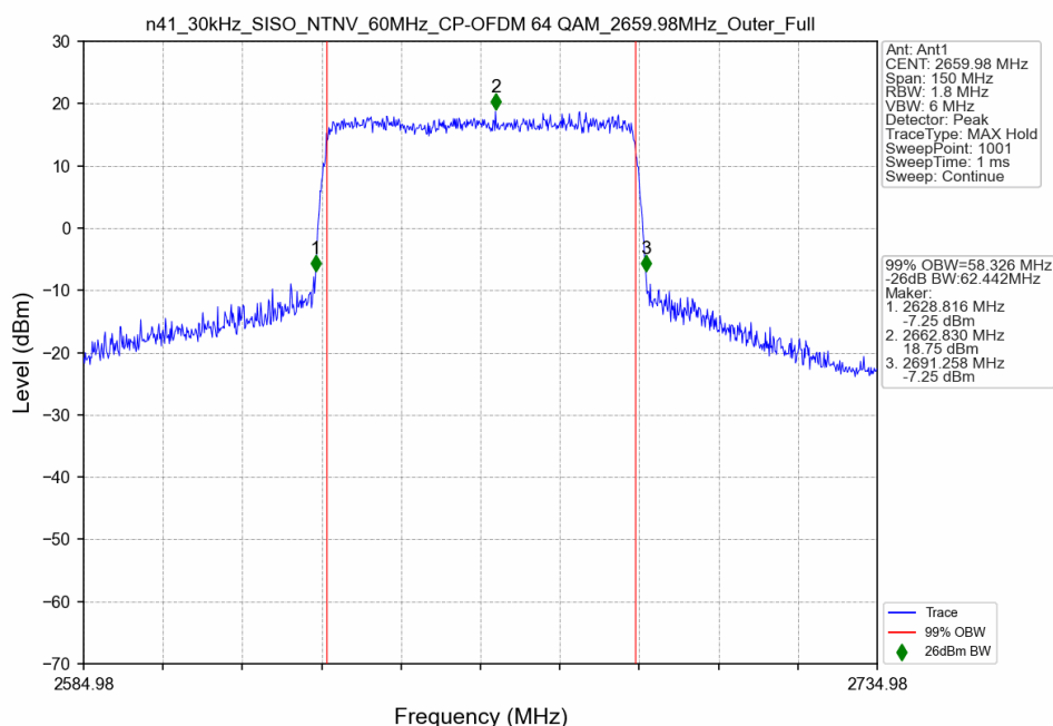
n41_30kHz_SISO_NTNV_60MHz_CP-OFDM 64 QAM_2659.98MHz_Outer_Full
