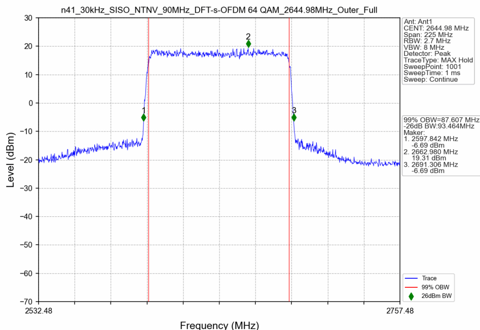
n41_30kHz_SISO_NTNV_90MHz_DFT-s-OFDM 64 QAM_2644.98MHz_Outer_Full
