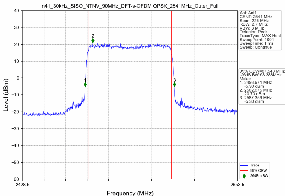
n41_30kHz_SISO_NTNV_90MHz_DFT-s-OFDM QPSK_2541MHz_Outer_Full
