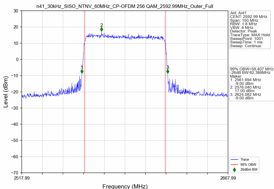
n41_30kHz_SISO_NTNV_60MHz_CP-OFDM 256 QAM_2592.99MHz_Outer_Full
