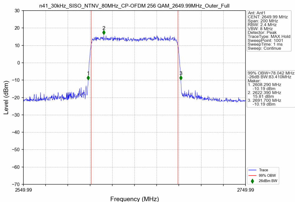
n41_30kHz_SISO_NTNV_80MHz_CP-OFDM 256 QAM_2649.99MHz_Outer_Full
