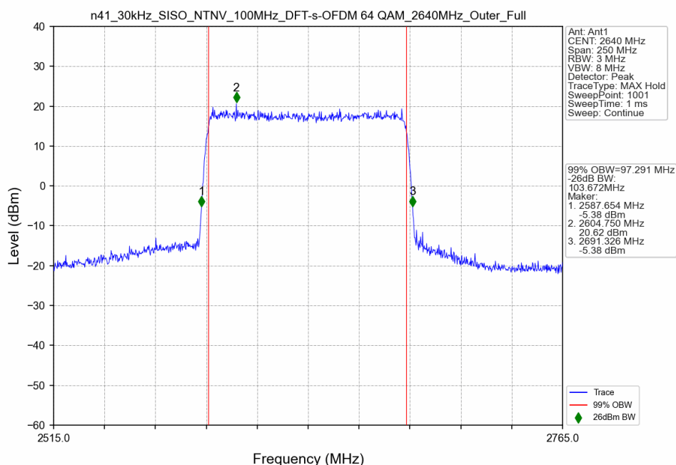
n41_30kHz_SISO_NTNV_100MHz_DFT-s-OFDM 64 QAM_2640MHz_Outer_Full
