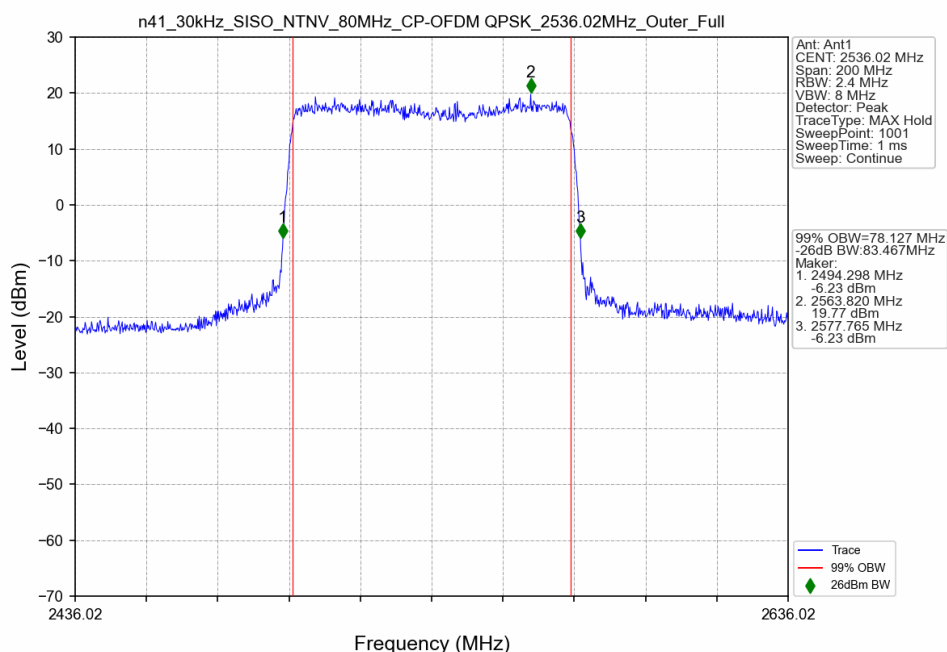
n41_30kHz_SISO_NTNV_80MHz_CP-OFDM QPSK_2536.02MHz_Outer_Full
