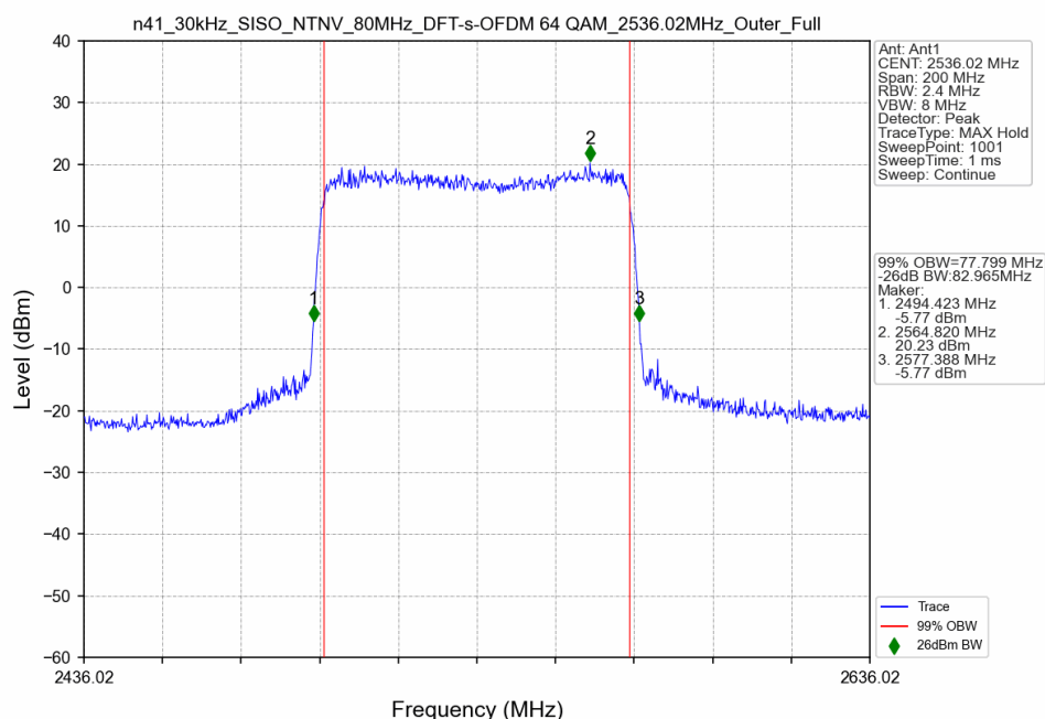
n41_30kHz_SISO_NTNV_80MHz_DFT-s-OFDM 64 QAM_2536.02MHz_Outer_Full
