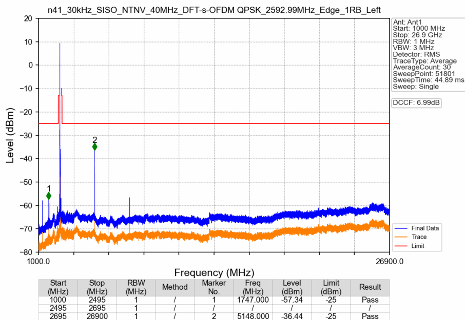
n41_30kHz_SISO_NTNV_40MHz_DFT-s-OFDM QPSK_2592.99MHz_Edge_1RB_Left
