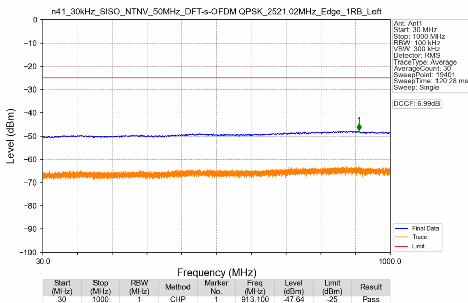
n41_30kHz_SISO_NTNV_50MHz_DFT-s-OFDM QPSK_2521.02MHz_Edge_1RB_Left
