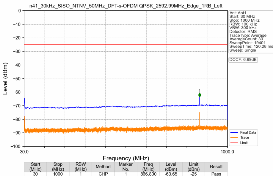
n41_30kHz_SISO_NTNV_50MHz_DFT-s-OFDM QPSK_2592.99MHz_Edge_1RB_Left
