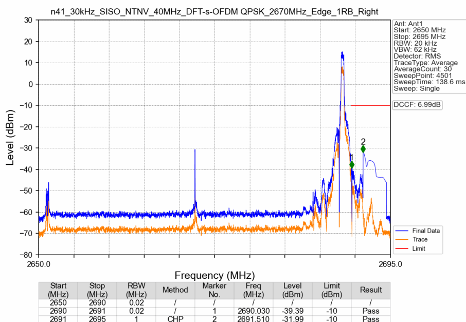
n41_30kHz_SISO_NTNV_40MHz_DFT-s-OFDM QPSK_2670MHz_Edge_1RB_Right
