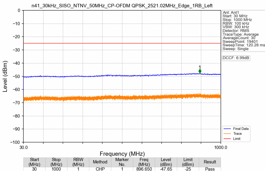
n41_30kHz_SISO_NTNV_50MHz_CP-OFDM QPSK_2521.02MHz_Edge_1RB_Left
