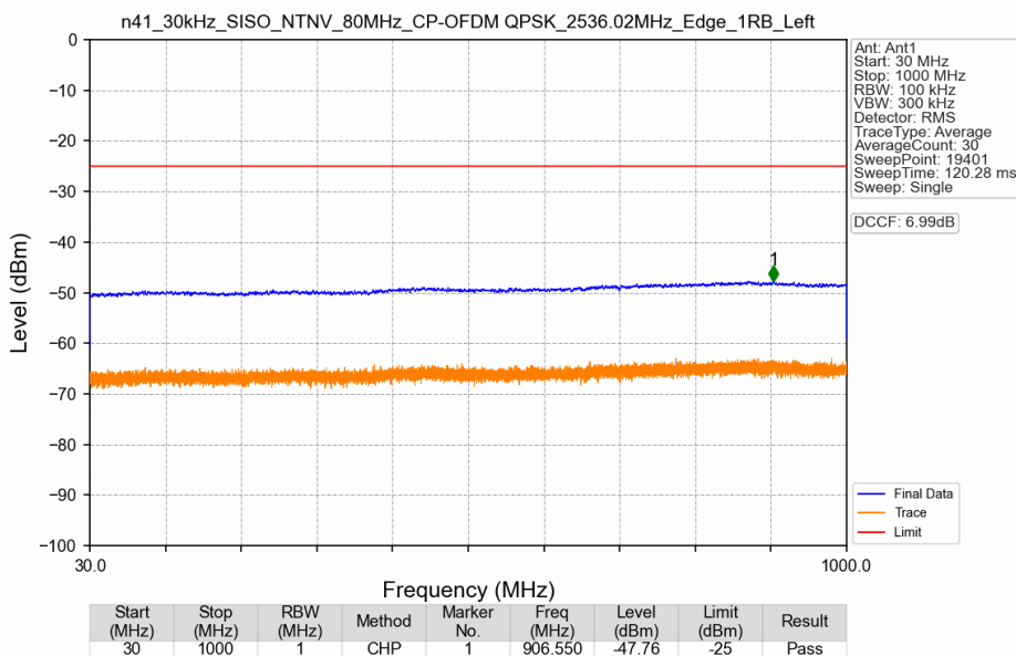
n41_30kHz_SISO_NTNV_80MHz_CP-OFDM QPSK_2536.02MHz_Edge_1RB_Left
