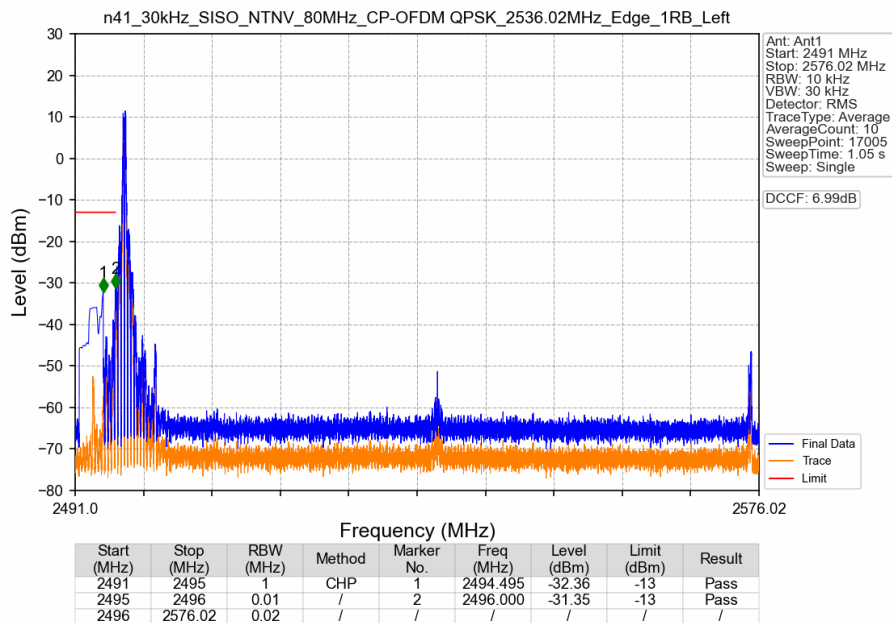
n41_30kHz_SISO_NTNV_80MHz_CP-OFDM QPSK_2536.02MHz_Edge_1RB_Left
