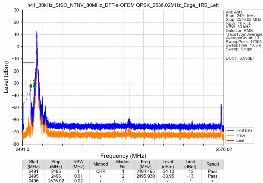
n41_30kHz_SISO_NTNV_80MHz_DFT-s-OFDM QPSK_2536.02MHz_Edge_1RB_Left
