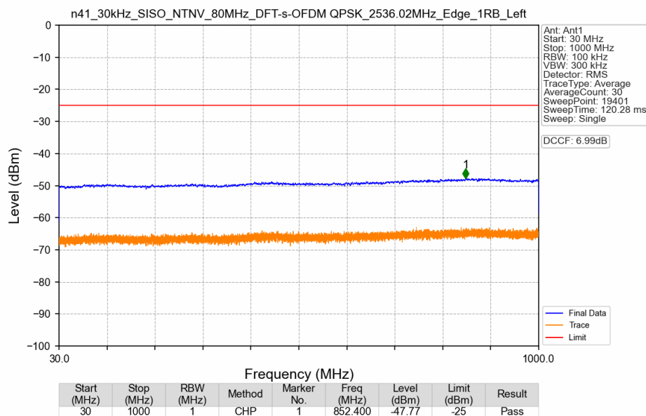
n41_30kHz_SISO_NTNV_80MHz_DFT-s-OFDM QPSK_2536.02MHz_Edge_1RB_Left
