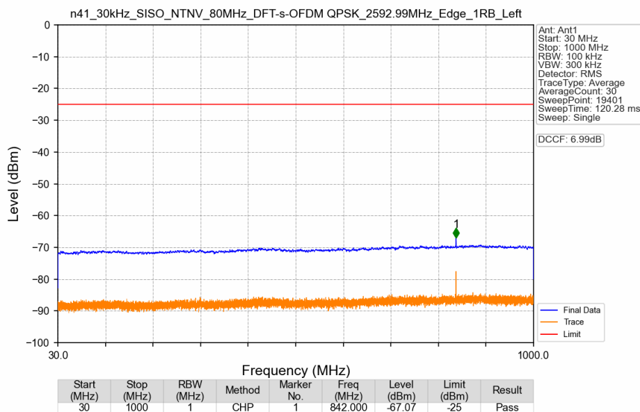
n41_30kHz_SISO_NTNV_80MHz_DFT-s-OFDM QPSK_2592.99MHz_Edge_1RB_Left
